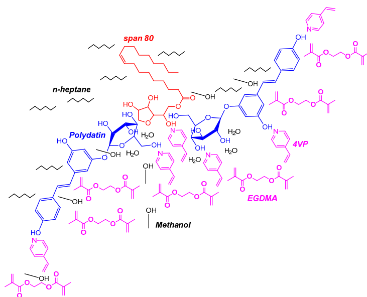
Figure 8. Depiction of a plausible surface-molecular imprinting process taking place when polydatin is used as template in a suspension polymerization with n -heptane in the oil phase, Span 80 as surfactant, 4VP as FM, EGDMA as crosslinker and MeOH/H 2 O as solvent in the monomer phase.
