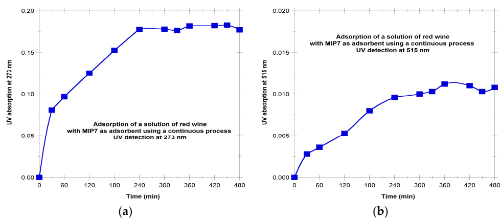
Figure 12. Dynamics of sorption of a solution of red wine in MIP7 considering a continuous process performed with a flow rate Q = 0.35 \text{ mL/min} and \text{H}_2\text{O}/\text{ACN} 70/30 ( v/v ) as solvent. Red wine was directly diluted in \text{H}_2\text{O}/\text{ACN} at 6% ( v/v ). (a) Global UV absorption of the solution at column outlet measured at 273 nm; (b) Similar measurement at 515 nm.
