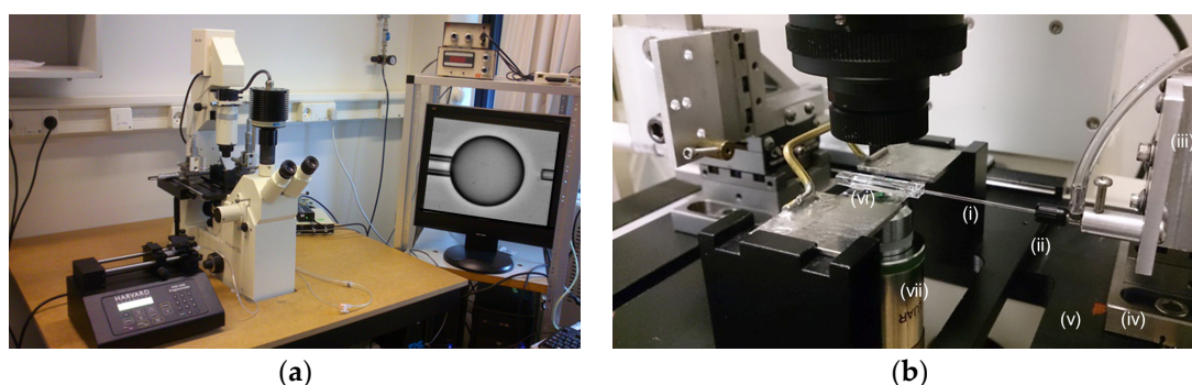
Figure 2. The micropipette manipulation station. (a) The setup consists of an inverted microscope to place and visualize the micropipette tip, operated by micromanipulators, connected to a pressurization system ( \mu\text{atm} to \text{matm} ); the samples are placed in a custom-made microchamber and all the experiments are recorded in real time by using a side-port camera for subsequent analysis. (b) The micropipette (i) is mounted via a chuck (ii) in a custom-built holder controlled by micromanipulators (iii), mounted on a stage micrometer, (iv) bolted firmly to the microscope platform (v). The image of the pipette tip in the microchamber (vi) is viewed via a 40\times objective lens (vii).
