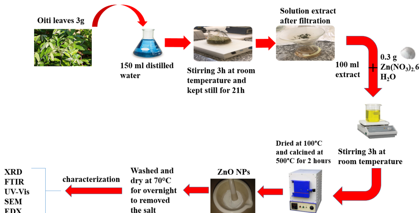
Figure 1. Schematic representation of the green ZnO NPs synthesis using Licania tomentosa leaf extract.
