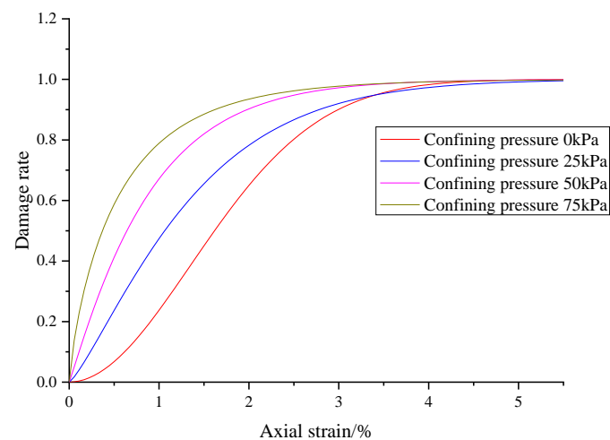
Figure 15. The development law of damage rate \lambda with strain.
