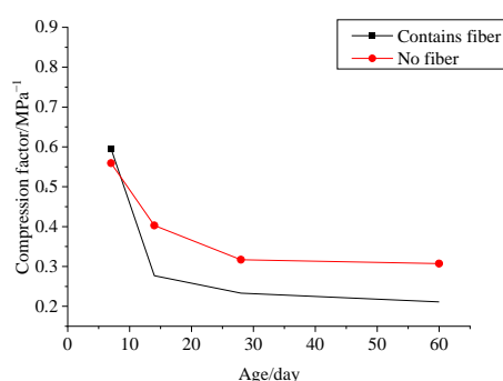
Figure 2. Compression coefficient changes with age.
