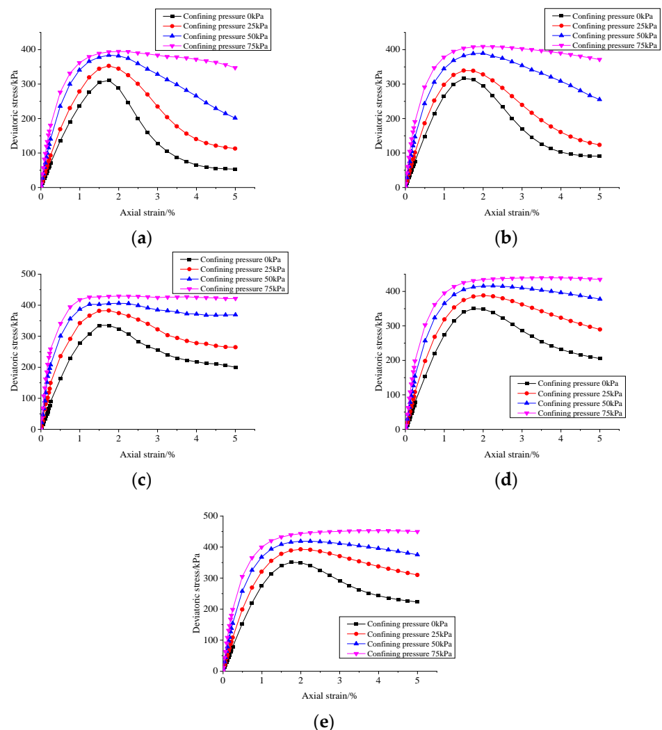
Figure 4. Stress–strain curves with different fiber contents. (a) Fiber content is 0.1%; (b) fiber content is 0.15%; (c) fiber content is 0.2%; (d) fiber content is 0.25%; (e) fiber content is 0.3%.
