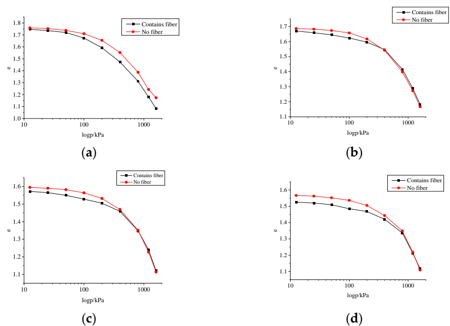
Figure 1. Plotted e-logp curve of fiber-solidified soil. (a) Maintenance time: 7 days; (b) maintenance time: 14 days; (c) maintenance time: 28 days; (d) maintenance time: 60 days.
