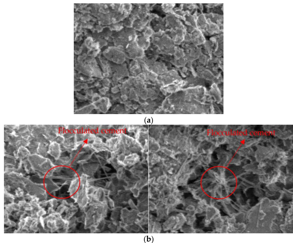
Figure 18. Microscopic morphology of curing agent product. (a) Lime hydration products; (b) lime hydration products.
