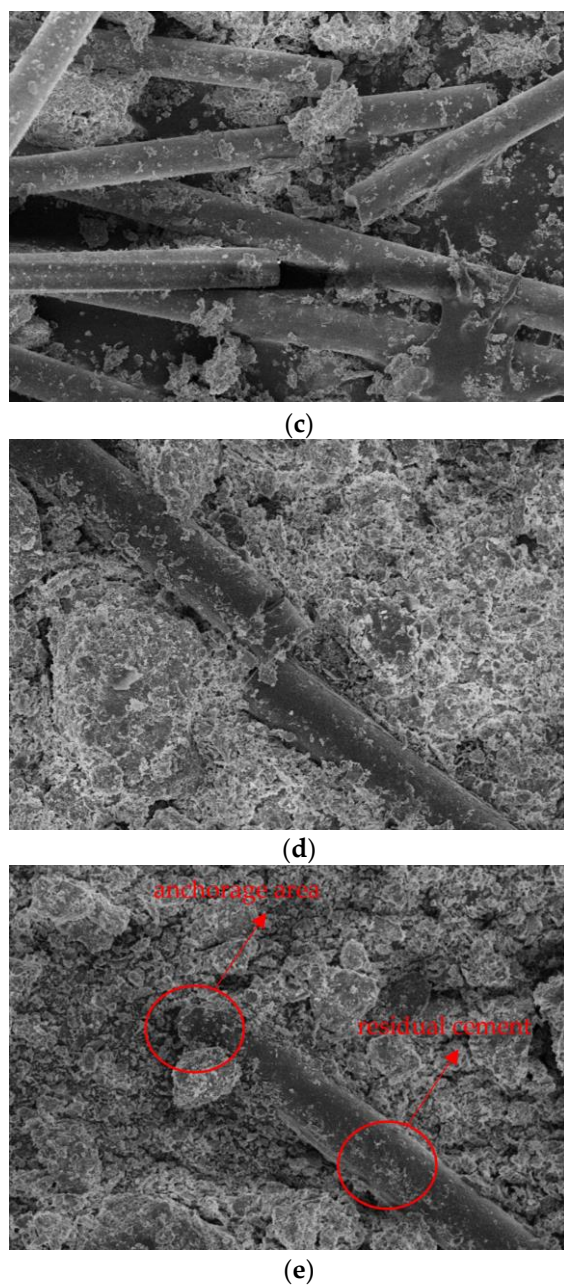
Figure 19. SEM photo of fiber. (a) Fiber bundle (300 times); (b) fiber interweaving (300 times); (c) fiber interweaving (500 times); (d) single fiber (1000 times); (e) fiber anchoring (1000 times).
