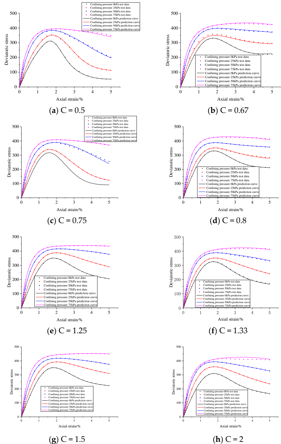
Figure 13. Comparison of test results and model prediction curve.
