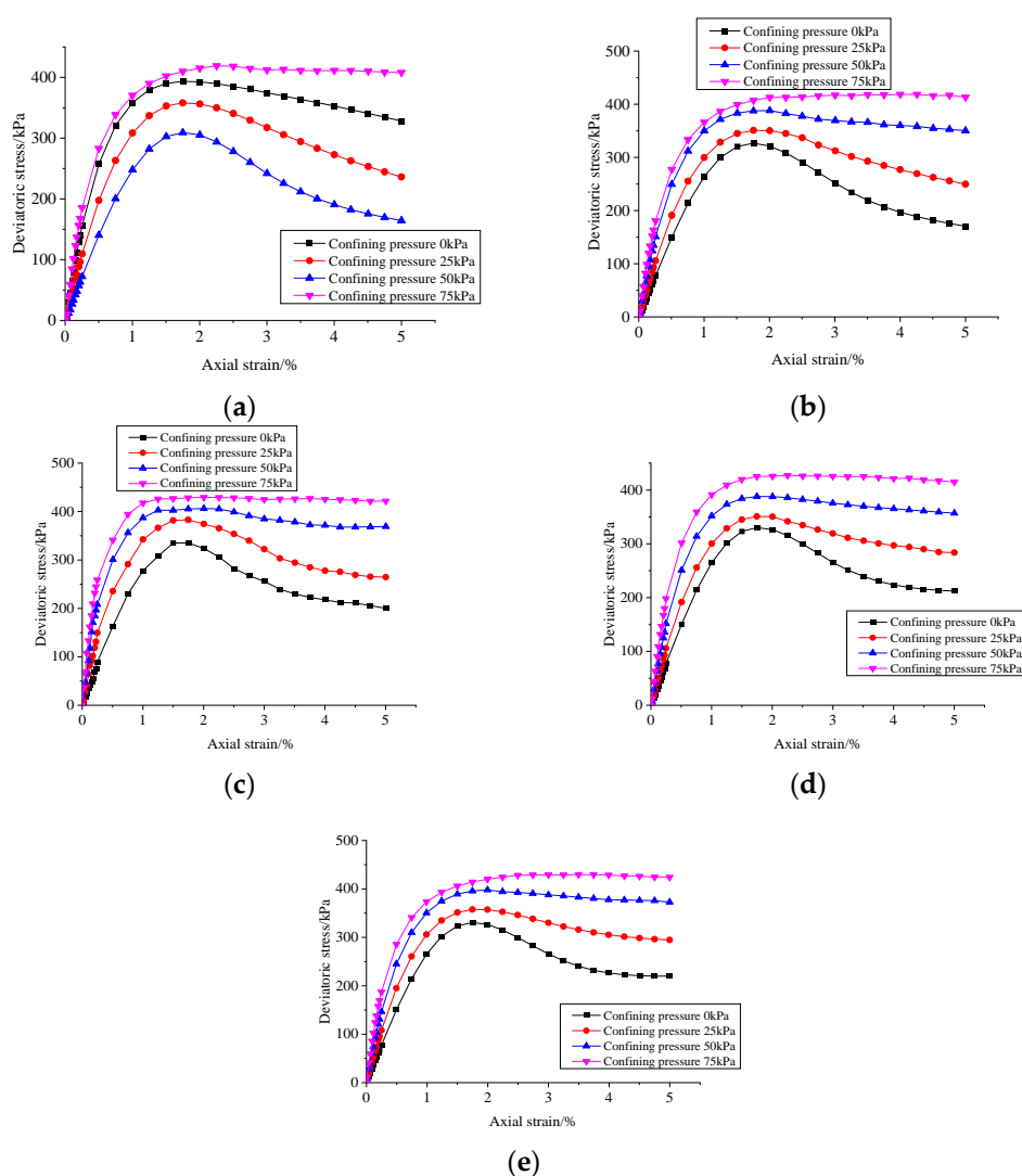
Figure 5. Stress–strain curves of different fiber lengths. (a) Fiber length is 10 mm; (b) fiber length is 15 mm; (c) fiber length is 20 mm; (d) fiber length is 25 mm; (e) fiber length is 30 mm.
