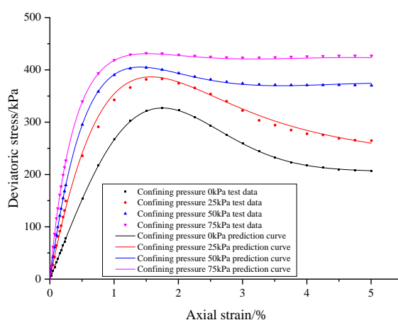
Figure 10. Comparison of test results and revised model prediction curve results.
