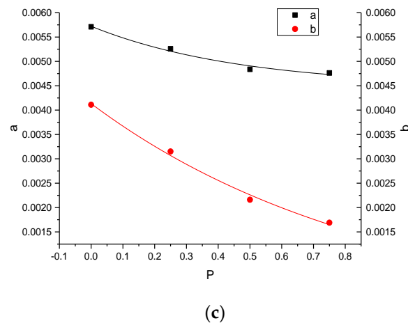
Figure 14. Fitting curve of binary-medium model as P changes. (a) Changes in nonlinear material coefficients \alpha and n with P ; (b) changes in initial elastic modulus E_b and local deformation coefficient c with P ; and (c) changes in material parameters a and b with P .
