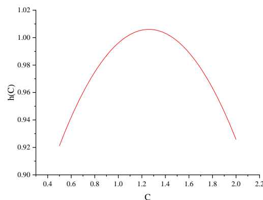
Figure 11. Cement element correction function.
