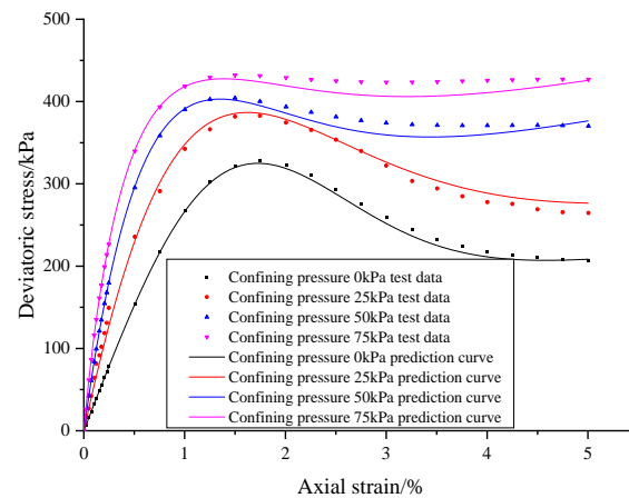
Figure 7. Comparison of test results and model prediction curve results.
