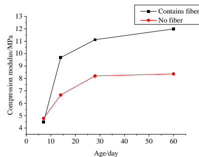
Figure 3. Compression modulus change curve with age.
