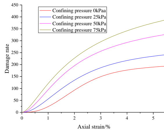
Figure 8. Friction element stress versus strain curve.
