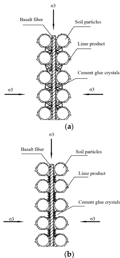
Figure 20. Schematic diagram of reinforced friction principle in triaxial shear test. (a) Before peak stress; (b) after peak stress.
