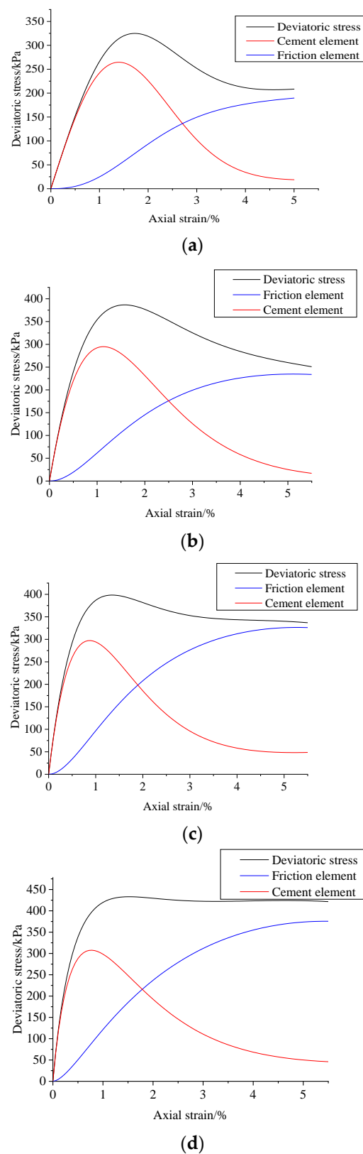
Figure 16. Stress borne by cementing elements and friction elements inside the soil under different confining pressures. (a) Confining pressure 0 kPa; (b) confining pressure 25 kPa; (c) confining pressure 50 kPa; (d) confining pressure 75 kPa.
