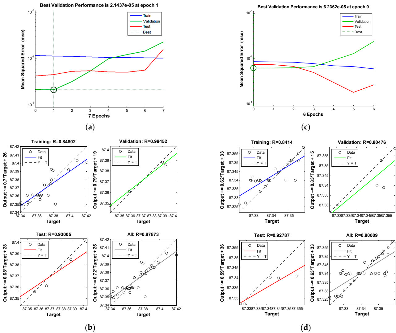
Figure 4. Visual representation of ANN performance; (a): mean square error (MSE) of pasteurized milk; (b): correlation coefficients (R) of pasteurized milk; (c): MSE of raw milk; (d): R of raw milk. The target is the experimental MC, and the output is the predicted MC.
