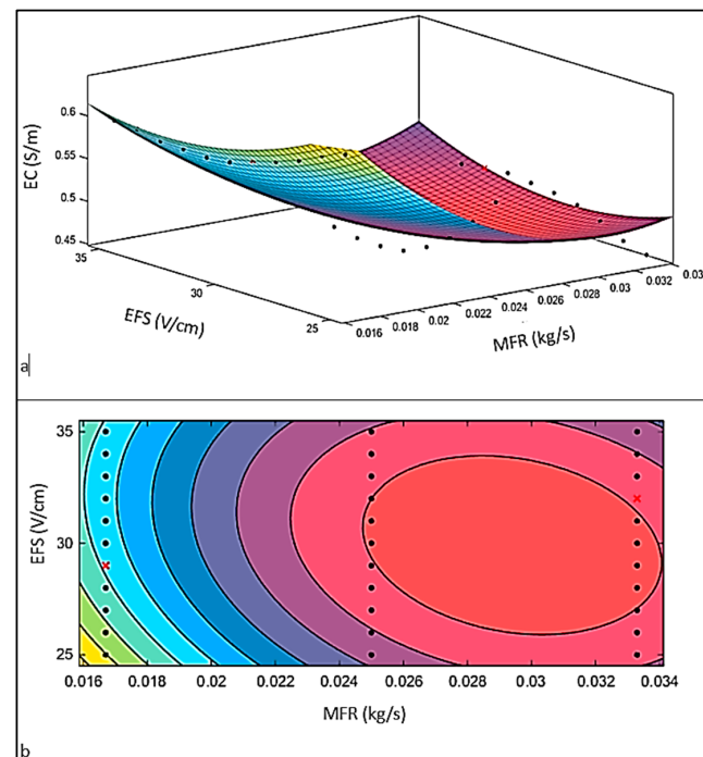
Figure 3. The effect of EFS and MFR on EC predicted by ANNs: (a) 3D plot, (b) contour plot.
