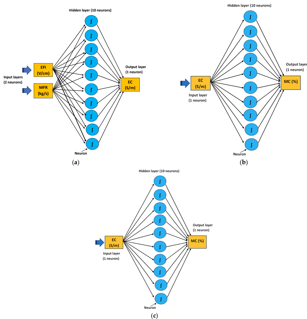
Figure 1. The feedforward neural network with multilayers: (a) prediction of electrical conductivity, (b) prediction of moisture content of pasteurized milk, (c) prediction of moisture content of raw milk. EFI: electric field intensity (straight), MFR: mass flow rate, EC: electric conductivity.
