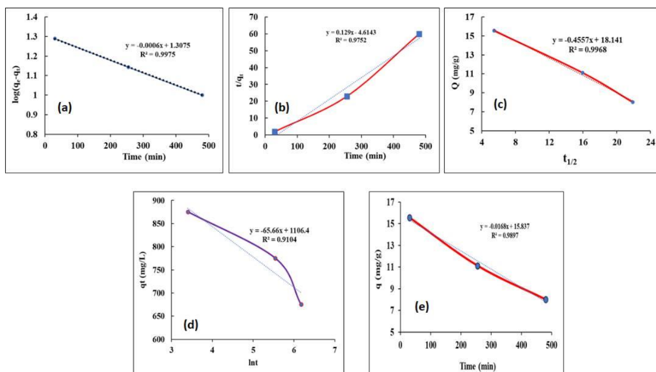
Figure 7. Adsorption kinetics fitted with (a) Pseudo-First-Order, (b) Pseudo-Second-Order (c) Intraparticle Diffusion Kinetics Models, and (d) Elovich Kinetic Model (e) Effect of adsorption time on the boron adsorption.
