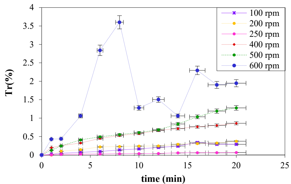
Figure 8. Effect of the stirring speed on the emulsion stability (C8Span 80: 2% wt./wt., w: (100–600) rpm, int/org (v/v): (3/4), emu/ext (v/v): 0.15/1, t_{\text{emuls}} = 3 min, [\text{HNO}_3]_{\text{Internal phase}}: 0.5\text{M} ).
