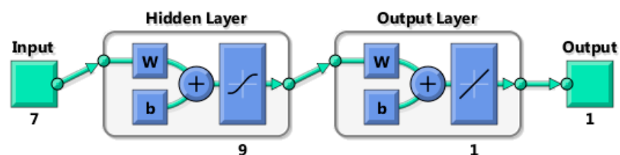
Figure 9. Schematic representation of the ANN model.
