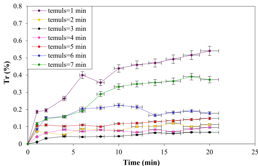
Figure 5. Effect of the emulsification time on emulsion stability (C Span 80: 2\% wt./wt., w : 250\text{ rpm} , int/org ( v/v ): 1/1 , emu/ext ( v/v ): 0.15/1 , t_{\text{emuls}} = [1-7]\text{ min} , [\text{HNO}_3]_{\text{Internal phase}} = 0.5\text{ M} ).
