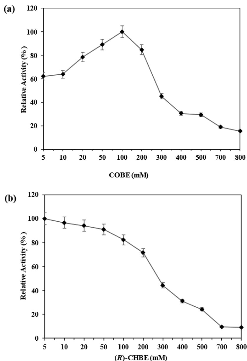
Figure 5. Effects of COBE loading (5–800 mM) on the reductase activity at 30 °C and pH 7.0 (a); effects of CHBE loading (5–800 mM) on the reductase activity at 30 °C and pH 7.0 (b).
