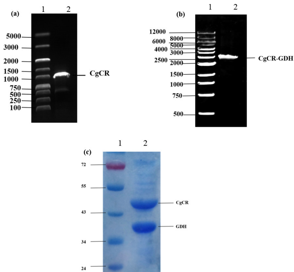
Figure 3. Analysis of the CgCR gene fragment through electrophoresis (Lane 1: marker, Lane 2: CgCR gene) (a); analysis of the CgCR-GDH gene fragment through electrophoresis (Lane 1: marker, Lane 2: CgCR-GDH gene) (b); SDS-PAGE analysis of recombinant protein of CgCR and GDH in recombinant E. coli CgCR cells expressing carbonyl reductase (CgCR) and glucose dehydrogenase (GDH) (Lane 1: marker, Lane 2: CgCR (43.9 kDa) and GDH (36.0 kDa) in E. coli CgCR) (c).
