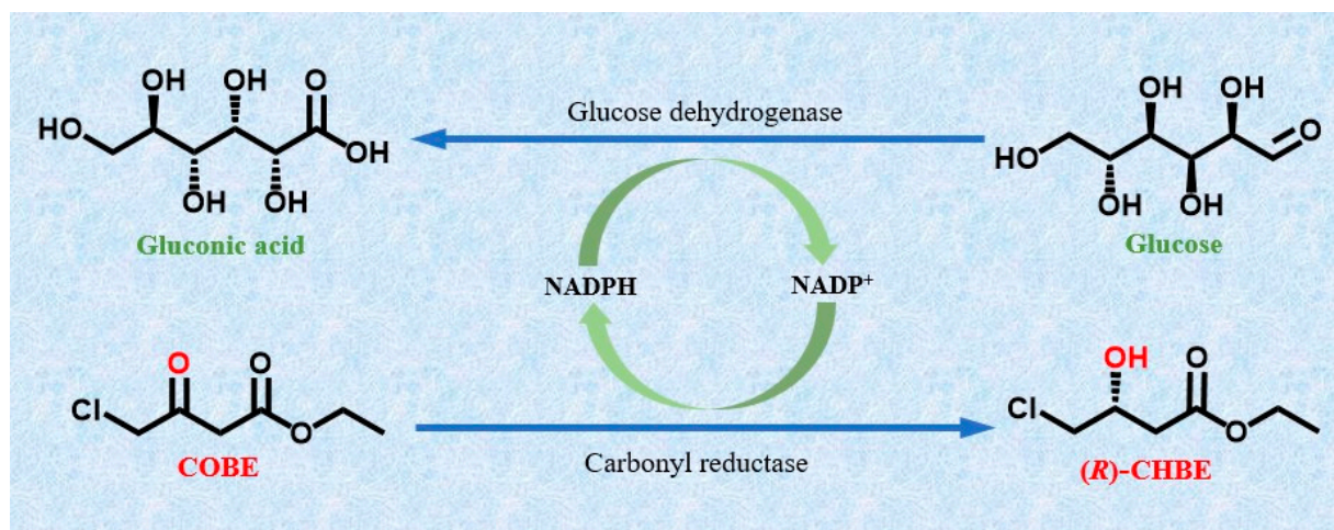
Figure 1. Glucose/GDH cofactor regeneration system.
