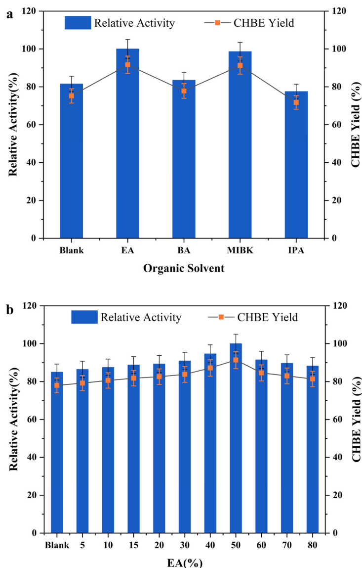
Figure 6. Effect of different organic solvents (50% of volumetric ratio) on the catalytic reaction (100 mM COBE, 30 °C, and pH 7.0) (a); effect of ethyl acetate (0–80% of volumetric ratio) on the catalytic reaction (100 mM COBE, 30 °C, and pH 7.0) (b).
