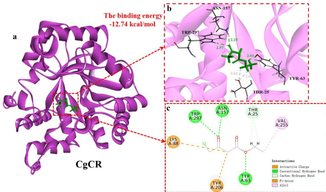
Figure 4. The binding of COBE with CgCR (a); making apparent interactions with the functionally important residues of CgCR (b); the 2D plot of CgCR binding-pocket residues and their interaction (c).
