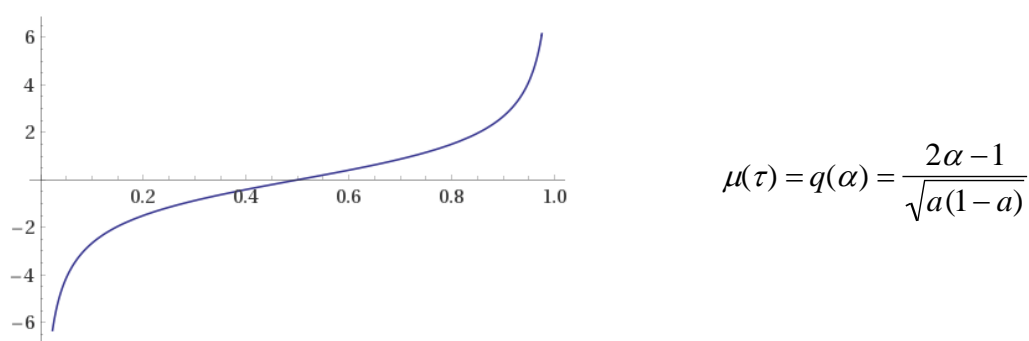
Figure 3. Identical expectile and quantile functions for the Koenker distribution.
