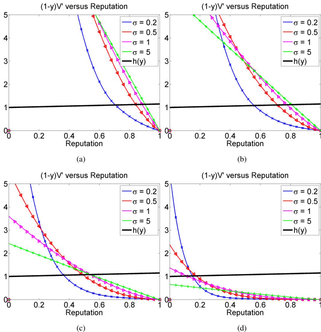
Figure 2. A plot of the quantity (1-y)V'(y) , where V(y) is a numerical solution of the reduced boundary value problem Equation (17). The value y^* is defined as the intersection of these curves with h(y) (the solid line). (a) \rho = 0.1 ; (b) \rho = 0.2 ; (c) \rho = 0.5 ; (d) \rho = 2.0 .
