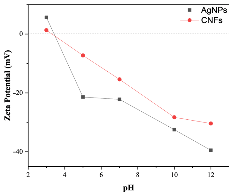
Figure 2. Zeta potential ( \zeta ) in mV of silver nanoparticles (AgNPs) and carbon nanofibers (CNFs) as a function of pH in a water solution.
