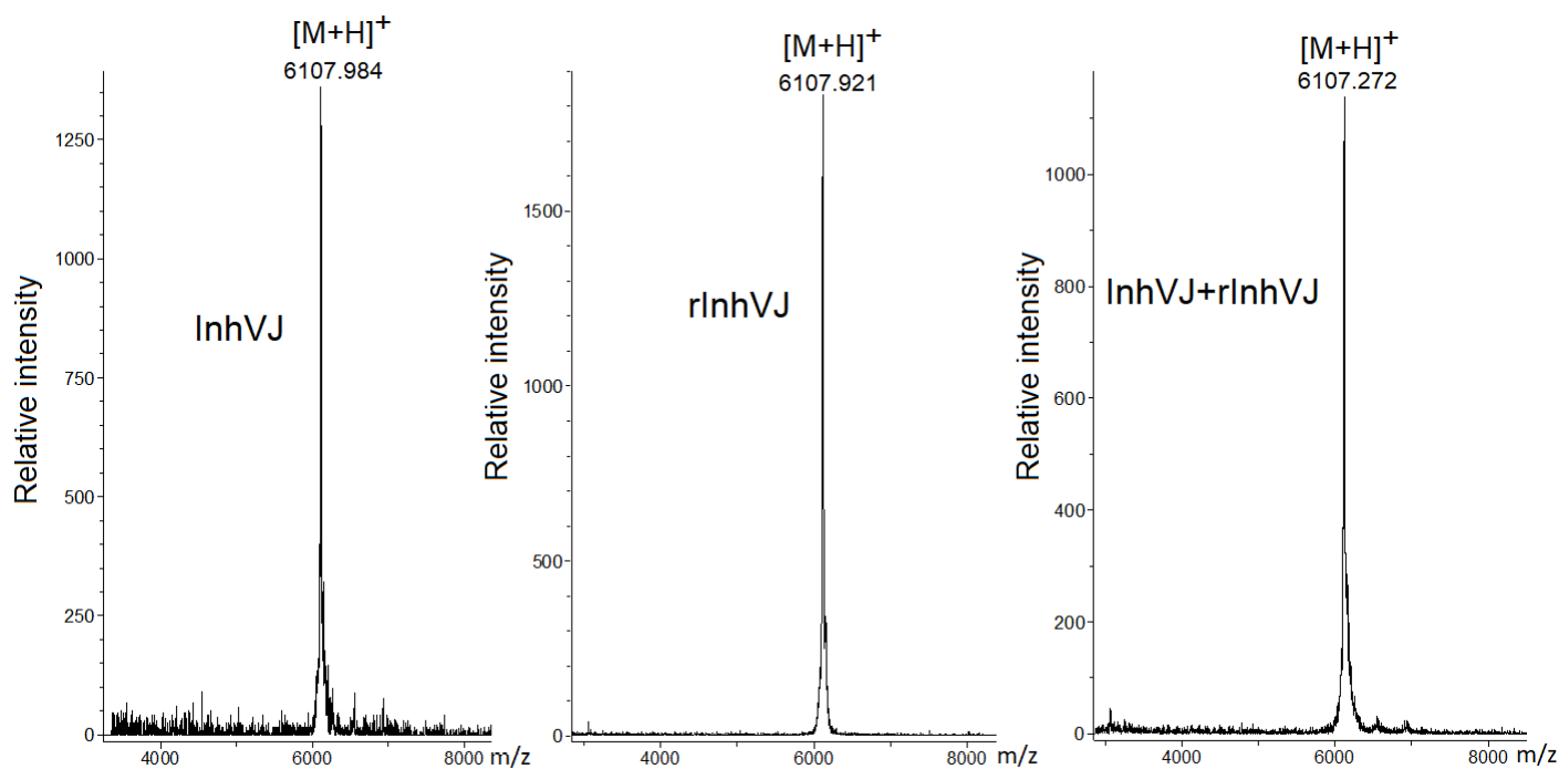
Figure S1 – (a) Elution profile of native InhVJ, recombinant InhVJ (rInhVJ) and their mix on Nucleosil C 18 column (Sigma Aldrich, USA) in a linear gradient of buffer B (0–50%) at a flow rate of 0.5 ml/min for 50 min. (b) Mass spectra of native InhVJ, recombinant InhVJ (rInhVJ) and their mix.
