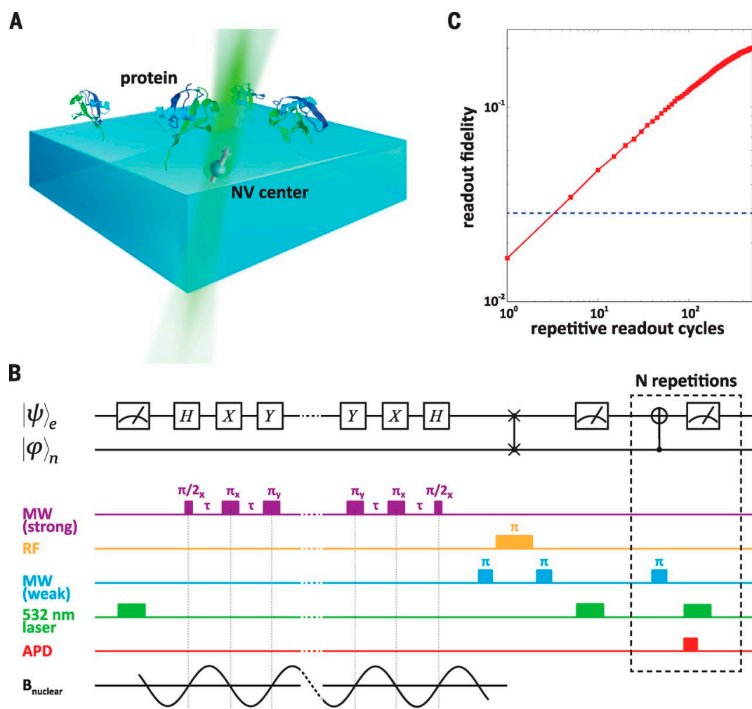
Figure 1. Experimental setup and magnetometry with repetitive readout described in [11]. Image from [11]. Reprinted with permission from AAAS. (A) Schematic of the experimental setup. Ubiquitin proteins attached to the diamond surface are probed using a proximal quantum sensor consisting of a nitrogen-vacancy (NV) center electronic spin and its associated 15 N nuclear spin; (B) Quantum circuit diagram and experimental magnetometry pulse sequence; (C) Measured gain in the readout fidelity as a function of repetitive readout cycles. MW: microwave; RF: radiofrequency; APD: avalanche photodiode; B magnetic field of the nuclear spin.
