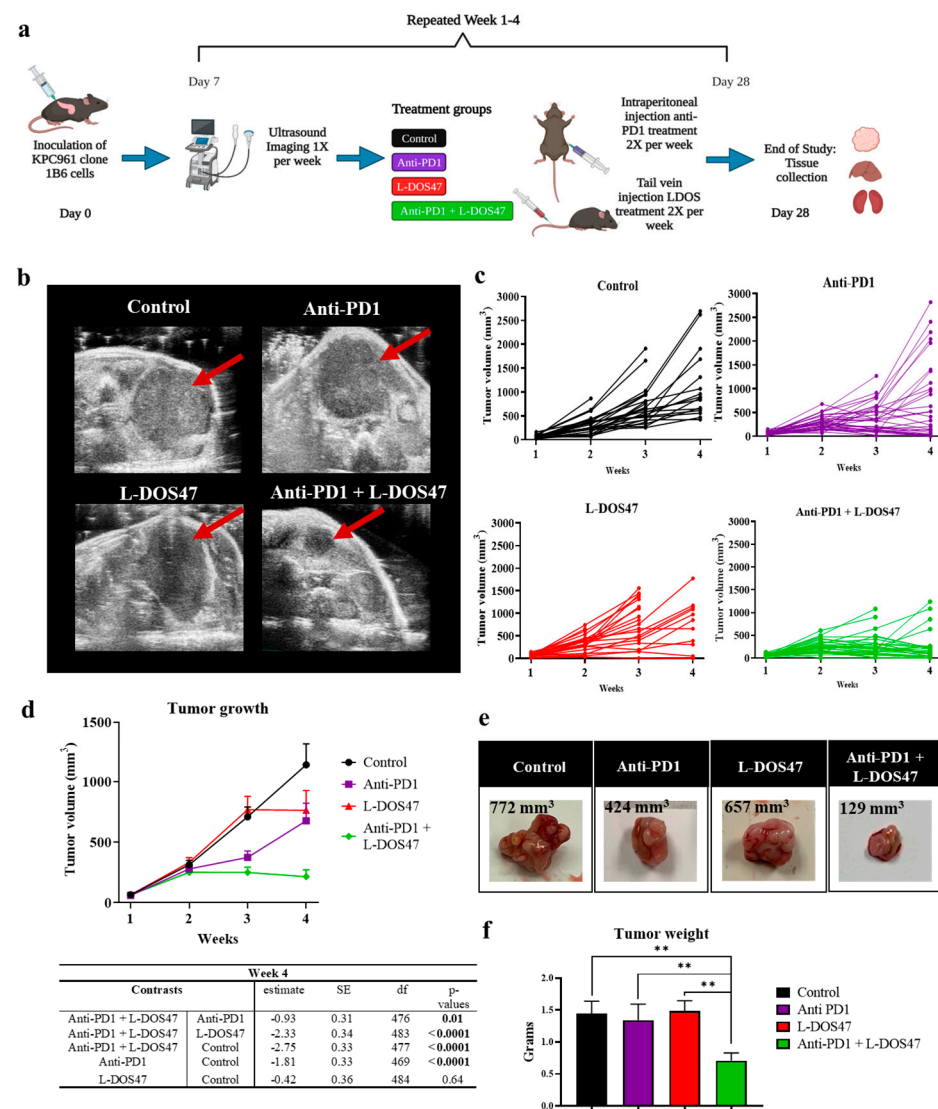
Figure 4. Therapeutic efficacy in KPC961-1B6 orthotopic tumors. (a) Experimental design. (b) Representative ultrasound images of KPC961-1B6 pancreatic tumors. (c) Individual tumor growth in each therapy group for 3 replicates ( n = 28 in the control group; n = 35 in the anti-PD1 group; n = 23 in the L-DOS47 group; and n = 35 in the anti-PD1 + L-DOS47 group). (d) Mean tumor volume \pm SEM for each therapy group with the corresponding table showing the differences at endpoint (week 4). (e) Representative ex vivo images of KPC961-1B6 tumors for each therapy group with the corresponding tumor volumes as measured by US (rounded to integral digit). (f) Mean tumor weight at endpoint. Statistical significance is reported based on the p -values obtained from the Tukey’s test ** p \leq 0.01 .
