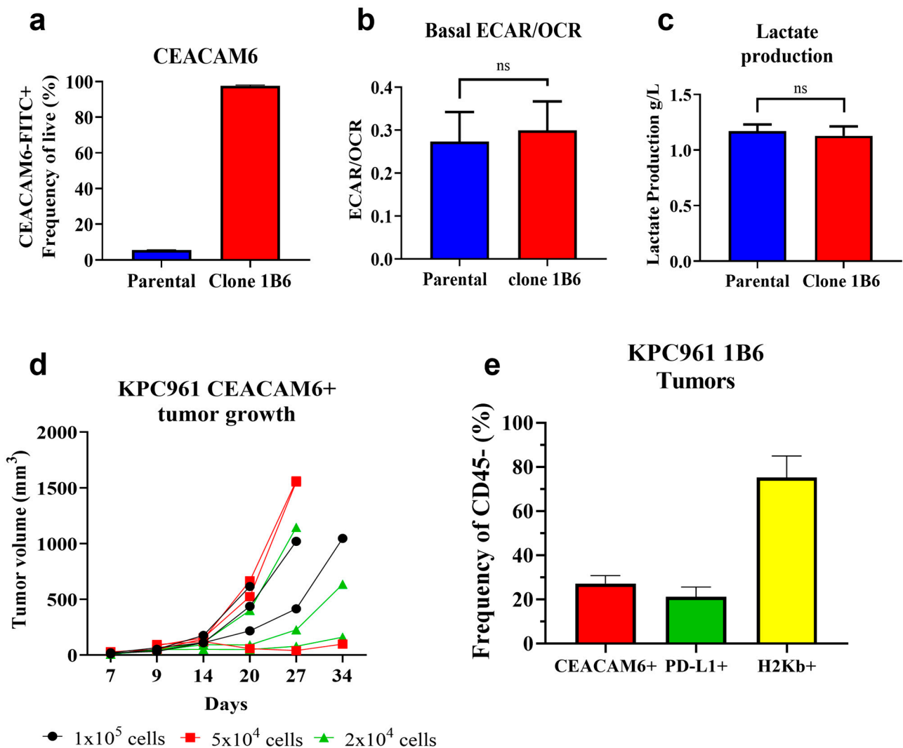
Figure 1. Generation of an orthotopic pancreatic adenocarcinoma murine tumor model expressing human CEACAM6. (a) Percentage of CEACAM6-expressing cells analyzed via flow cytometry in KPC961 parental and KPC961 clone 1B6 cells. (b) Ratio of extracellular acidification (ECAR) and oxygen consumption rate (OCR) profiles in KPC961 parental and clone 1B6 cells. (c) Lactate production in KPC961 parental and clone 1B6 cells. (d) Tumor growth as a function of inoculum size. KPC961-CEACAM6 cells were inoculated into the pancreas of B6.129 mice ( n = 3 for each inoculum size) at 100,000, 50,000, and 20,000 cells, and tumor volumes were measured via ultrasound. Ascites fluid was observed in two mice inoculated with 100,000 cells on days 24 and 29, two mice inoculated with 50,000 cells on day 29, and one mouse inoculated with 20,000 cells on day 27. (e) Expression of CEACAM6, PD-L1, and H2Kb in KPC961-1B6 cells of inoculated orthotopic tumors obtained via flow cytometry.
