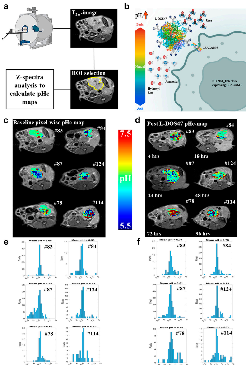
Figure 2. Pharmacodynamics of L-DOS47 in vivo as measured via MRI-CEST pH imaging. (a) Summarized scheme for image acquisitions and post-processing analyses for extracellular tumor pH (pHe) maps. A mouse was placed into the MRI scanner to start image collection, and a T_{2w} image was used as an anatomical (reference) image through which the region of interest (ROI) was drawn to selectively calculate pHe only in the tumor region of the CEST images. (b) L-DOS47 mechanism of action. Both urease and CEACAM6 protein structures were taken from the Protein Data Bank. The MRI mouse picture in (a) and the entire picture (b) were generated with BioRender.com.
