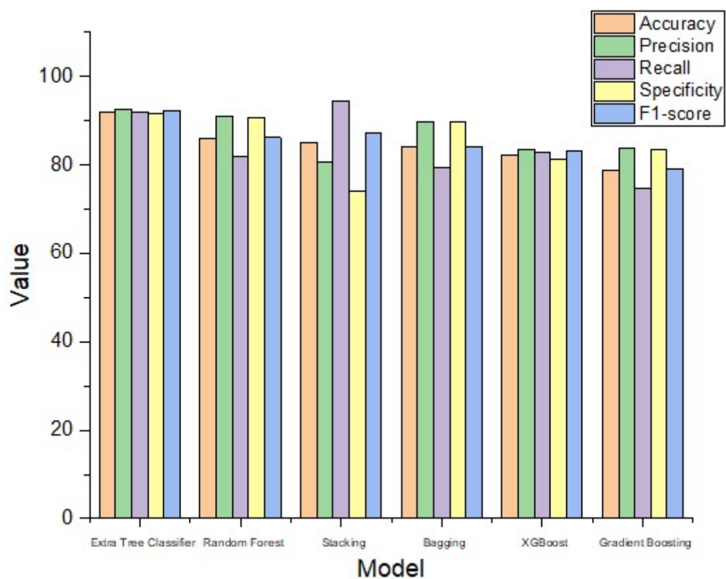
Figure 5. Metrics comparison between different models.
