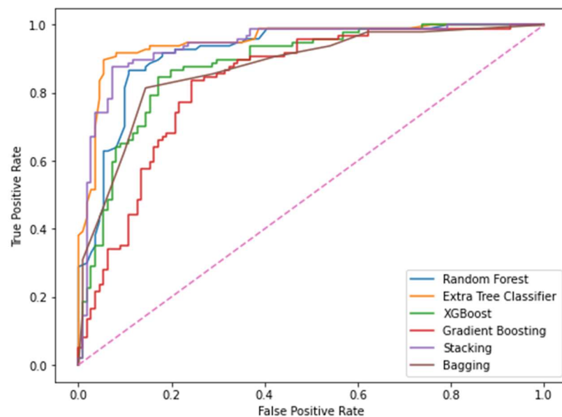
Figure 6. ROC curve of models.
