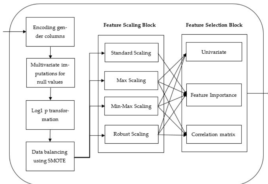
Figure 3. The proposed preprocessing block to classify liver disease.
