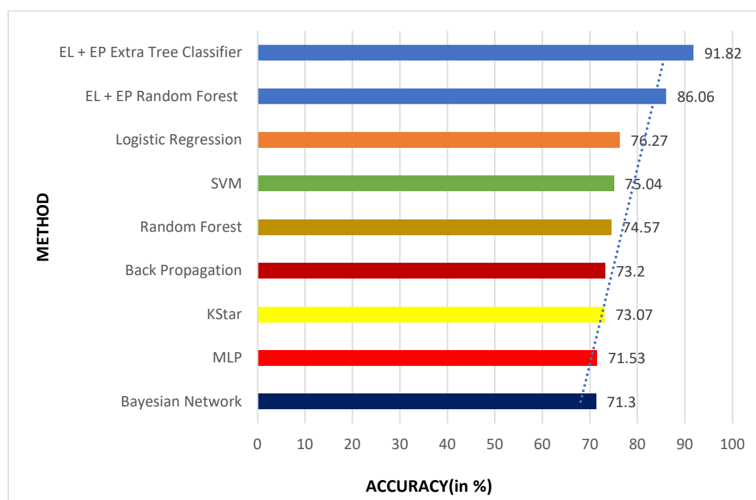
Figure 12. Comparison graph of proposed work with other existing works.
