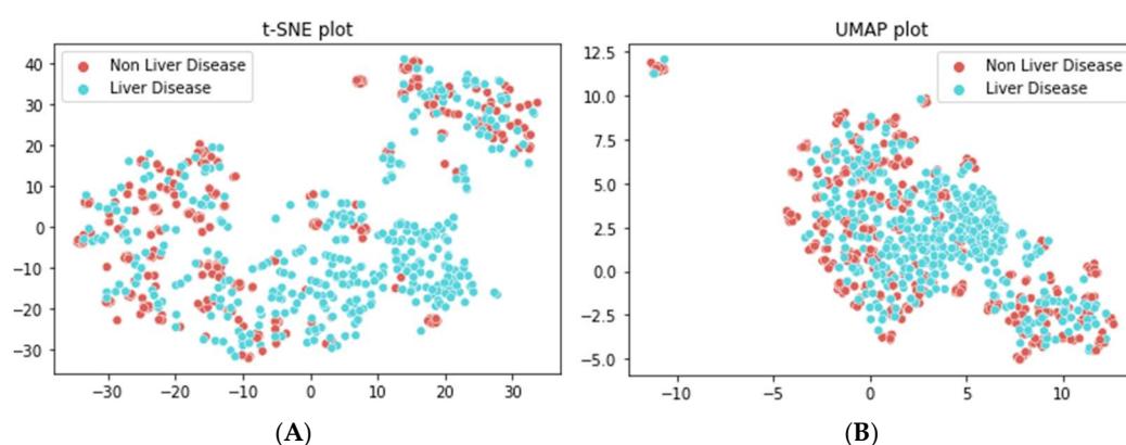
Figure 11. Feature visualization of extra tree classifier model. (A) t-SNE plot (B) UMAP plot.
