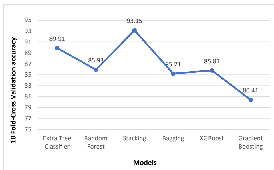
Figure 8. Comparison of 10-fold cross validation accuracy of different Models.
