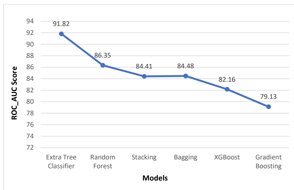
Figure 7. Metrics comparison graph of ROC_AUC.
