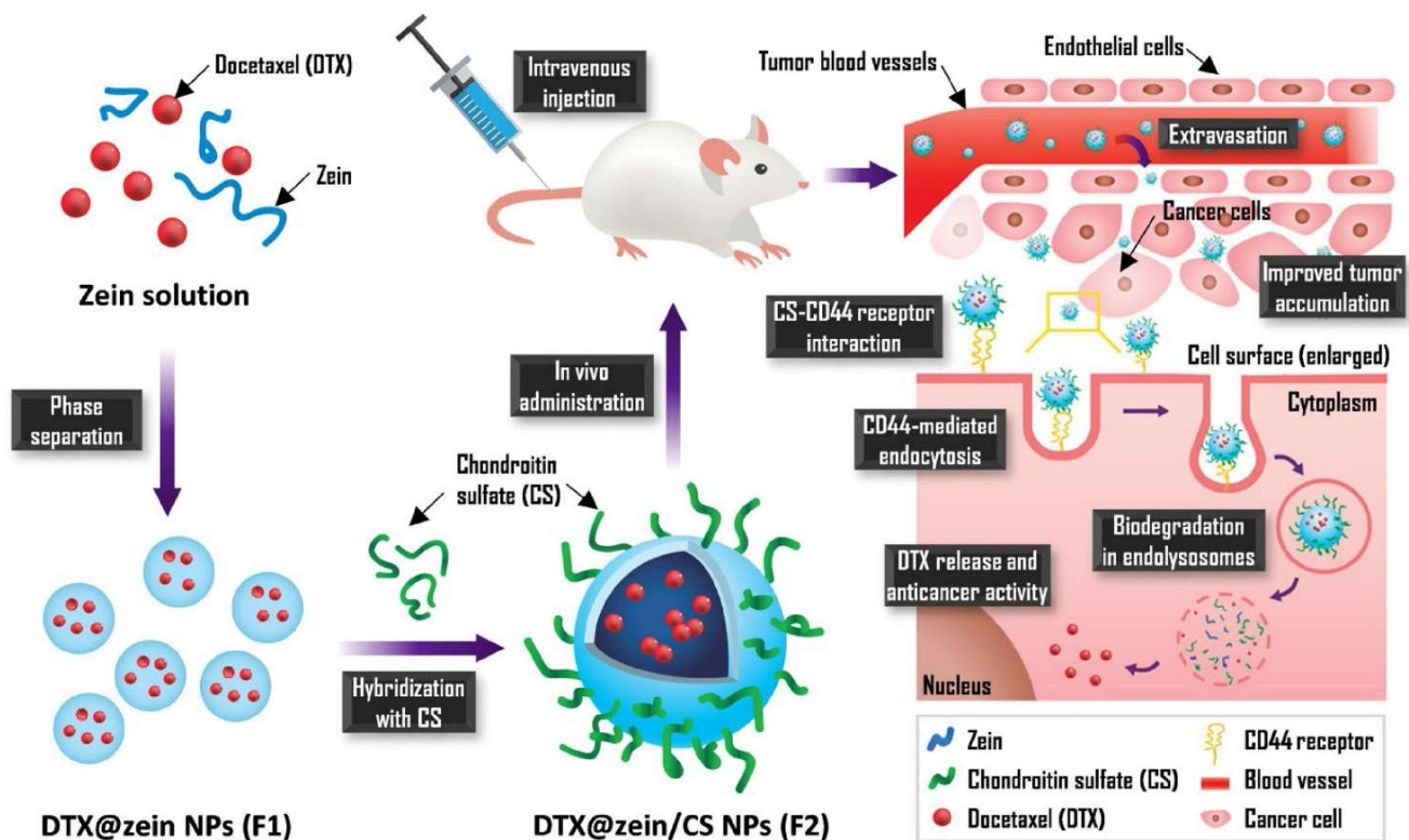
Figure 5. Scheme for the preparation Dtx-loaded CS-hybridized zein NPs and their mechanism of action. Reprinted with permission from Ref. [99]. Copyright (2021) Elsevier.
