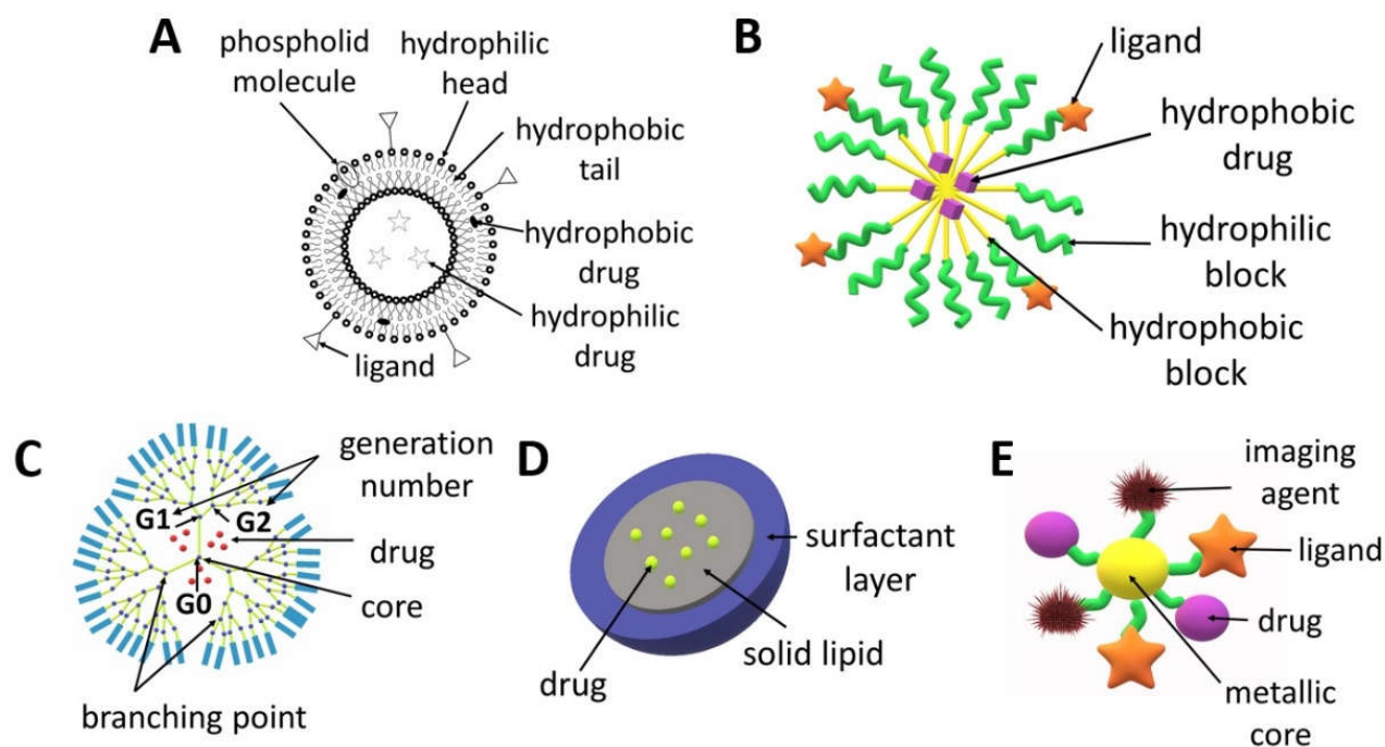
Figure 2. Scheme of the structures of drug delivery systems: (A) liposome, (B) micelle, (C) dendrimer, (D) solid lipid nanoparticle, (E) metallic nanoparticle.
