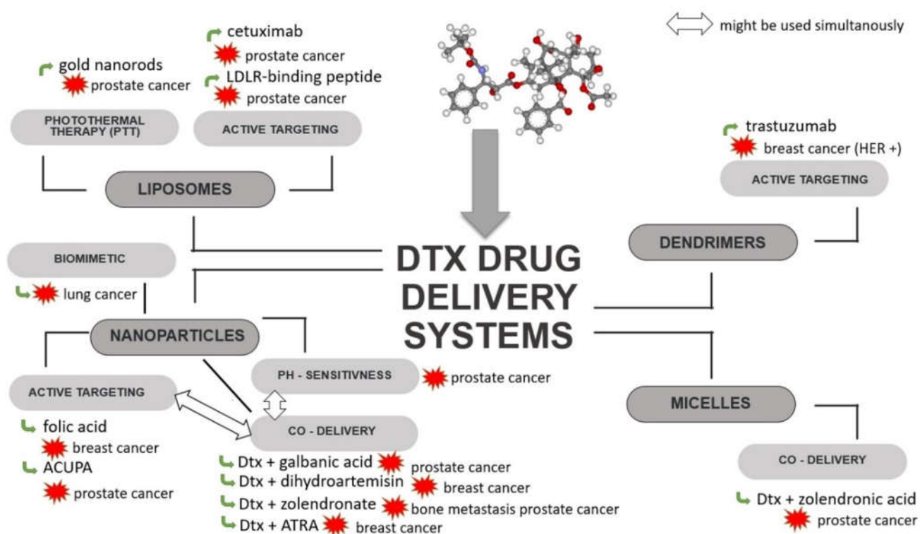
Figure 4. Scheme of strategies used for Dtx-loaded delivery systems. ACUPA—((S)-2-(3-((S)-5-amino-1-carboxypentyl) ureido) pentanedioic acid; ATRA—all-trans-retinoic acid; Dtx—docetaxel; HER—human epidermal growth factor receptor; LDLR—low-density lipoprotein receptor.
