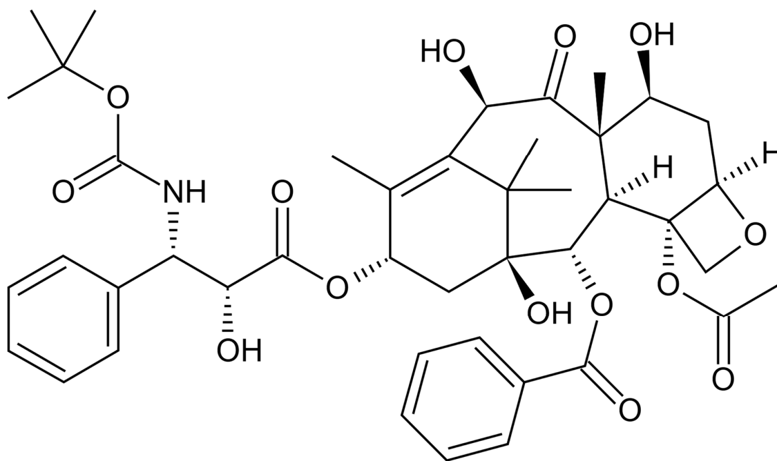
Figure 3. Chemical structure of docetaxel (Dtx).
