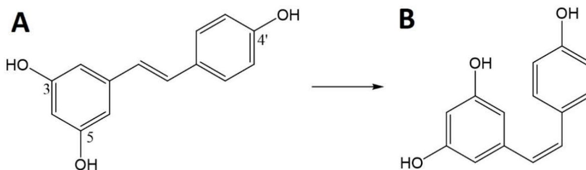
Figure 6. Chemical structure of resveratrol (Res)— trans (A) and cis (B).
