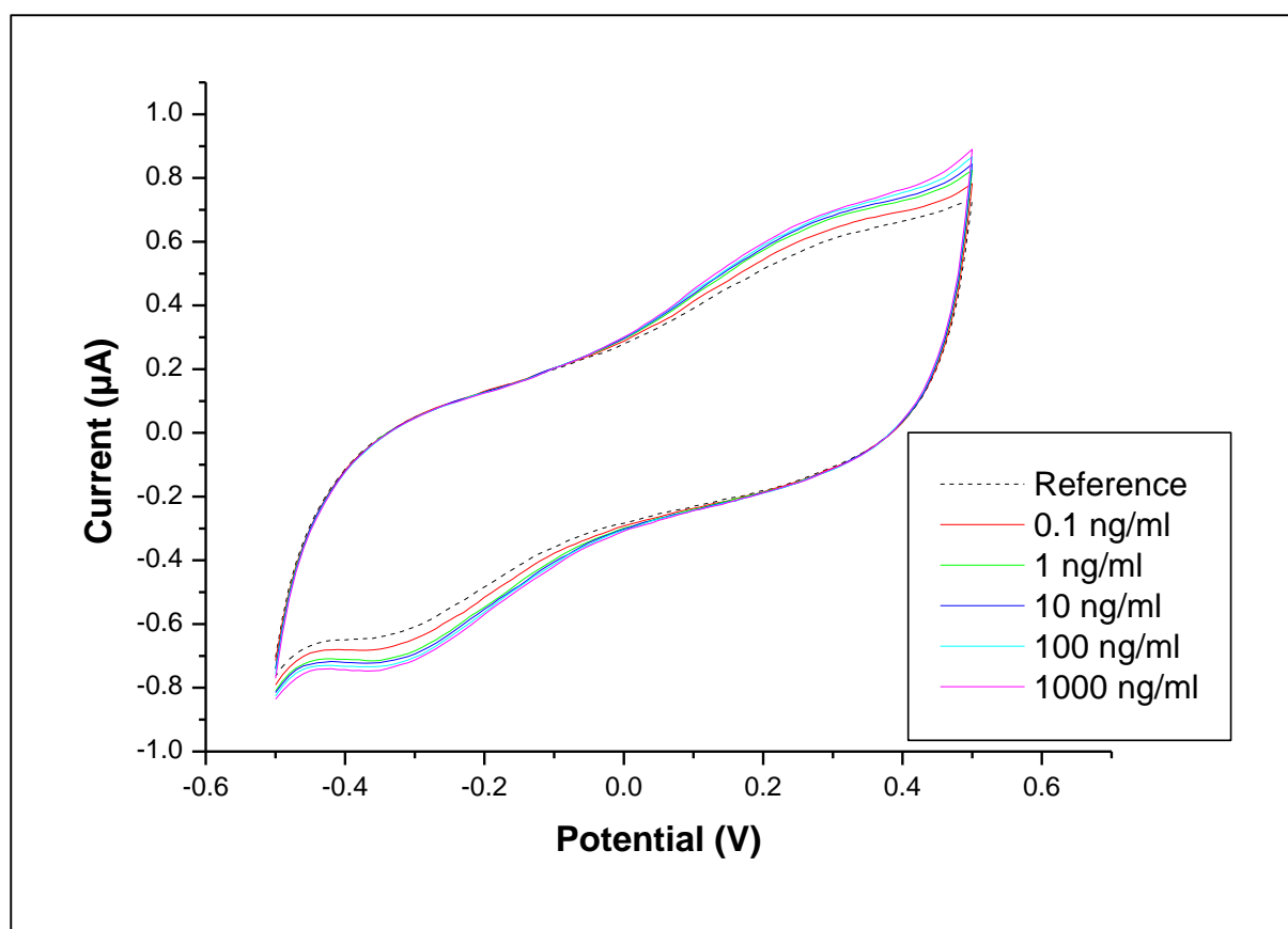
Figure S1. The series of CVs of samples with immobilized aptamers stored in the fridge for two to three week.
