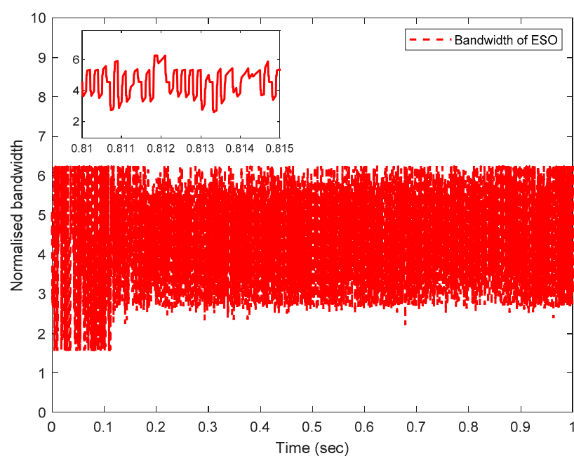
Figure 6. Time histories of the observer's bandwidth control \varpi_0 .
