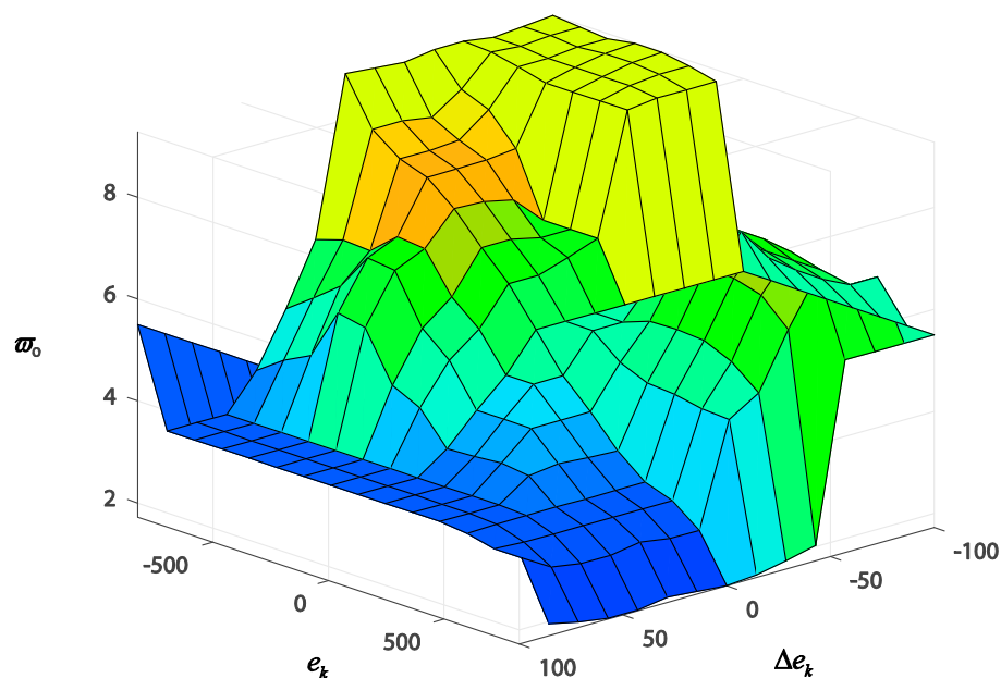
Figure 5. Fuzzy surface of the observer's bandwidth parameter \varpi_0 .
