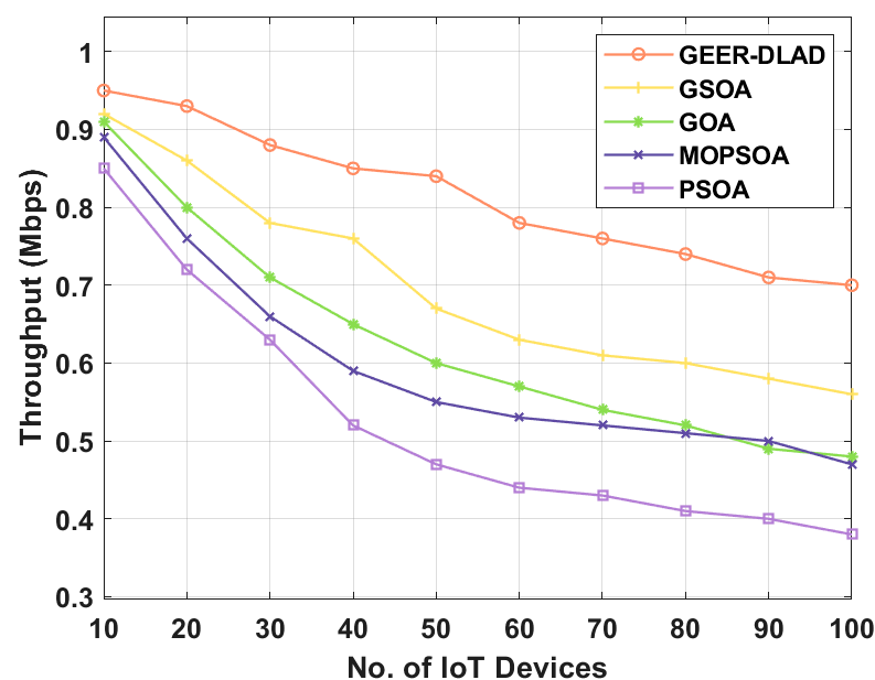
Figure 7. Throughput analysis of GEER-DLAD model.
