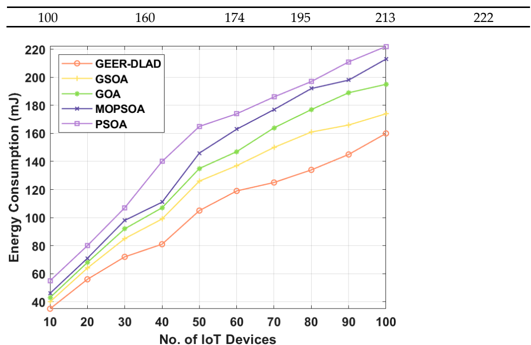
Figure 5. The Energy consumption analysis of GEER-DLAD model.
