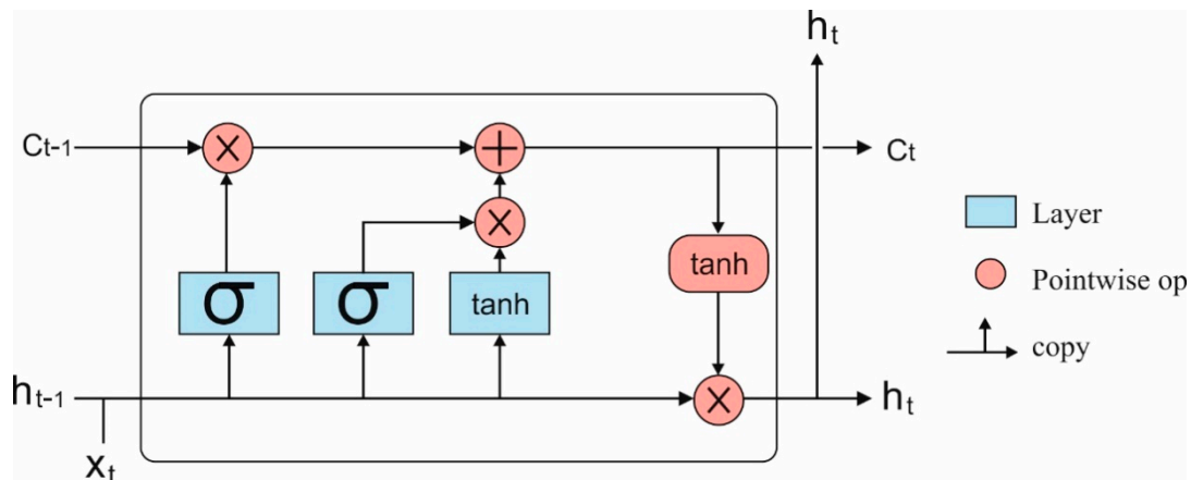
Figure 4. The Structure of LSTM.
