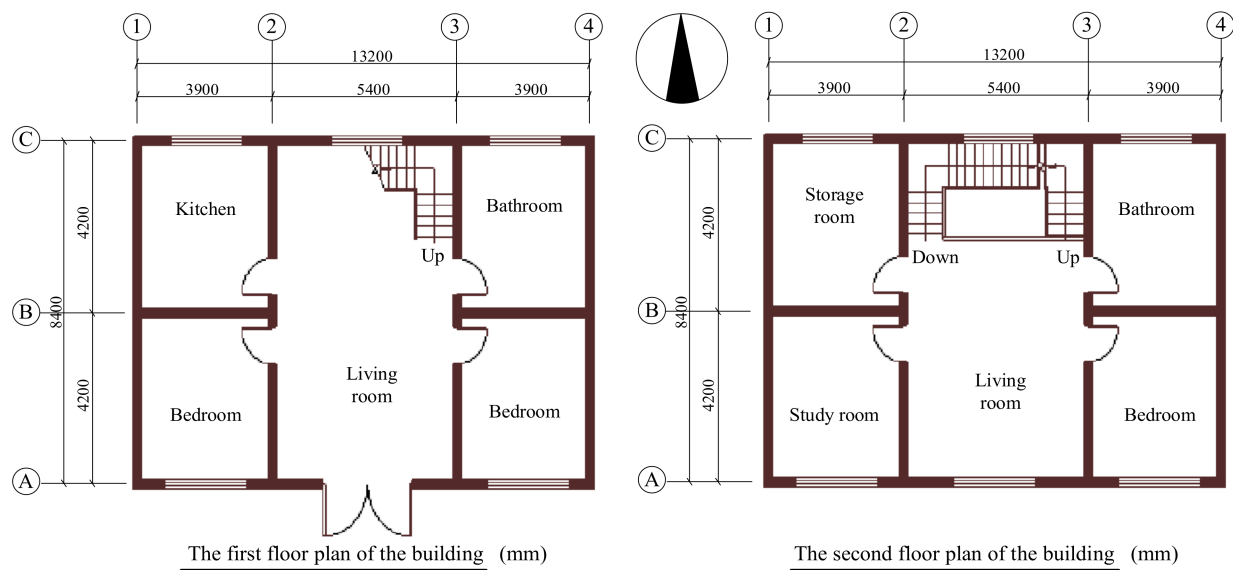
Figure 5. Floor plan of the representative building.
