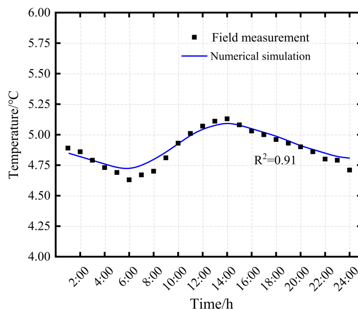
Figure 8. Comparison of measured and simulation results.
