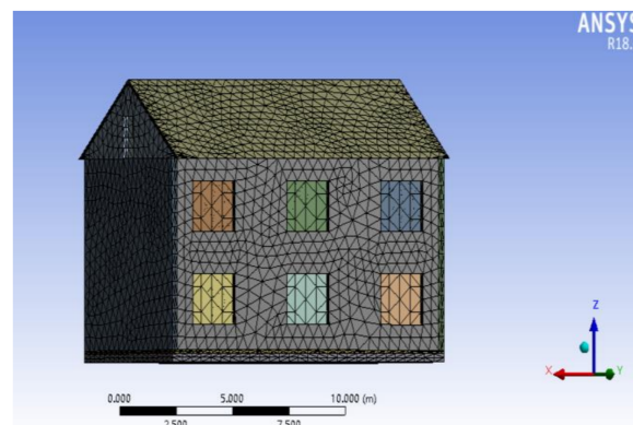
Figure 7. Refined mesh model.
