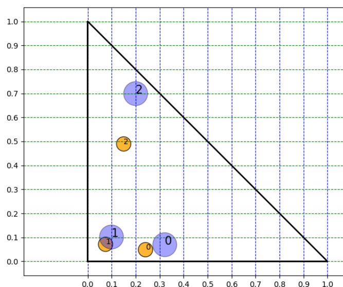
Figure 3. Triangular representation of A_{r_A}, B_{r_B} \in C - IFS(E) with E = \{0, 1, 2\} , C_E = 3 and r_A = 0.1 , r_B = 0.06 .
