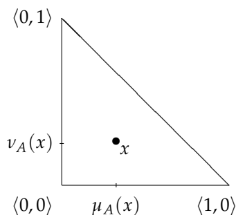
Figure 1. Geometrical interpretation of an element of an IFS.
