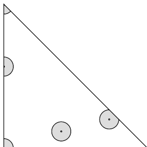
Figure 2. Geometric representation of different circular IFSs onto the IFS interpretation triangle.
