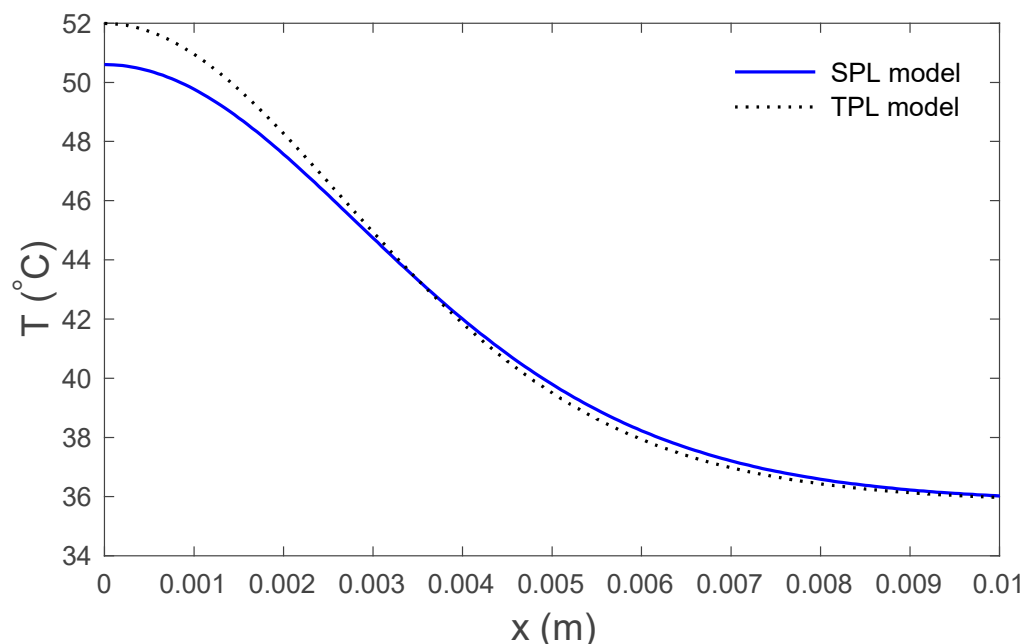
Figure 2. Variations in temperature versus the distance for the SPL and the TPL models.
