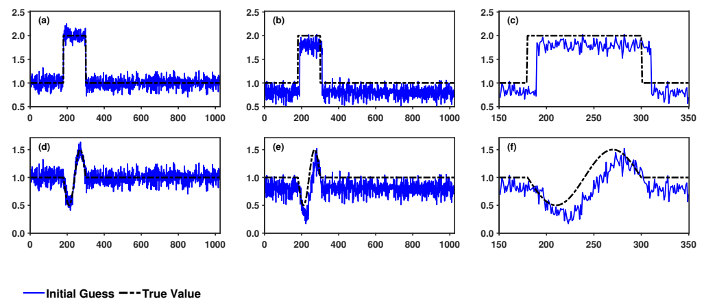
Figure 5. Different types of initial guesses. (a,d) correspond to \phi_g^1 and \phi_g^2 . (b,e) correspond to \phi_g^3 and \phi_g^4 . (c,f) show enlarged views of \phi_g^3 and \phi_g^4 over the interval x \in [150\Delta x, 350\Delta x] . The horizontal axis represents the spatial node index s in all subfigures, and the vertical axis denotes the corresponding solution \phi(x_s) , s = 0, 1, \dots, 1023 .
