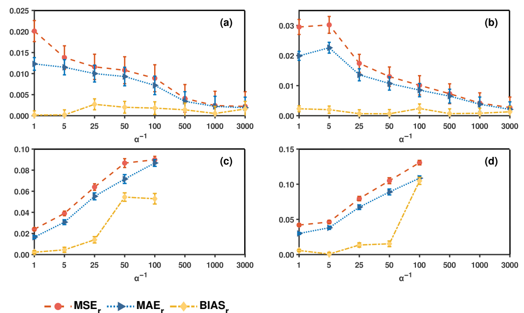
Figure 10. Variation in MSE_r , MAE_r , and BIAS_r with respect to the condition number of the background error covariance matrix. Error bars denote the error variance at each point. (a,b) show the errors of the corrected FTH- and WS-type initial guesses obtained using the AIKFI algorithm, respectively. (c,d) present the corresponding errors obtained using the l_1 -norm R4D-Var algorithm, which uses cross-validation to select regularization parameters [5]. The initial guess is \phi_g(x) = \phi(x) + \varepsilon same to (34c); the correlation length in the structure function of the background error covariance matrix varies within \alpha^{-1} \in \{1, 5, 25, 50, 100, 500, 1000, 3000\} , corresponding to condition numbers ranging from 10^2 to 10^{14} .
