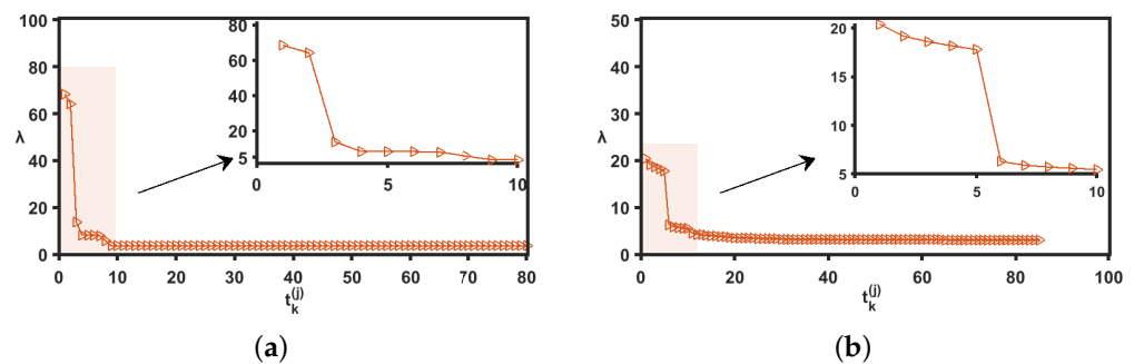
Figure 7. Adaptive regularization parameter selection during the correction process using the AIKFI algorithm. (a) Regularization parameter selection for the correction of \phi_g^3 . (b) Regularization parameter selection for the correction of \phi_g^4 . The horizontal axis denotes the computation time, whose relationship with the iteration index j and the observation time k is given by t_k^{(j)} = k(j-1) + k . The small image in the upper right corner of the figure represents an enlarged display of the shaded area.
