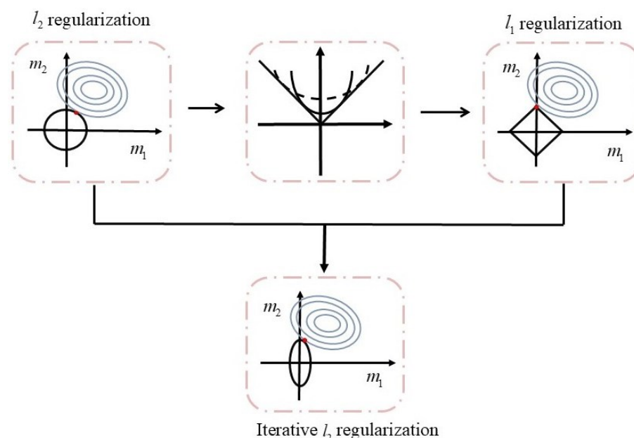
Figure 2. The technical roadmap for constructing the l_1 -norm surrogate function using the l_2 -norm.
