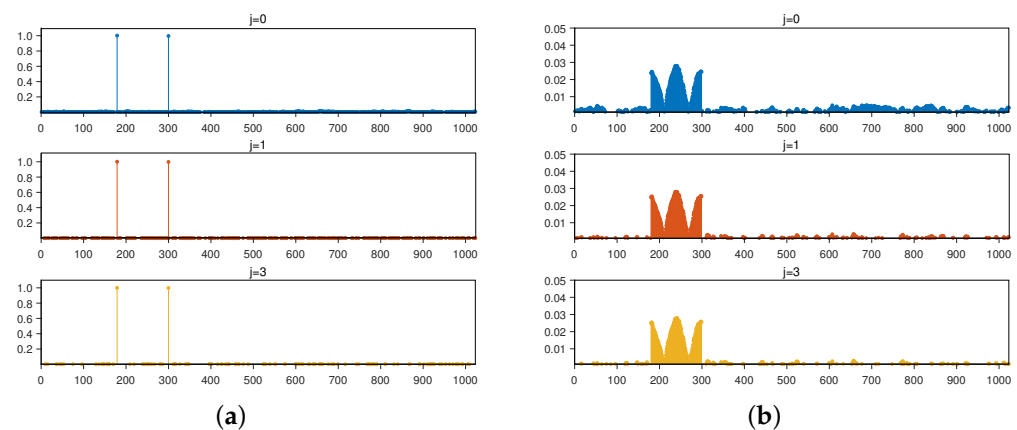
Figure 9. Sparsity evolution in the gradient information during the iterative correction process using the AIKFI algorithm. (a) Sparsity evolution for the correction of the initial guess \phi_g^5 in Figure 8a. (b) Sparsity evolution for the correction of the initial guess \phi_g^6 in Figure 8d. The j denotes the iteration index. The horizontal axis represents point s = 1, 2, \dots, 1023 , while the vertical axis denotes the corresponding gradient information of the initial guess \mathbf{m} = \mathbf{Lm} \in \mathbb{R}^{1023} .
