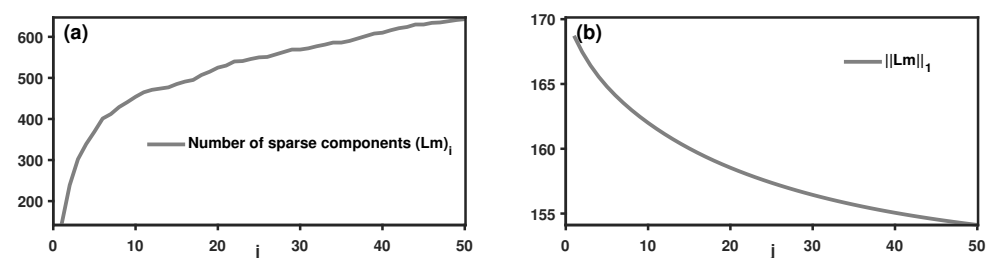
Figure 4. Evolution of the Sparsity of Gradient Information \mathbf{Lm} During the Correction of 4 \times 4 km Observations Using the Iterative Sparse Regularization Kalman Filter. (a) Variation in the number of sparse components (\mathbf{Lm})_i < 10^{-2} of the gradient information throughout the correction process. (b) Variation in the l_1 -norm \|\mathbf{Lm}\|_1 of the gradient information throughout the correction process.
