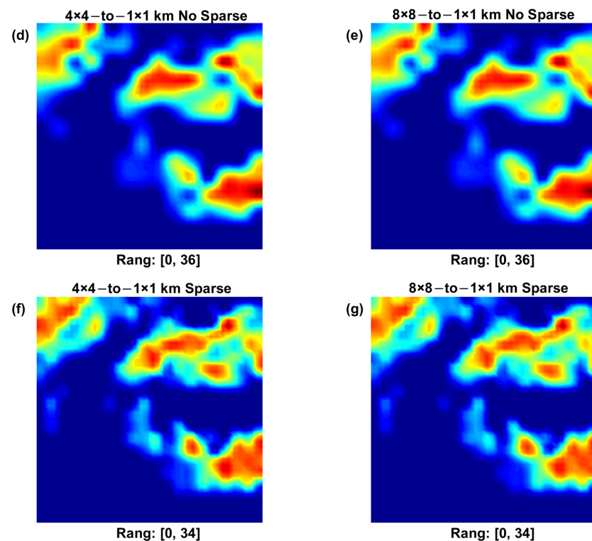
Figure 3. Reconstruction effect in extreme rainfall area. (a) True rainfall reflectivity. (b,c) 4 \times 4 km and 8 \times 8 km observations. (d,e) Correction results without sparse regularization. (f,g) Correction results with sparse regularization.
