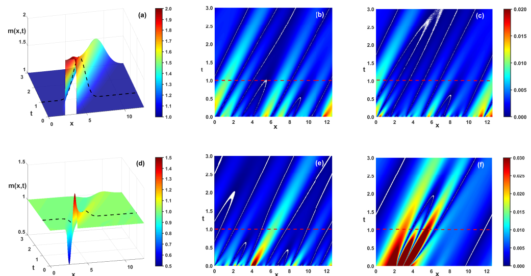
Figure 11. Error in the spatial evolution between the assimilation results and the true states. The dotted line in the figure represents the end of the assimilation window where T = 1 . (a,d) show the evolution of the true states for FTH-type and WS-type, respectively. (b,e) present the absolute errors of the spatial evolution of the analyzed states corresponding to Figure 8c,f relative to the true evolution. (c) depicts the absolute error of the evolution result for the corrected WS-type initial guess in Figure 8a using a fixed regularization parameter in AIKFI, while (f) shows the corresponding error for the corrected WS-type initial guess in Figure 8d obtained with the unconstrained f-slope method.
