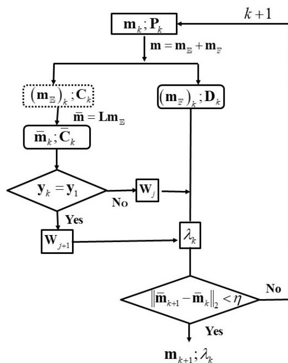
Figure 1. The schematic diagram of the AIKFI algorithm.
