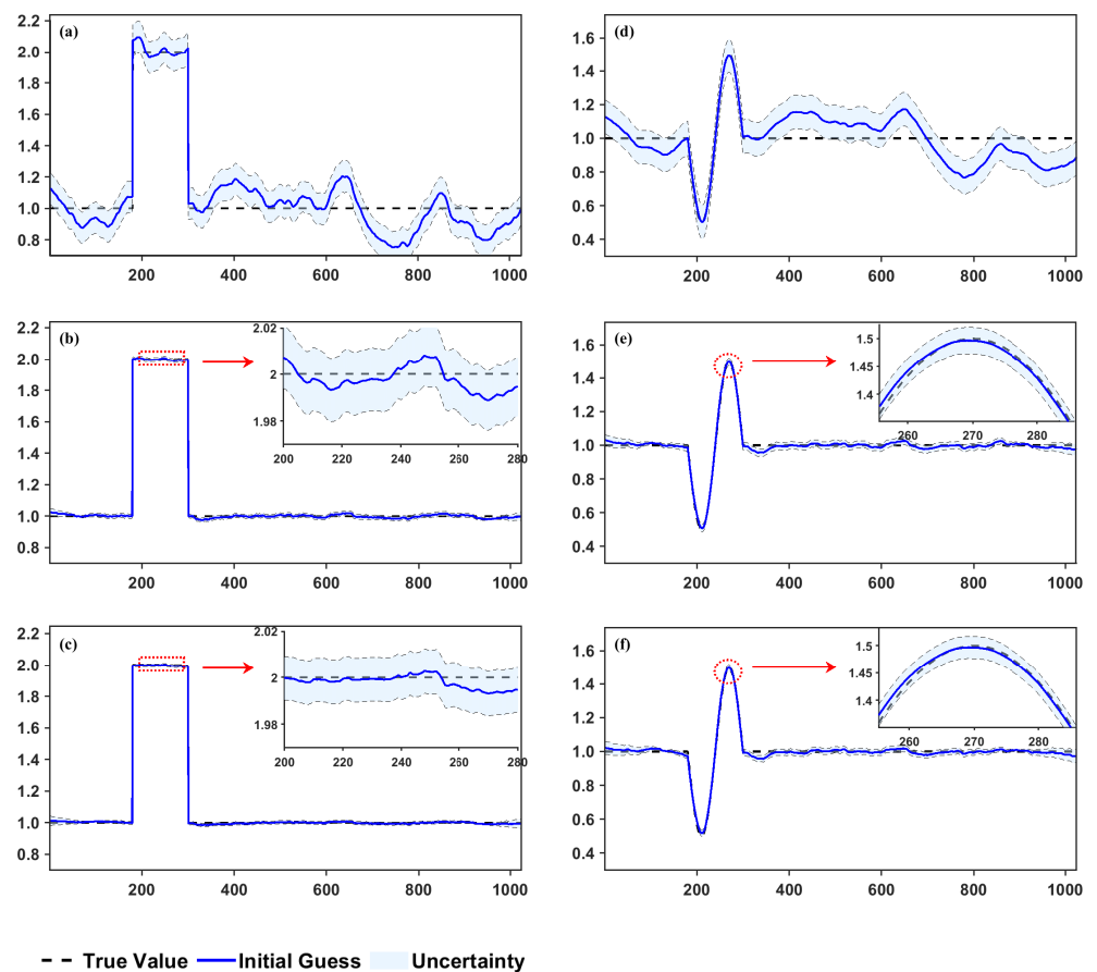
Figure 8. Iterative assimilation performance and uncertainty evolution during the correction process using the AIKFI algorithm. (a,d) show the initial guesses \phi_g^5 and \phi_g^6 together with their uncertainties, where the correlation lengths in the structure function of the background error covariance matrix are set to \alpha^{-1} = 25 and \alpha^{-1} = 50 , respectively. (b,e) present the assimilation results and their uncertainties after 1st iteration of the AIKFI algorithm for \phi_g^5 and \phi_g^6 . (c,f) display the final results, i.e., the assimilation results and their uncertainties after the 3rd iteration.
