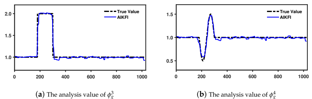
Figure 6. Correction results of the initial guesses \phi_g^3 and \phi_g^4 via the AIKFI algorithm.
