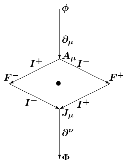
Figure 1. Simplest case of conformal invariant differential operators F^\pm depict the duality decomposition of the electromagnetic eld F_{\mu\nu} . A_\mu , resp., J_\mu , is the electromagnetic potential, resp., the current. I^\pm depict the differential operators which come from the equation \partial_{[\mu} A_{\nu]} = F_{\mu\nu} . Knapp–Stein operators relate cases symmetric w.r.t. the central black dot.
