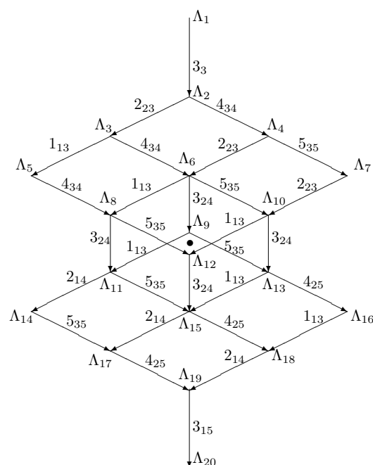
Figure 2. Main multiplets for sl(6, \mathbb{R}) .
