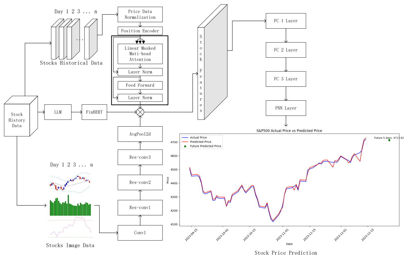
Figure 2. LLM-Augmented Linear Transformer-CNN Framework.
