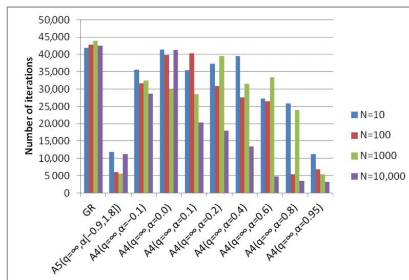
Figure 11. Number of iterations of the algorithms GR, A4(q, \alpha) , A5(q, \alpha[a, b]) required to achieve a given accuracy for different \alpha values from initial point x_2 . Function f_{EELX}(x) = (1 - x_1)^2 + 100 \left( 1 - \sum_{i=1}^n \frac{x_i^2}{10^{i-1}} \right)^2 + \frac{1}{2} \sum_{i=1}^n \frac{x_i^2}{10^{i-1}} .
