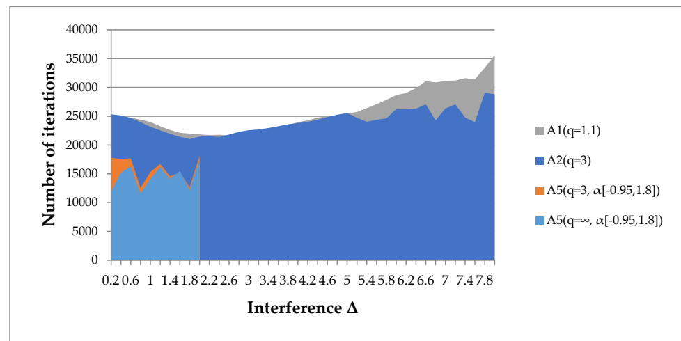
Figure 10. Number of iterations of the algorithms A1(q) , A2(q) , A4(q, \alpha) , A5(q, \alpha[a, b]) required to achieve a given accuracy with interference from the initial point x_2 . N = 100 , function f_{EEL}(x) = (1 - x_1)^2 + 30 \left( 1 - \sum_{i=1}^n \frac{x_i^2}{10^{i-1}} \right)^2 .
