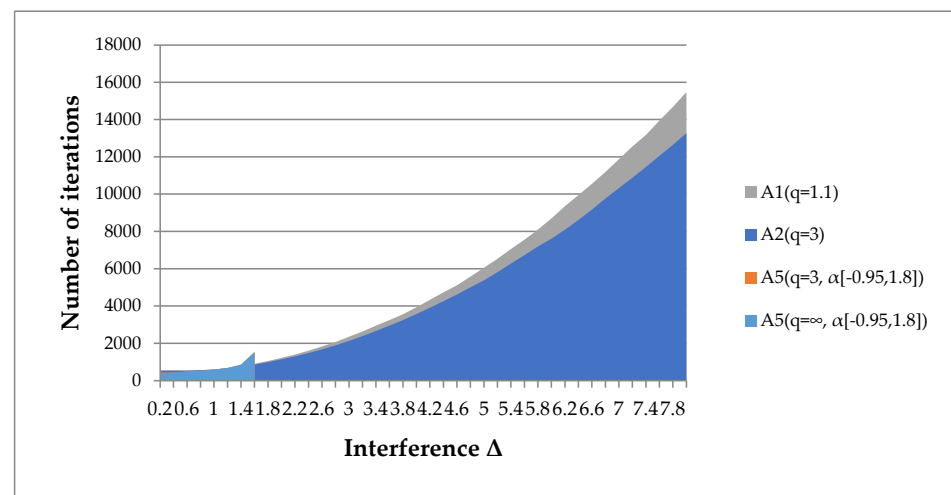
Figure 16. Number of iterations of the algorithms A1( q ), A2( q ), A4( q, \alpha ), A5( q, \alpha[a, b] ) required to achieve a given accuracy with interference. N = 1000 , function f_R(x) = \sum_{i=1}^n \frac{100 \frac{i-1}{n-1}}{10} (e^{x_i} - x_i - 1) .
