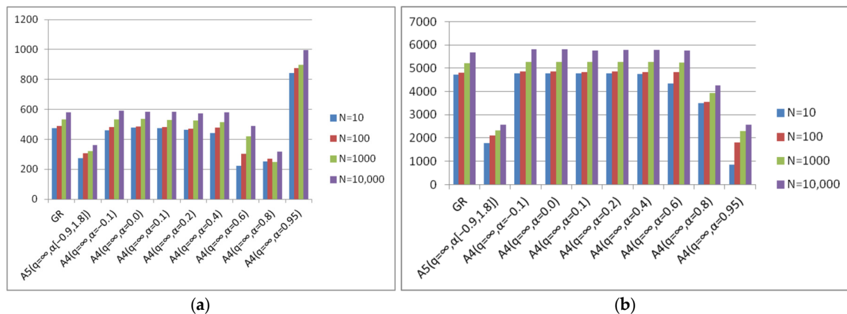
Figure 15. Number of iterations of the algorithms GR, A4( q, \alpha ), A5( q, \alpha[a, b] ) required to achieve a given accuracy for different \alpha values (a) Function f_R(x) = \sum_{i=1}^n \frac{i-1}{10} (e^{x_i} - x_i - 1) ; (b) Function f_R(x) = \sum_{i=1}^n \frac{1000 \frac{i-1}{n-1}}{10} (e^{x_i} - x_i - 1) .
