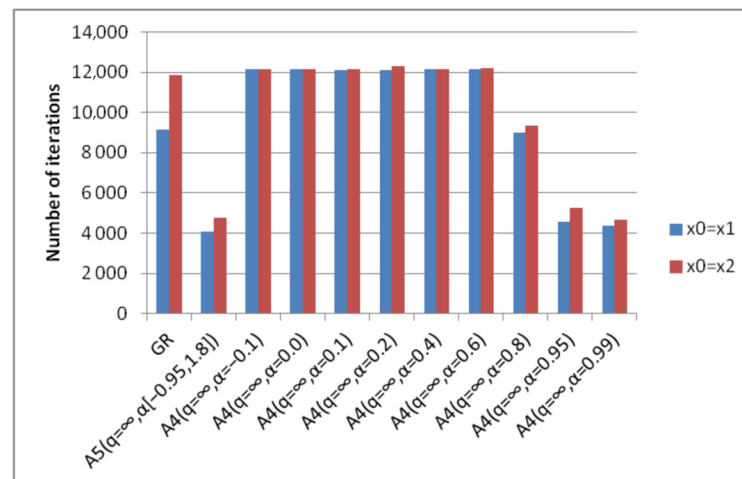
Figure 2. Number of iterations of the algorithms GR, A4( q, \alpha ), A5( q, \alpha[a, b] ) required to achieve a given accuracy for different \alpha values from initial points x_1 and x_2 . Function f_R(x) = 100(x_2 - x_1^2)^2 + (x_1 - 1)^2 .
