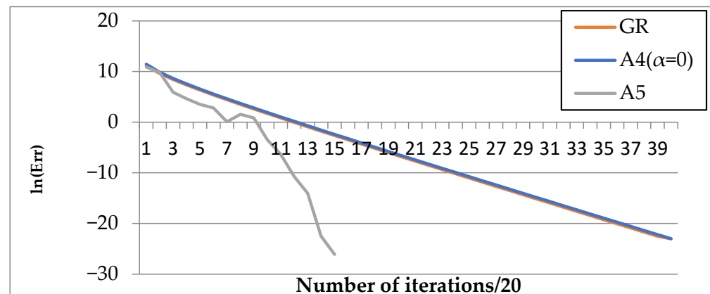
Figure 17. Minimization error in logarithmic scale against number of iterations with 20-iteration step.
