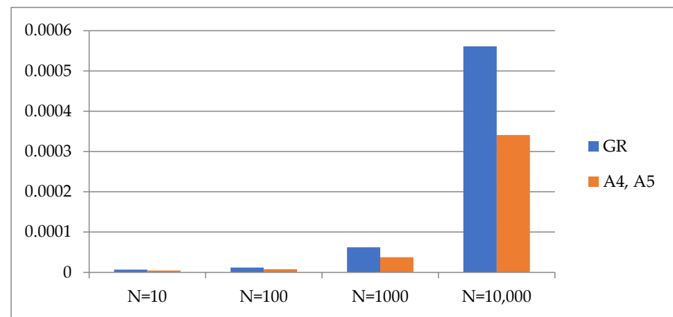
Figure 18. Iteration runtime (s) for the function f_{EEL}(x, [a_{max} = 10, b_{max} = 10]) . GR is gradient method; A4 and A5 are the new methods with step adaptation.
