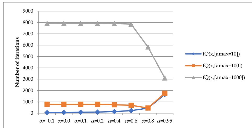
Figure 19. The effect of parameter \alpha on convergence rate in Algorithm A4(q = \infty, \alpha) for the function f_Q .
