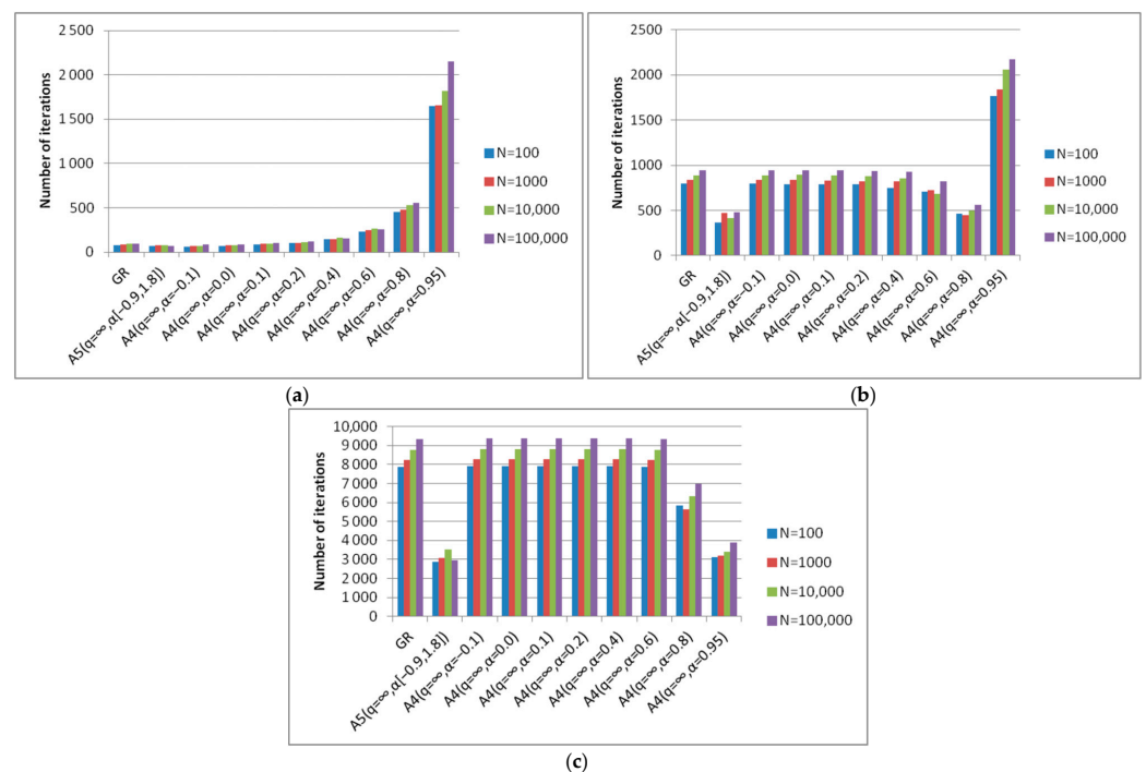
Figure 4. Number of iterations of the algorithms GR, A4(q, \alpha) , A5(q, \alpha[a, b]) required to achieve a given accuracy for different \alpha values (a) Function f_Q(x) = \frac{1}{2} \sum_{i=1}^n 10 \frac{i-1}{n-1} x_i^2 ; (b) Function f_Q(x) = \frac{1}{2} \sum_{i=1}^n 100 \frac{i-1}{n-1} x_i^2 ; (c) f_Q(x) = \frac{1}{2} \sum_{i=1}^n 1000 \frac{i-1}{n-1} x_i^2 .
