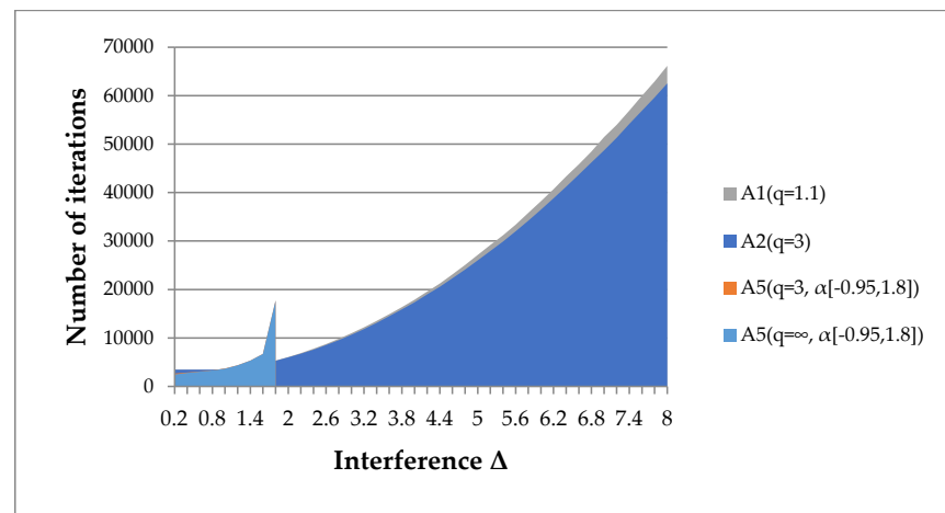
Figure 14. Number of iterations of the algorithms A1(q) , A2(q) , A4(q, \alpha) , A5(q, \alpha[a, b]) required to achieve a given accuracy with interference. N = 1000 , function f_{Q2}(x) = \left(\sum_{i=1}^n 1000^{\frac{i-1}{n-1}} x_i^2\right)^2 .
