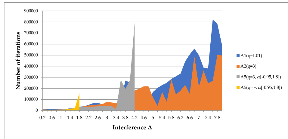
Figure 3. Number of iterations of the algorithms A1(q) , A2(q) , A4(q, \alpha) , A5(q, \alpha[a, b]) required to achieve a given accuracy from initial point x_1 with interference. Function f_R(x) = 100(x_2 - x_1^2)^2 + (x_1 - 1)^2 .
