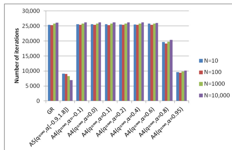
Figure 9. Number of iterations of the algorithms GR, A4(q, \alpha) , A5(q, \alpha[a, b]) required to achieve a given accuracy for different \alpha values from the initial point x_2 . Function f_{EEL}(x) = (1 - x_1)^2 + 30 \left( 1 - \sum_{i=1}^n \frac{x_i^2}{10^{n-1}} \right)^2 .
