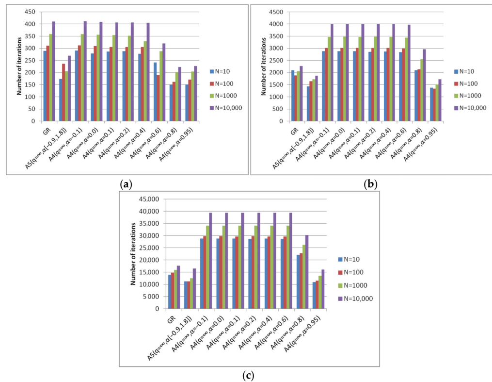
Figure 13. Number of iterations of the algorithms GR, A4(q, \alpha) , A5(q, \alpha[a, b]) required to achieve a given accuracy for different \alpha values (a) Function f_{Q2}(x) = \left(\sum_{i=1}^n 100^{\frac{i-1}{n-1}} x_i^2\right)^2 ; (b) Function f_{Q2}(x) = \left(\sum_{i=1}^n 1000^{\frac{i-1}{n-1}} x_i^2\right)^2 ; (c) f_{Q2}(x) = \left(\sum_{i=1}^n 10000^{\frac{i-1}{n-1}} x_i^2\right)^2 .
