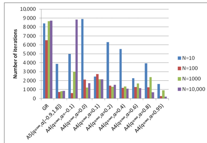
Figure 6. Number of iterations of the algorithms GR, A4(q, \alpha) , A5(q, \alpha[a, b]) required to achieve a given accuracy for different \alpha values from the initial point x_2 . Function f_{EEL}(x) = (1 - x_1)^2 + 10 \left( 1 - \sum_{i=1}^n \frac{x_i^2}{10^{\frac{i-1}{n-1}}} \right)^2 .
