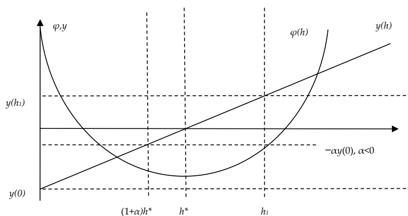
Figure 1. Function \phi(h) and its derivative.
