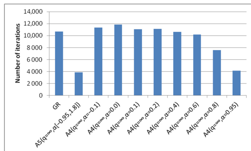
Figure 20. Average number of iterations among all test functions without interference.
