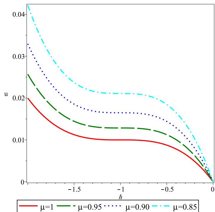
Figure 9. \hbar -curve of u(t) at t = 0.01 for various values of \mu .
