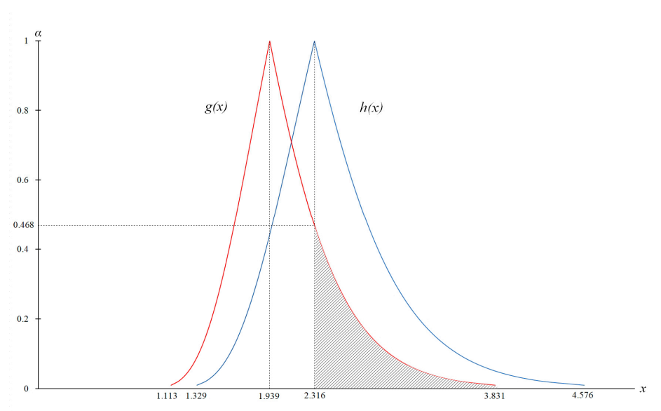
Figure 3. Membership functions g(x) and h(x) for numerical example.
