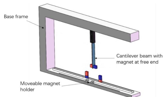
Figure 13. Possible experimental implementation.
