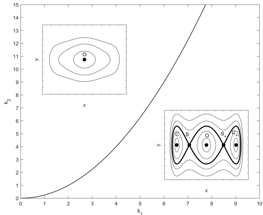
Figure 2. Orbits of the unperturbed system (6) under different values of k_1 and k_2 .
