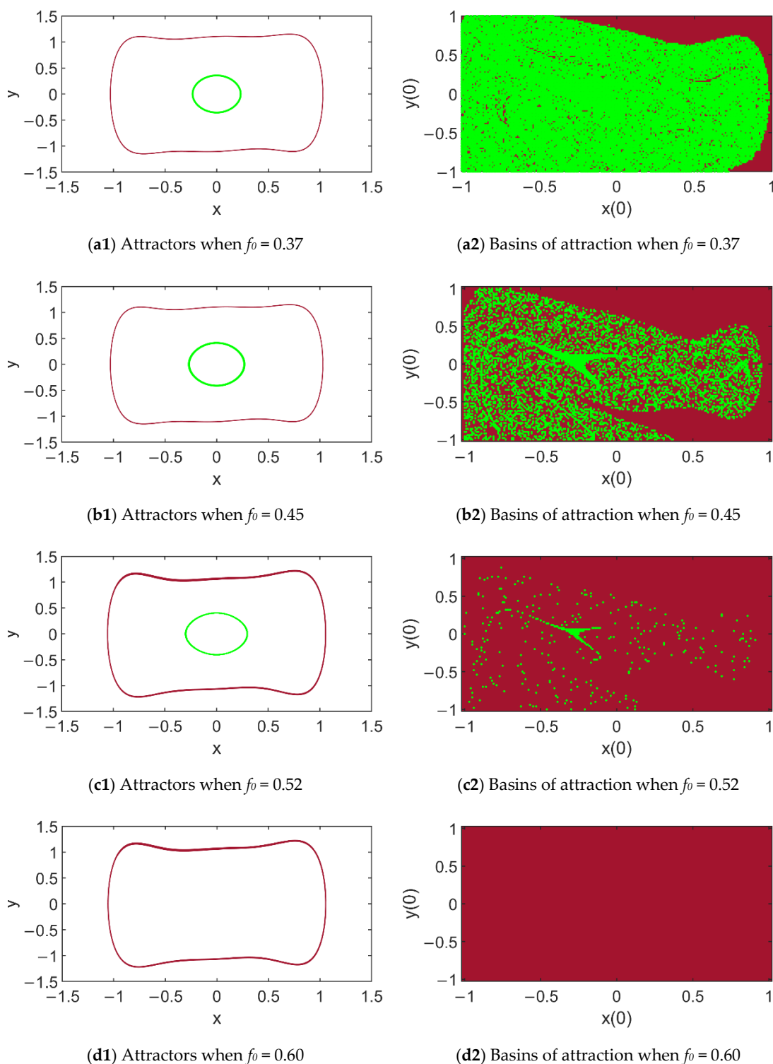
Figure 10. Sequences of attractors and their basins of attraction for f_0 ranging from 0.37 to 0.60.
