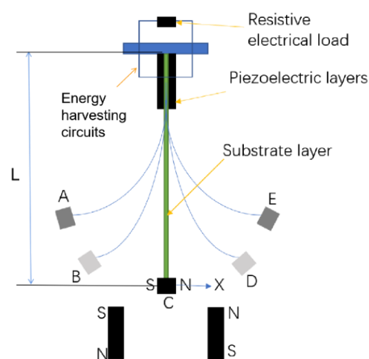
Figure 1. Simplified diagram of a tristable piezoelectric cantilever energy harvester.
