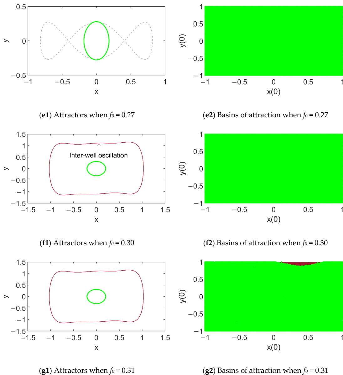
Figure 8. Sequences of attractors and their basins of attraction for f_0 ranging from 0.089 to 0.31.
