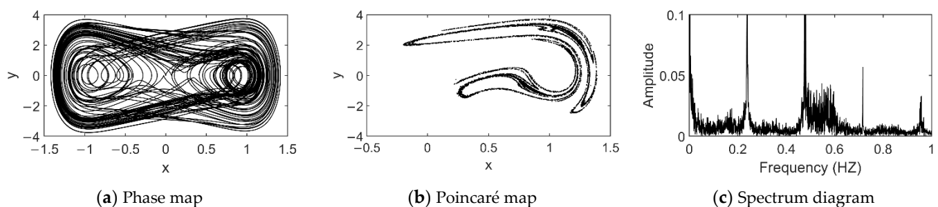
Figure 12. Chaos of the system (5) for f_0 = 4.2 .
