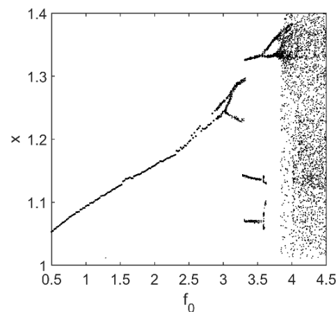
Figure 11. Bifurcation diagram under different values of f_0 .
