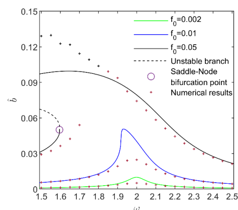
Figure 5. Variation of the amplitude of periodic solution near (\pm x_c, 0) with the change of \omega .
