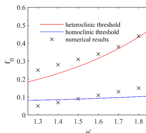
Figure 9. f_0^{homo} and f_0^{hetero} of system (5) versus the excitation frequency \omega .
