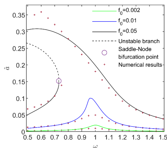
Figure 3. Variation of the amplitude of periodic solutions near (0, 0) with the change of \omega .
