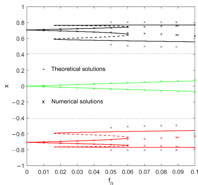
Figure 6. Variation of the periodic solutions with the amplitude of f_0 when \omega = 1.5 .
