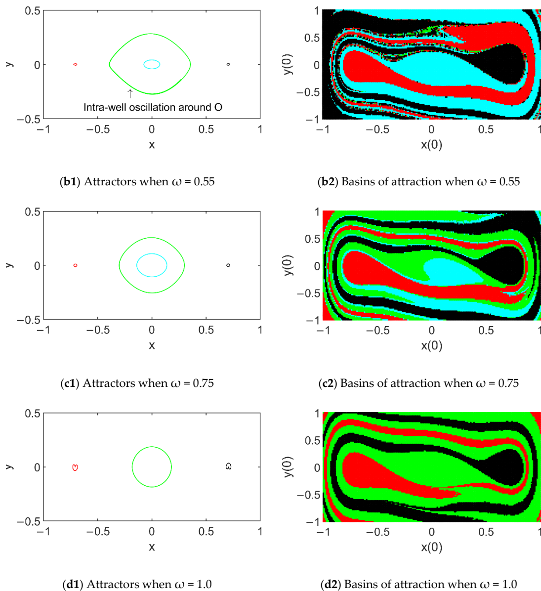
Figure 4. Evolution of attractors and their basins of attraction with the increase of \omega for f_0 = 0.05 .
