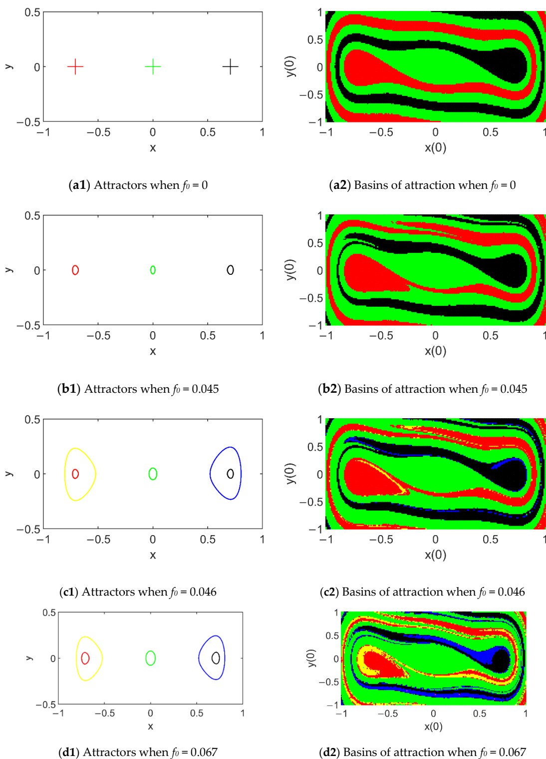
Figure 7. Evolution of attractors and their basins of attraction with the increase of f_0 for \omega = 1.5 .
