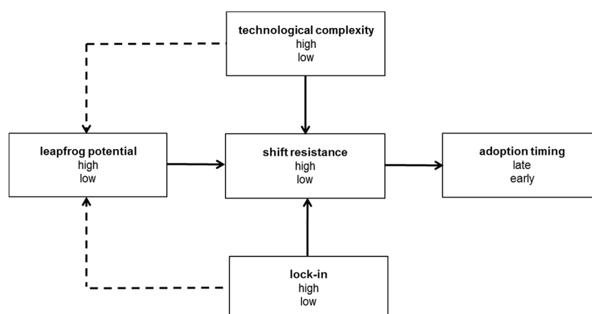
Figure 1. Analysis framework.
