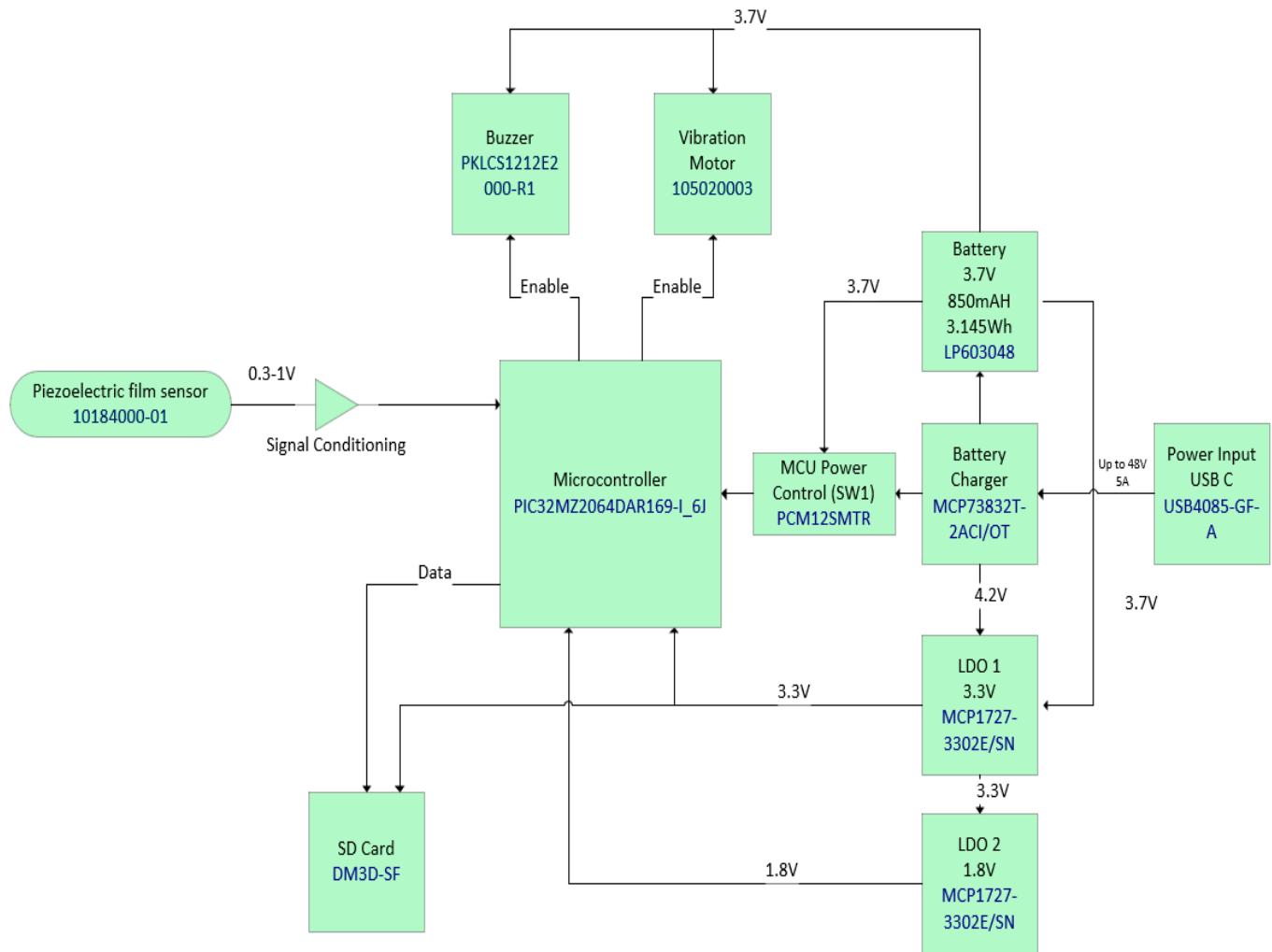
Figure 2. RespyBelt hardware components interconnections and their types.
