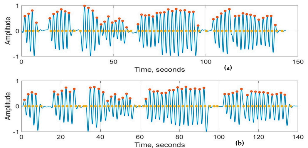
Figure 8. Respiration signals obtained from (a) RespyBelt and (b) SOMNOtouch (red dots represent detected peaks and yellow dots represent detected zero-crossing time points). The sections with missing respiratory cycles are due to the pauses in breathing. The signal amplitude does not have a unit as it is normalised to \pm 1 .
