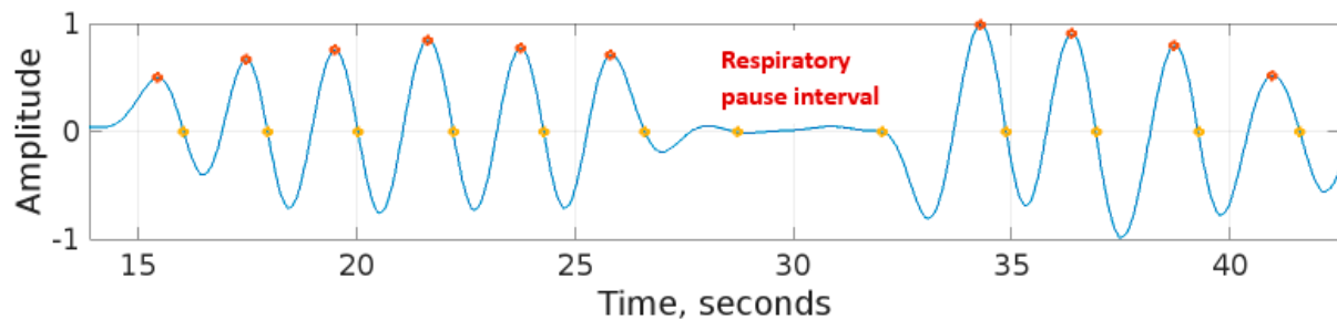
Figure 11. A respiratory signal recorded by RespyBelt indicating the respiratory pause centred around 30 s. The zero-crossing method identified two spurious respiratory cycles during this interval. The signal amplitude does not have a unit as it is normalised to \pm 1 .
