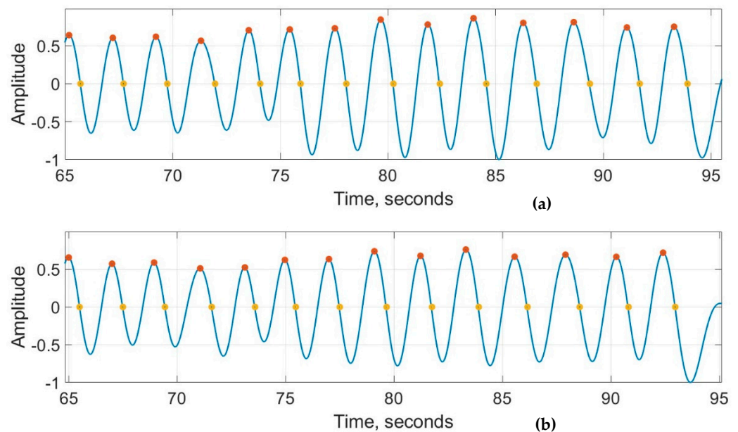
Figure 9. Zoomed in respiration signals obtained from (a) RespyBelt and (b) SOMNOtouch (red dots represent detected peaks and yellow dots represent detected zero-crossing time points). The signal amplitude does not have a unit as it is normalised to \pm 1 .
