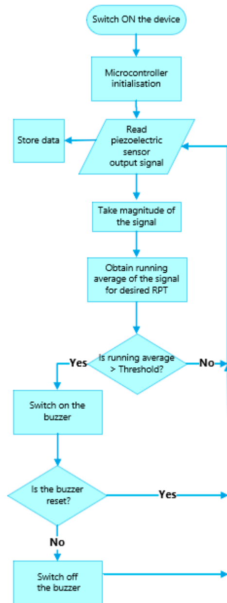
Figure 7. Flowchart of the RespyBelt software operating in real-time (RPT: respiratory pause time), indicating the manner respiratory pauses are detected.
