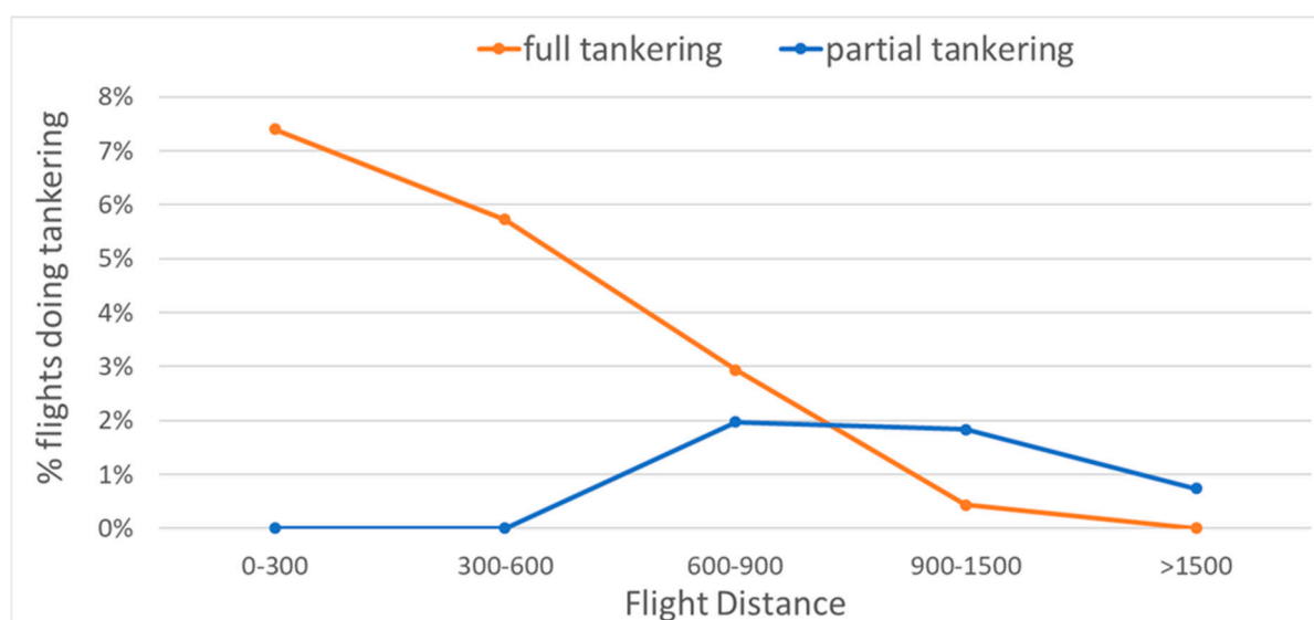
Figure 14. % of flights which could exercise fuel tankering (and save money by doing so), per distance flown.
