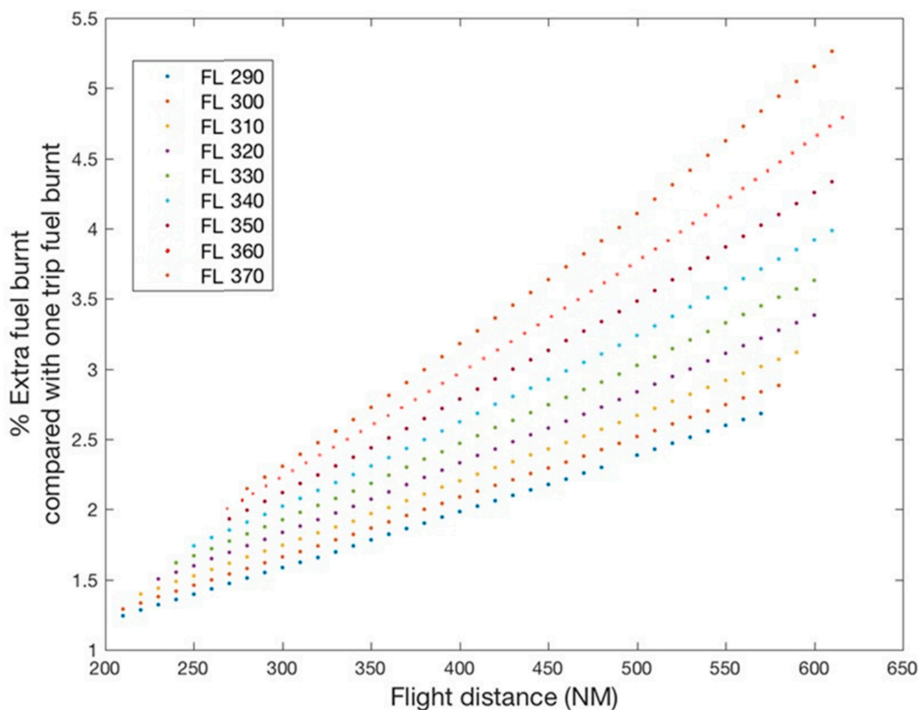
Figure 2. % of extra fuel burnt for full fuel tankering on various flight distances for a specific aircraft model.
