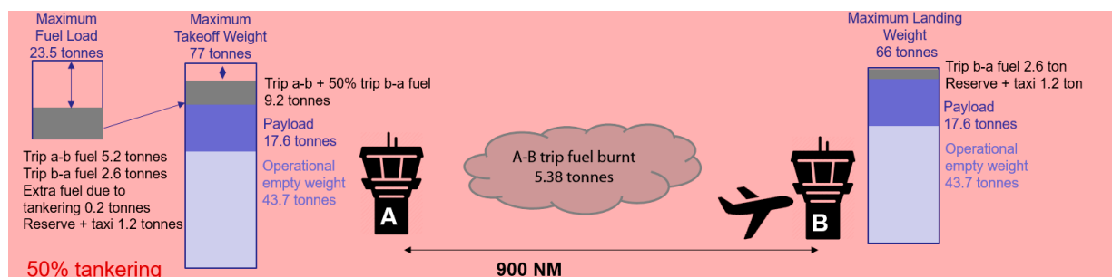
Figure 8. Example for a 900 NM flight performing a 50% partial fuel tankering.
