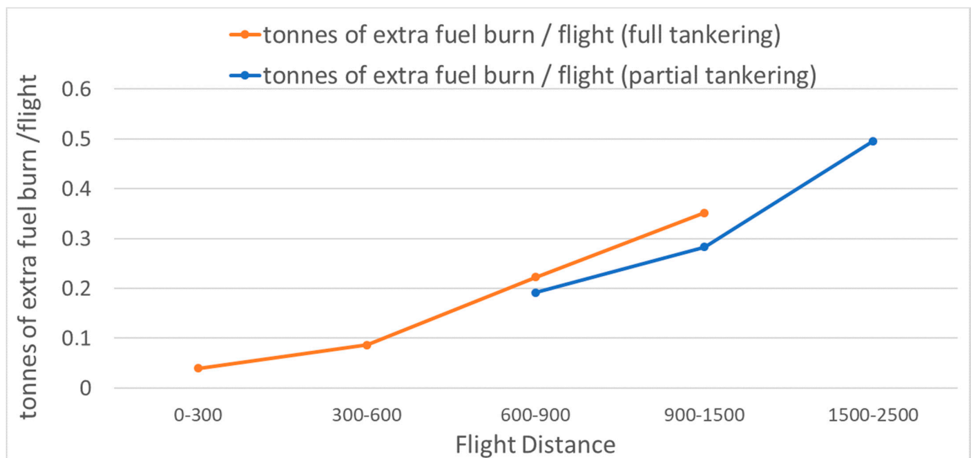
Figure 15. Extra fuel burn per distance flown.
