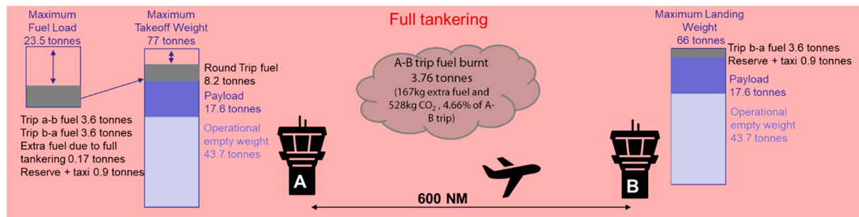
Figure 6. Example for a 600 NM flight performing a full (100%) tankering.
