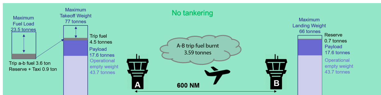
Figure 5. Example for a 600 NM flight with no tankering.
