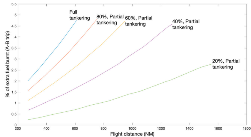
Figure 9. % of extra fuel burn as a function of % of tankering and distance flown for a specific aircraft model.
