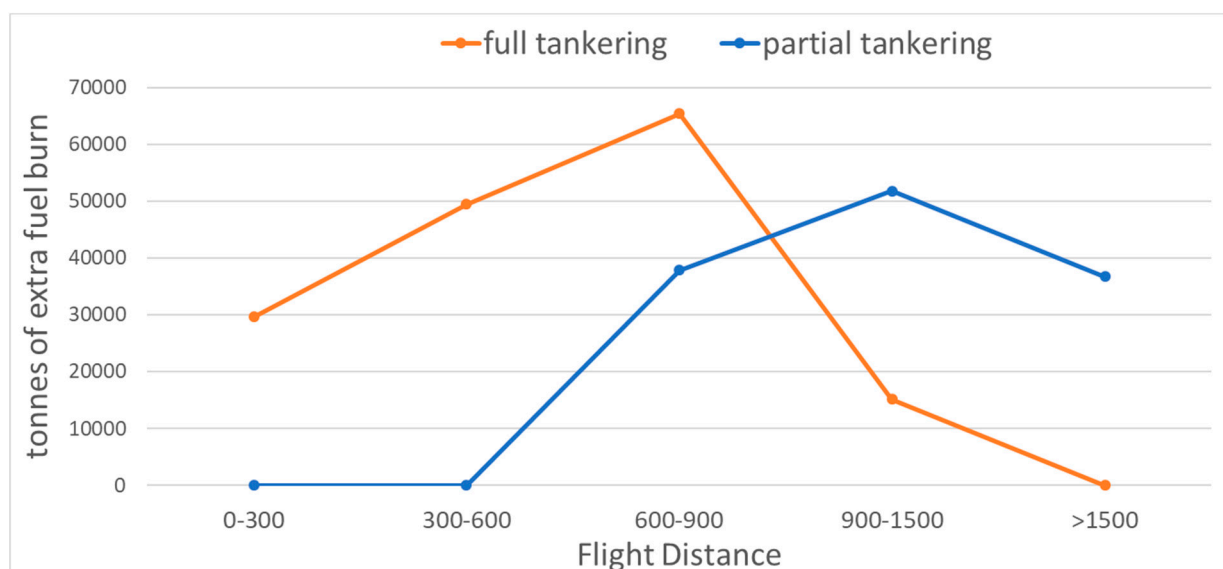
Figure 16. Tonnes of extra fuel burn per distance flown.
