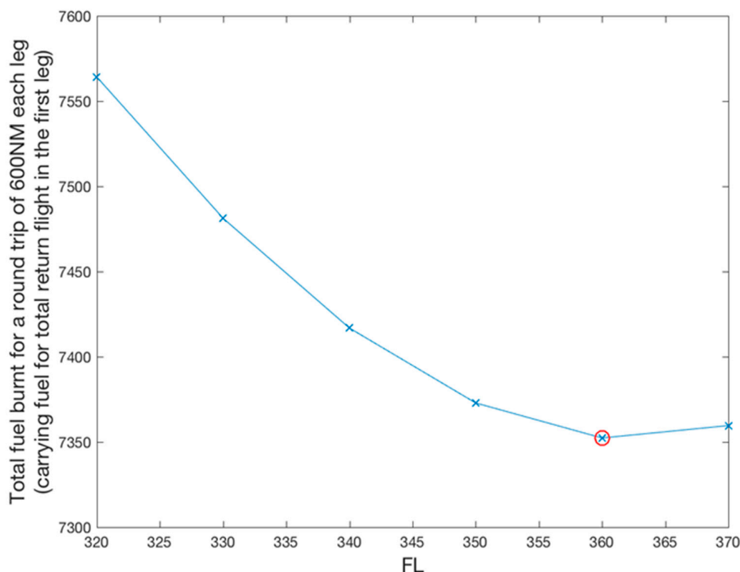
Figure 3. Total fuel burnt (kg) for full fuel tankering at various flight levels (hundreds of feet).
