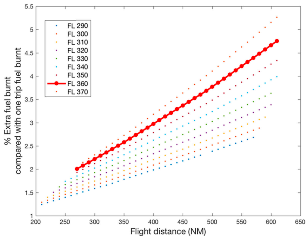
Figure 4. % of extra fuel burnt for various flight distances for a specific aircraft mode with optimum flight cruise level determined.
