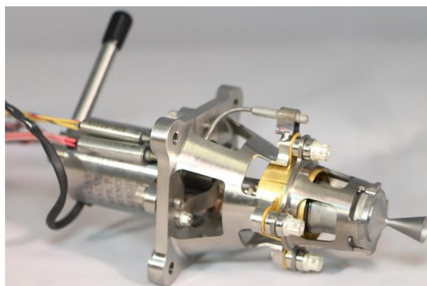
Figure 11. GR1 Thruster [32].
