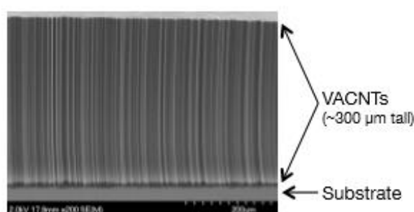
Figure 2. Vertically aligned Carbon Nanotube “Forest” under an electron microscope, forest height 300 \mu\text{m} [9].
