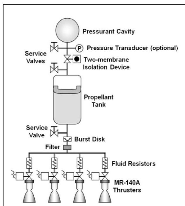
Figure 13. CHAMPS Functional Schematic [32].
