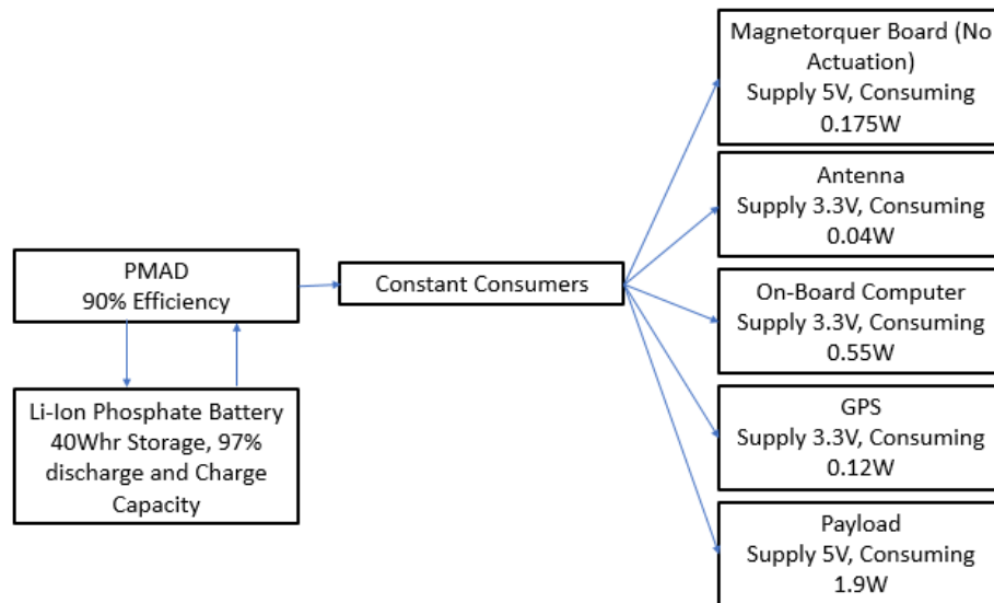
Figure 42. Constant Consumers Cold Case Block Diagram.
