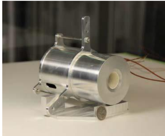
Figure 22. University of Toronto SFL Hall Effect Thruster [23].
