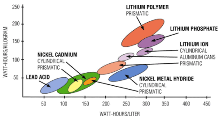
Figure 8. Battery Energy Densities [29].
