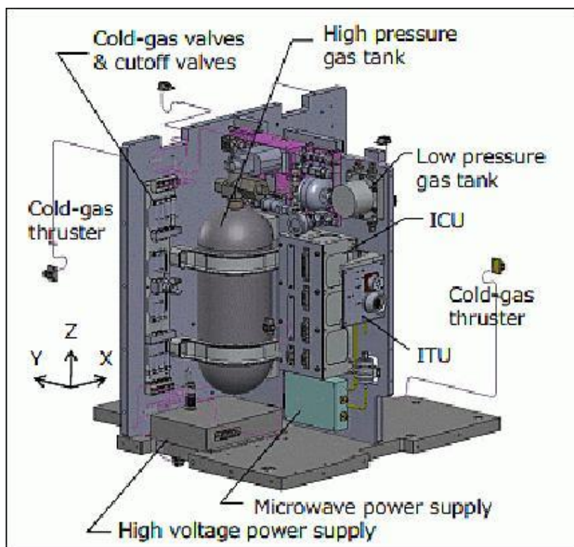
Figure 14. Cold Gas Thruster (eoPortal Directory, 2002) [33].
