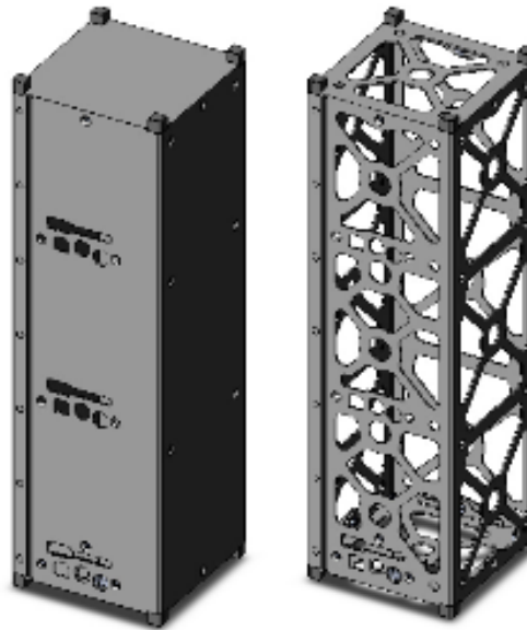
Figure 32. 3U Monocoque Walled Primary Structure (Pumpkin Incorporated, 2015) [48].
