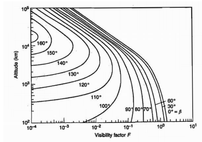
Figure 45. Visibility Factor Alterations against Orbit Altitude [10,63].
