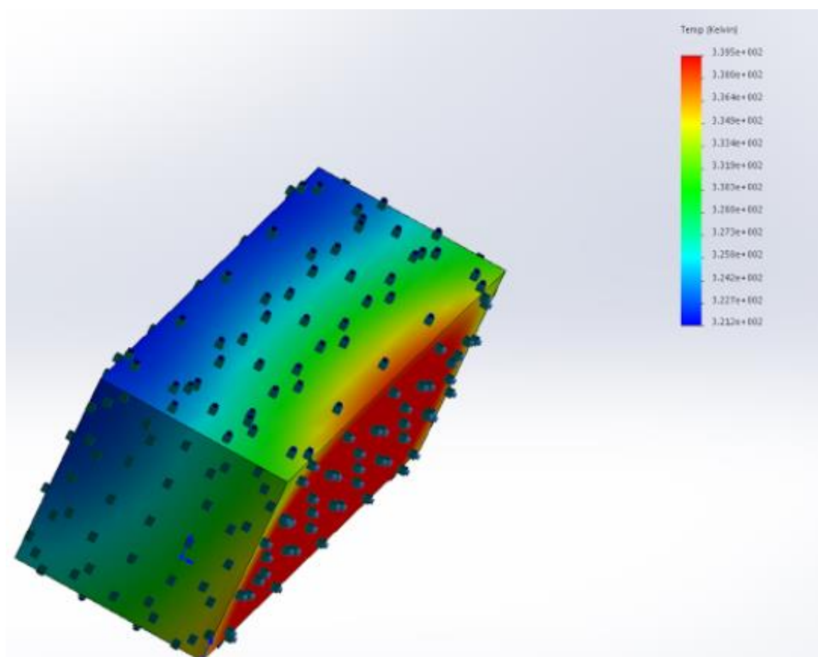
Figure 58. Hot-case Temperature Gradient with Power Dissipation of 0.7995 W.
