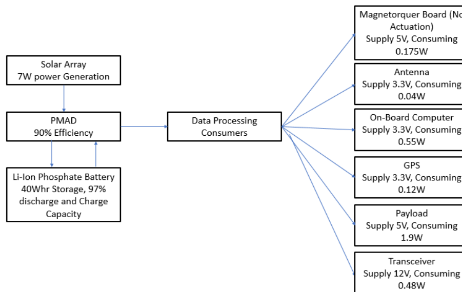
Figure 40. Data Processing Block Diagram.
