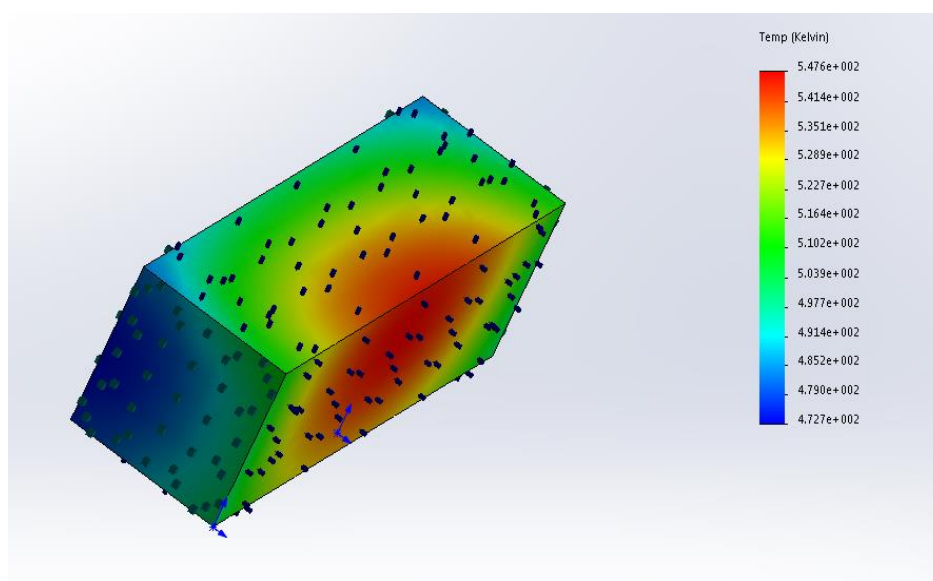
Figure 54. Initial Steady-state Simulation Results end of the Heating Phase.
