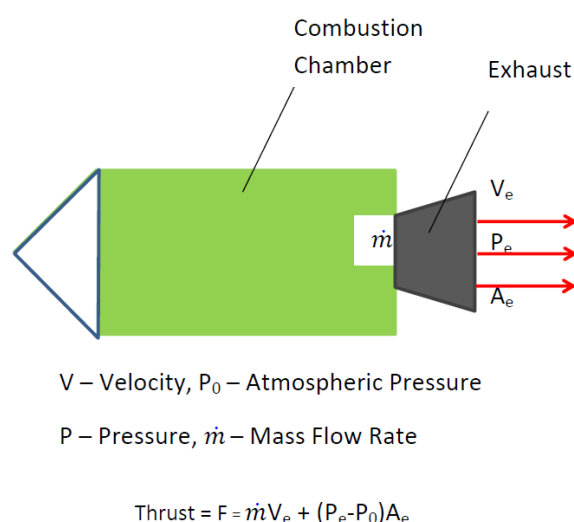
Figure 16. Physics of a Solid Rocket Motor [31].
