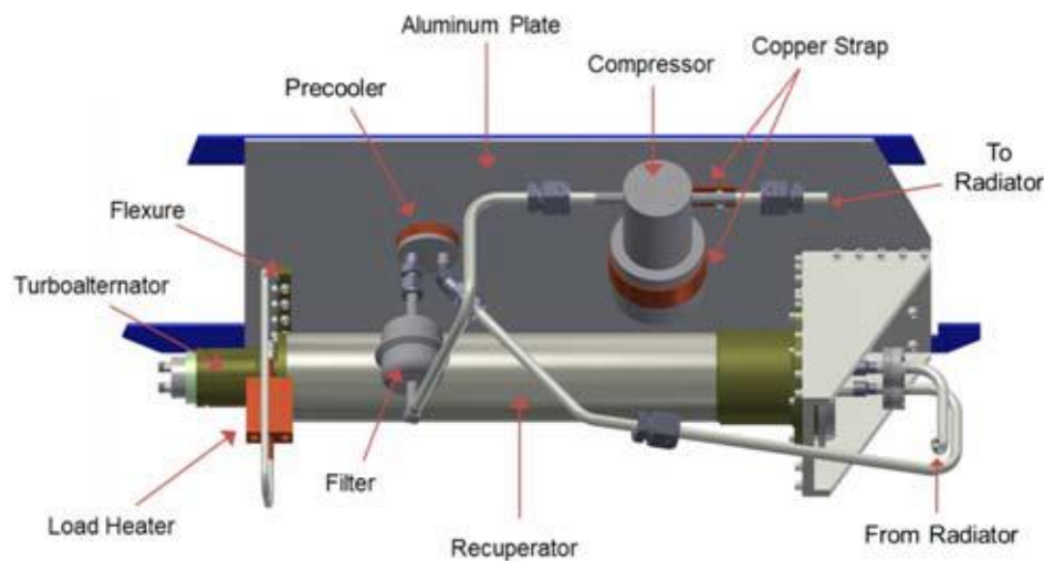
Figure 26. Mechanical Cryo-Cooler Configuration [23].
