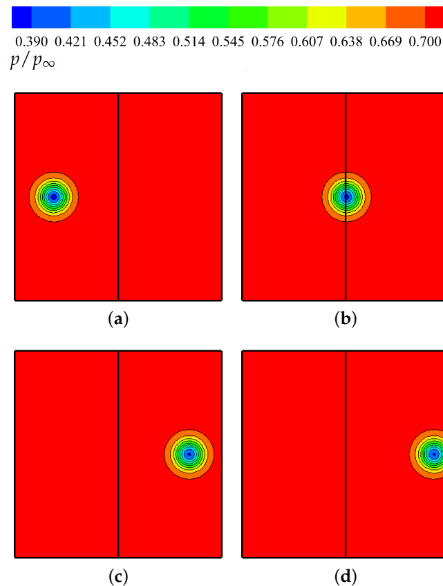
Figure 9. Pressure contours showing vortex convection across a block-interface boundary and illustrating its transparent nature to the flow. (a) t \times a_\infty / L_{ref} = 0 ; (b) t \times a_\infty / L_{ref} = 3.5 ; (c) t \times a_\infty / L_{ref} = 7 ; (d) t \times a_\infty / L_{ref} = 7.8 .
