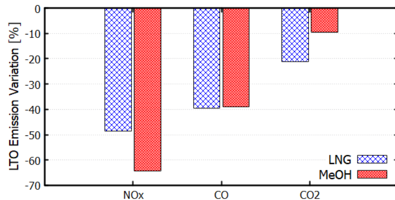
Figure 11. Set-thrust: LTO \text{NO}_x , CO and \text{CO}_2 variation of LNG and MeOH-powered GTF, relative to its baseline Jet-A operation.
