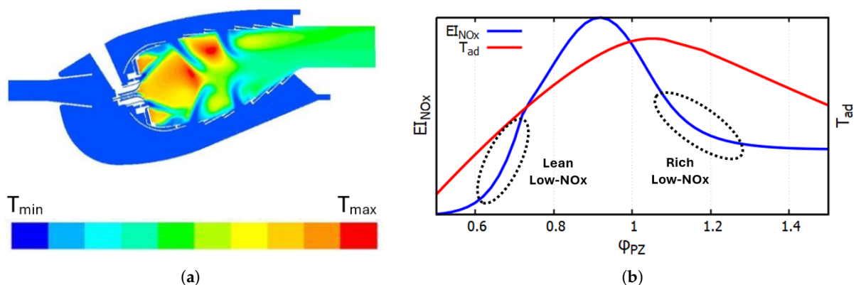
Figure 6. TalonX characteristics. (a) RQL burner-family cross-section with qualitative temperature contours [39]. (b) Qualitative EI_{\text{NO}_x} & T_{ad} vs \phi_{PZ} map for the TalonX at TO conditions.
