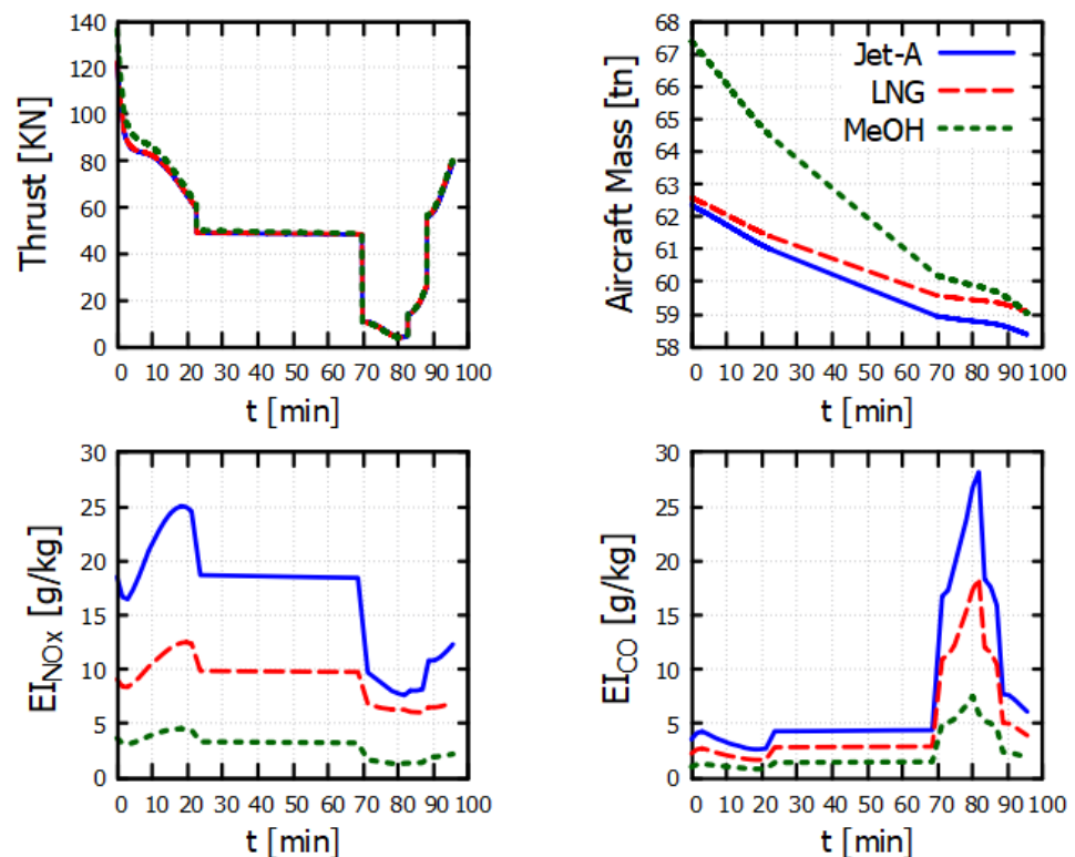
Figure 17. Thrust, aircraft total mass and EI time series for the London–Barcelona mission.
