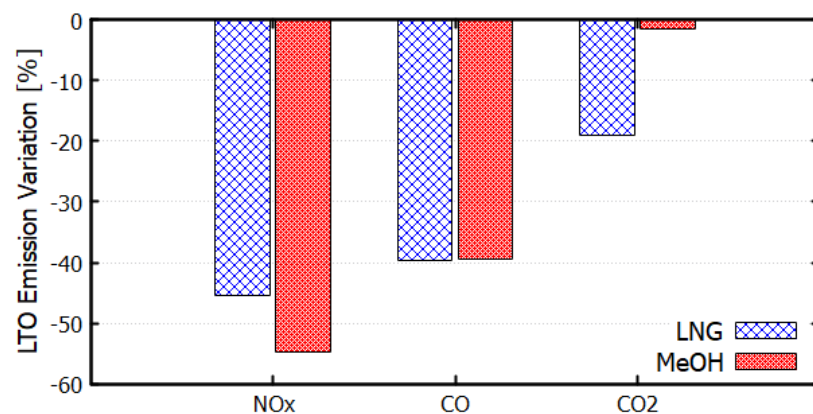
Figure 15. Set-TIT: LTO \text{NO}_x , CO and \text{CO}_2 variation of LNG and MeOH-powered GTF, relative to its baseline Jet-A operation.
