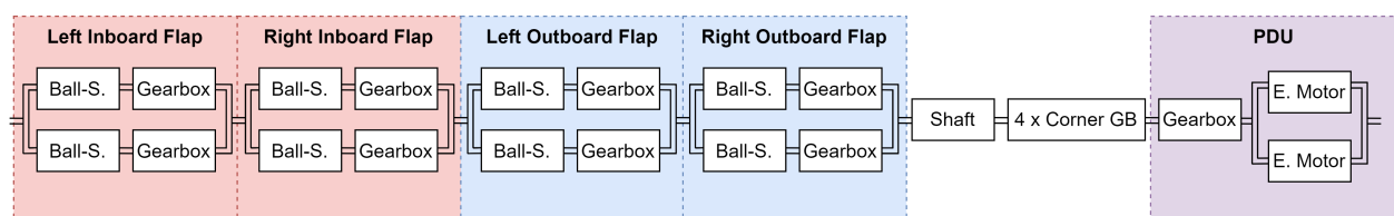
Figure 4. RBD of the conventional flap system.
