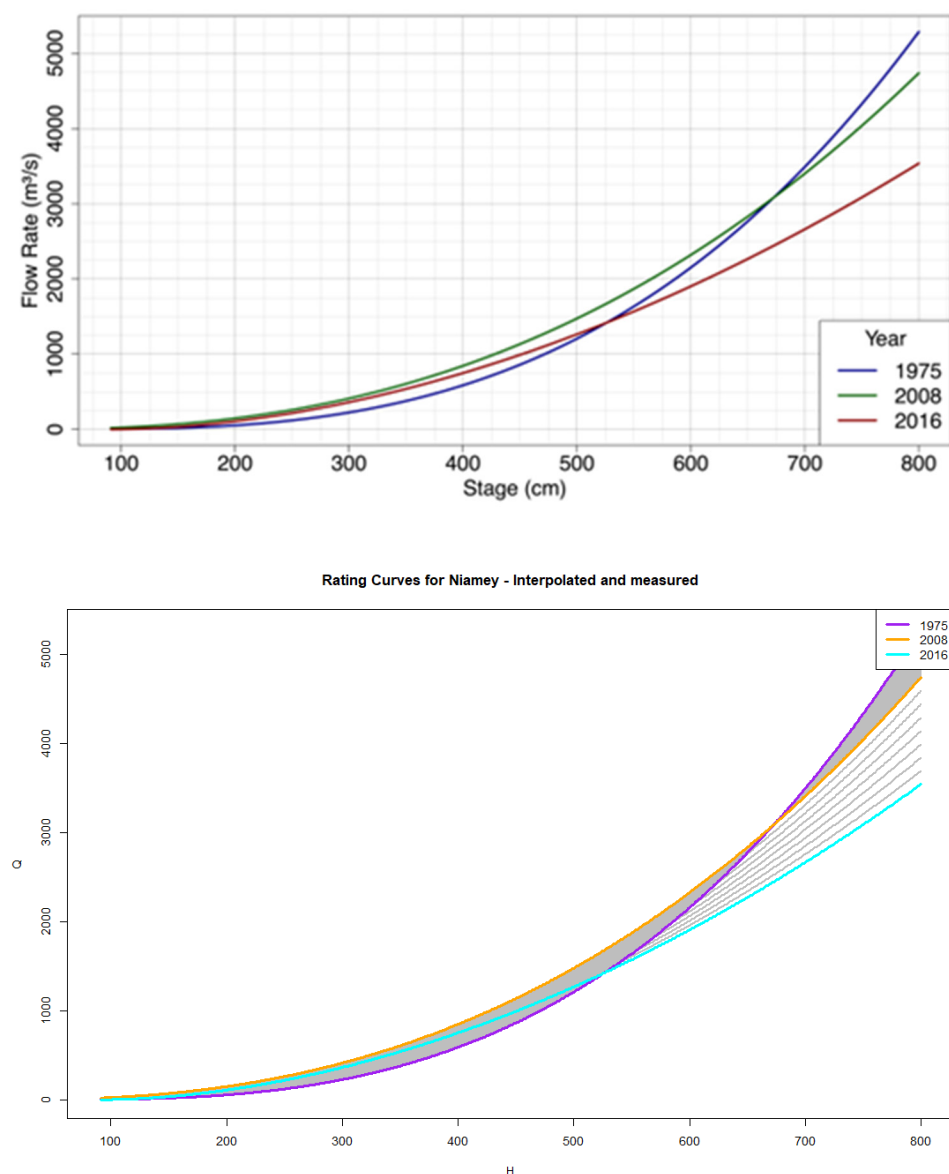
Figure 2. Graphical representation of the available rating curves (source: Directorate of Water Resources, Ministry of Hydraulics, Sanitation and Environment of Niger).
