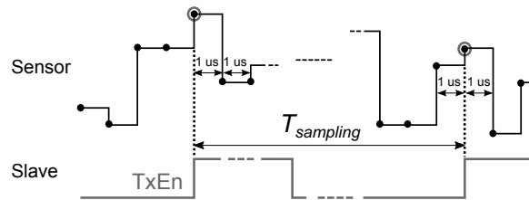
Figure 14. Capturing of the sensor values at the rising edges of the transmit enable (TxEn) signal with the sampling step T_{\text{sampling}} .
