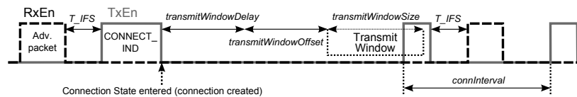
Figure 6. Transmit Window. After receiving the advertising packet form the slave, master sends the CONNECT_IND packet to the slave and transitions to the Connection State. The start of the first data packet, which determines the anchor point for the first connection event, and therefore the timings of all future connection events in this connection, is no earlier than transmitWindowDelay + transmitWindowOffset and no later than transmitWindowDelay + transmitWindowOffset + transmitWindowSize after the end of the CONNECT_IND packet ( transmitWindowDelay = 1.25 ms).
