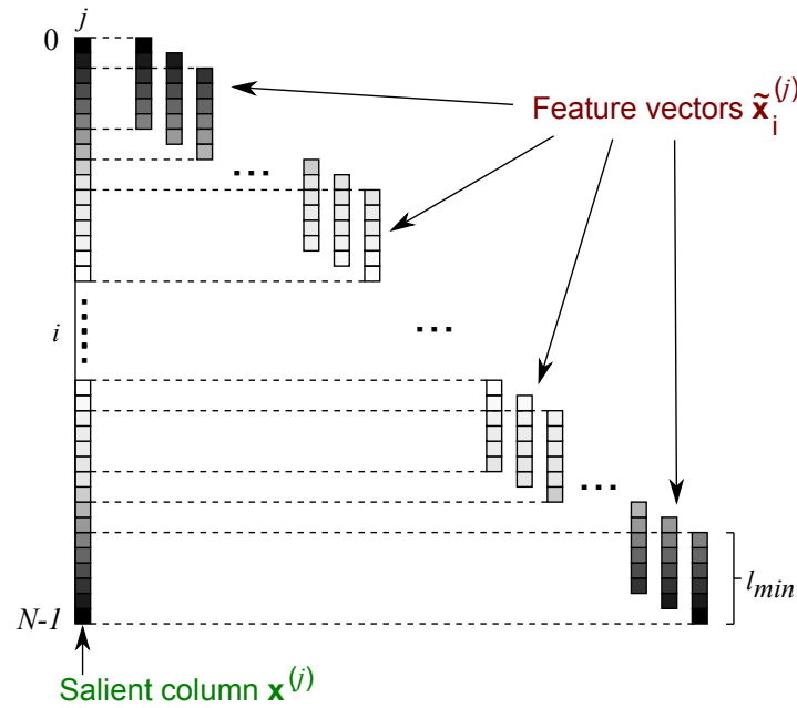
Figure 16. Extracting feature vectors \tilde{\mathbf{x}}_i^{(j)} from a salient column \mathbf{x}^{(j)} (represented as grey values) leads to a set S^{(j)} = \{\tilde{\mathbf{x}}_0^{(j)}, \dots, \tilde{\mathbf{x}}_{N-1-l_{min}}^{(j)}\} of feature vectors.
