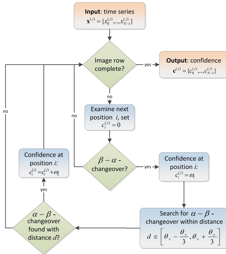
Figure 10. Flow chart for constructing confidence vectors \mathbf{c}^{(j)} for a particular time series \mathbf{x}^{(j)} . Input and output is visualized in Figure 11a,c. \alpha represents predefined marker candidate pixels based on the RGB color model and \beta represents pixels from the rest of the image.
