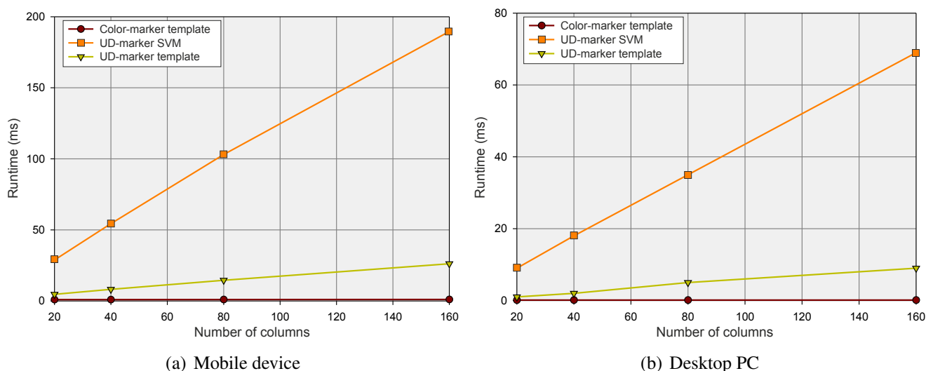
Figure 24. Runtimes for different marker detection methods on (a) a mobile device (Intel i5M 2.53 GHz, 4 GB RAM, Windows 7 64 bit) and (b) an desktop PC (Intel i5 2.80 GHz, 8 GB RAM, Windows 7 64 bit).
