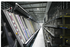
(a) A-frame [7]
