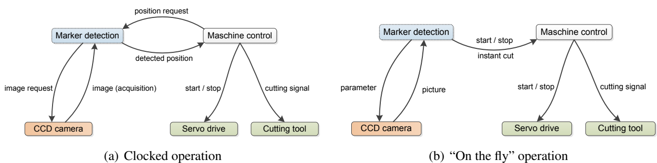
Figure 5. Interaction of the sensor (red) and actuators (green) in terms of two controlling strategies of the picking system: (a) clocked and (b) “on the fly” mode of operation. Figure 8 depicts the details of the “marker detection” module (dashed) which are presented throughout this paper. It serves as the (algorithmic) interface between the sensor and actuators.
