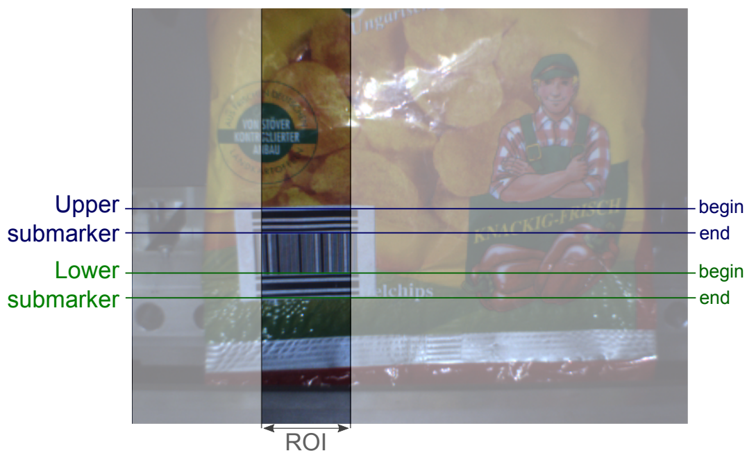
Figure 14. Definition of the Region of Interest (ROI) and the vertical bounds of the upper and lower marker parts within the ROI.
