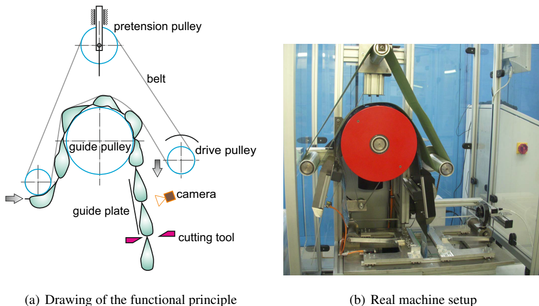
Figure 4. Drawing of the functional principle and the needed components (a) and the real setup at the Fraunhofer Institute for Material Flow and Logistics (b).
