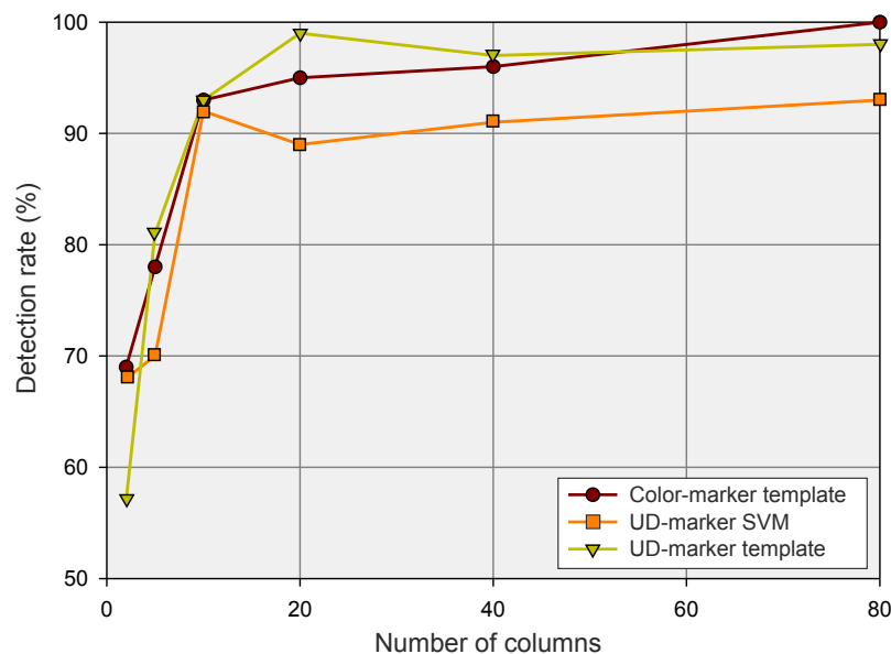
Figure 25. Trade-off consideration between the detection quality and the number of columns: the detection rate (%) depends on the number of salient columns as input for the marker detection algorithms Color-Marker_Template , UD-Marker_SVM and UD-Marker_Template .
