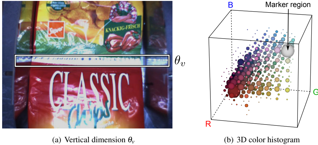
Figure 9. Model of the color based marker depending on the (a) vertical image dimension \theta_v of the marker and (b) the three dimensional RGB histogram. The size of the spheres symbolizes the pixel count in the subquads.
