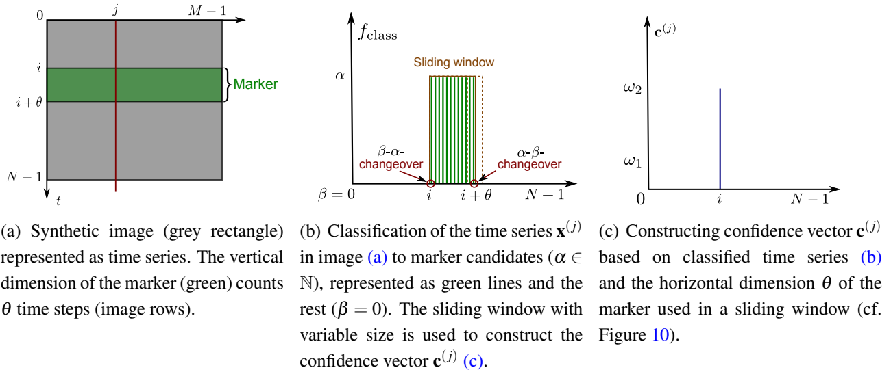
Figure 11. Classification of time series \mathbf{x}^{(j)} of a synthetic image shown in (a) to marker candidates ( \alpha \in \mathbb{N} ) and no marker time steps ( \beta = 0 ). The subsequent process of constructing a confidence vector \mathbf{c}^{(j)} based on (b) is depicted in (c).
