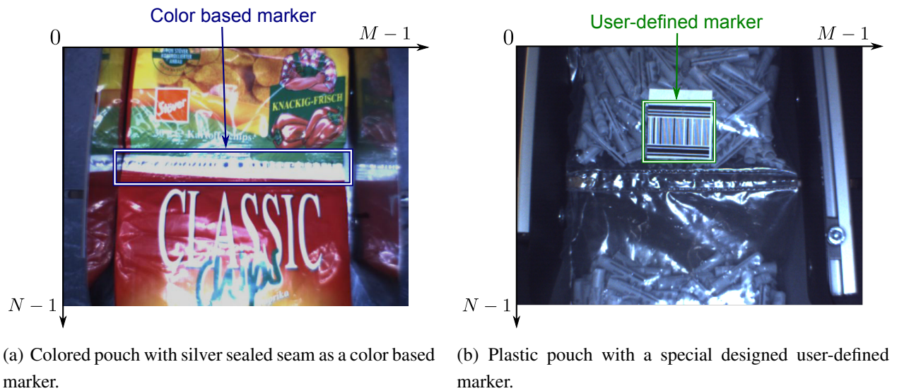
Figure 6. Two different types of marker: (a) a silver sealed seam as a color based marker and (b) a plastic pouch with a specially designed user-defined marker.
