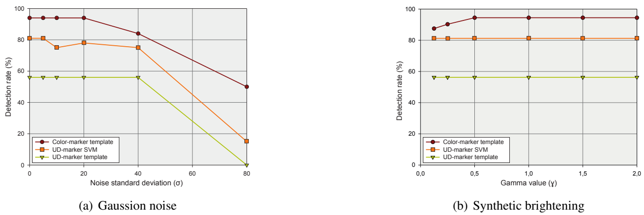
Figure 20. Evaluation of the robustness of the detection algorithm under varying (a) random Gaussian noise with standard deviation \sigma = 5; 10; 20; 40; 80 and (b) illumination conditions with \gamma = 0.125; 0.25; 0.5; 1.5; 2 .
