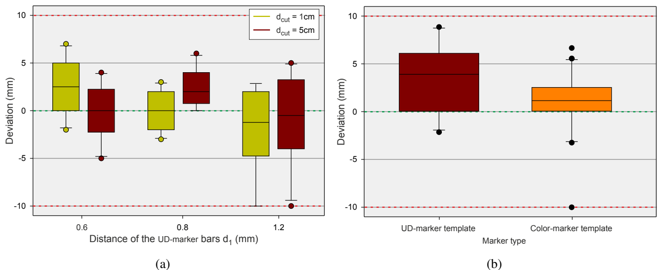
Figure 23. Accuracy of the detection process with UD-Marker_SVM on (a) transparent pouches. Varied parameters are the distance of the user-defined marker bars d_1 \in \{0.6\text{ mm}, 0.8\text{ mm}, 1.2\text{ mm}\} and the distance of the marker to the optimal cutting line d_{cut} \in \{1\text{ cm}, 5\text{ cm}\} . Visualization of the accuracy of the detection process of the template approaches (b): UD-Marker_Template on transparent pouches with user-defined marker and Color-Marker_Template on colored pouches. The y-axis in each box-whisker-plot indicates the deviation of the detected to the optimal cutting line.
