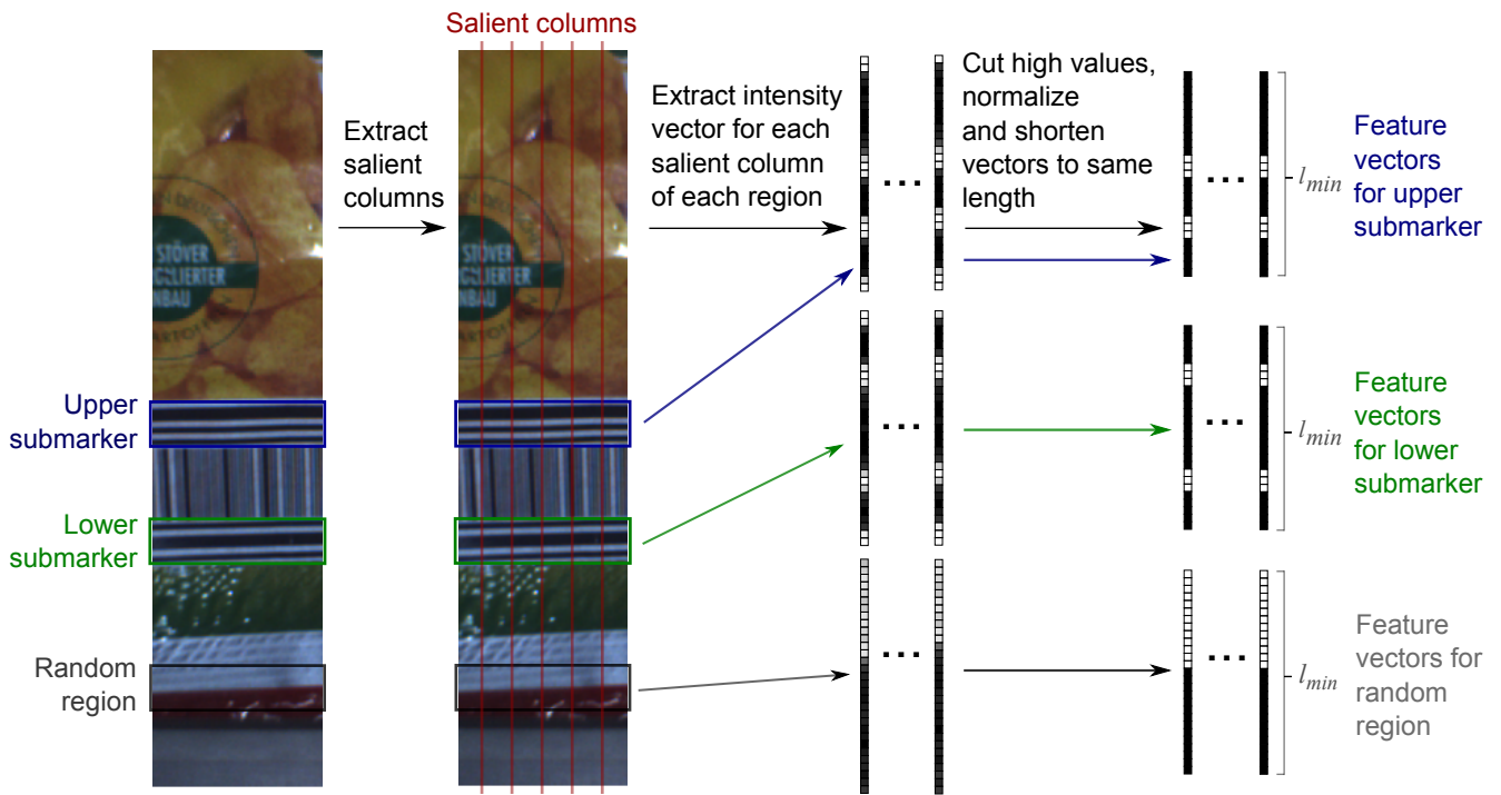
Figure 15. Schematic visualization of the learning classification model: extraction of feature vectors \mathbf{x}_i \in \mathbb{R}^{l_{min}} for the learning set of the SVM.
