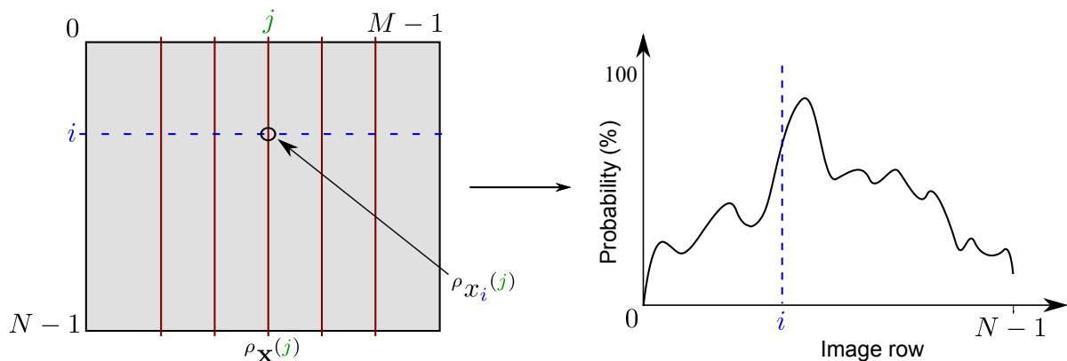
Figure 7. Schematic concept of the (Left) extraction of k \leq M salient columns \rho_{\mathbf{X}}(j) = \{\rho_{x_0}^{(j)}, \dots, \rho_{x_i}^{(j)}, \dots, \rho_{x_{N-1}}^{(j)}\} from an image of size N \times M pixels—the RGB-channel is represented by \rho \in \{r, g, b\} . The salient columns undergo a classification process leading to a time series which assigns the image rows a specific probability of containing the marker (Right).
