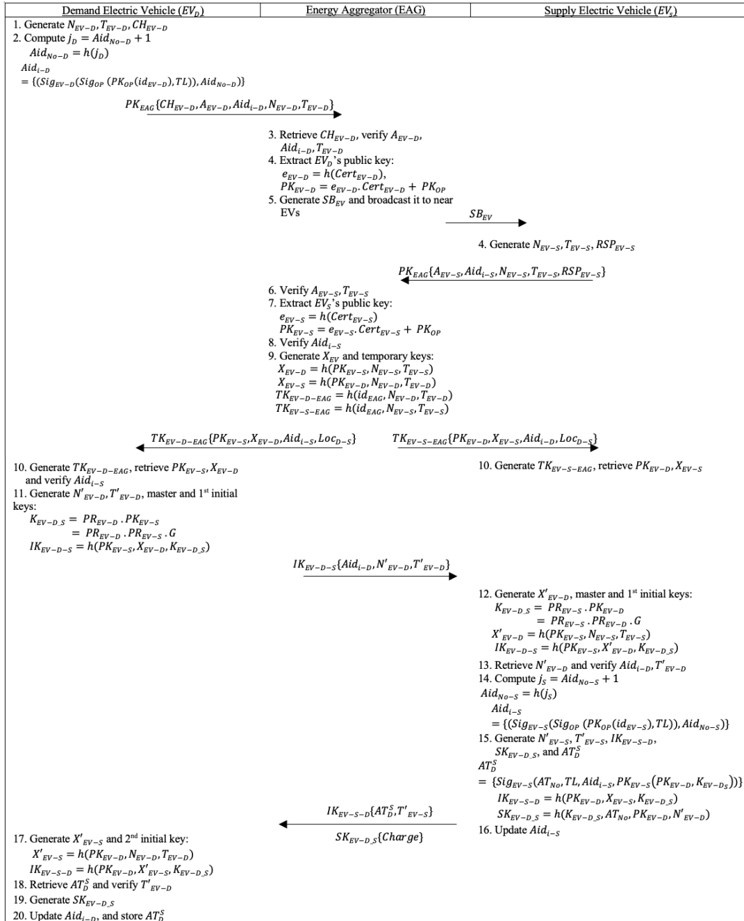
Figure 4. Proposed V2V mutual-authentication protocol.
