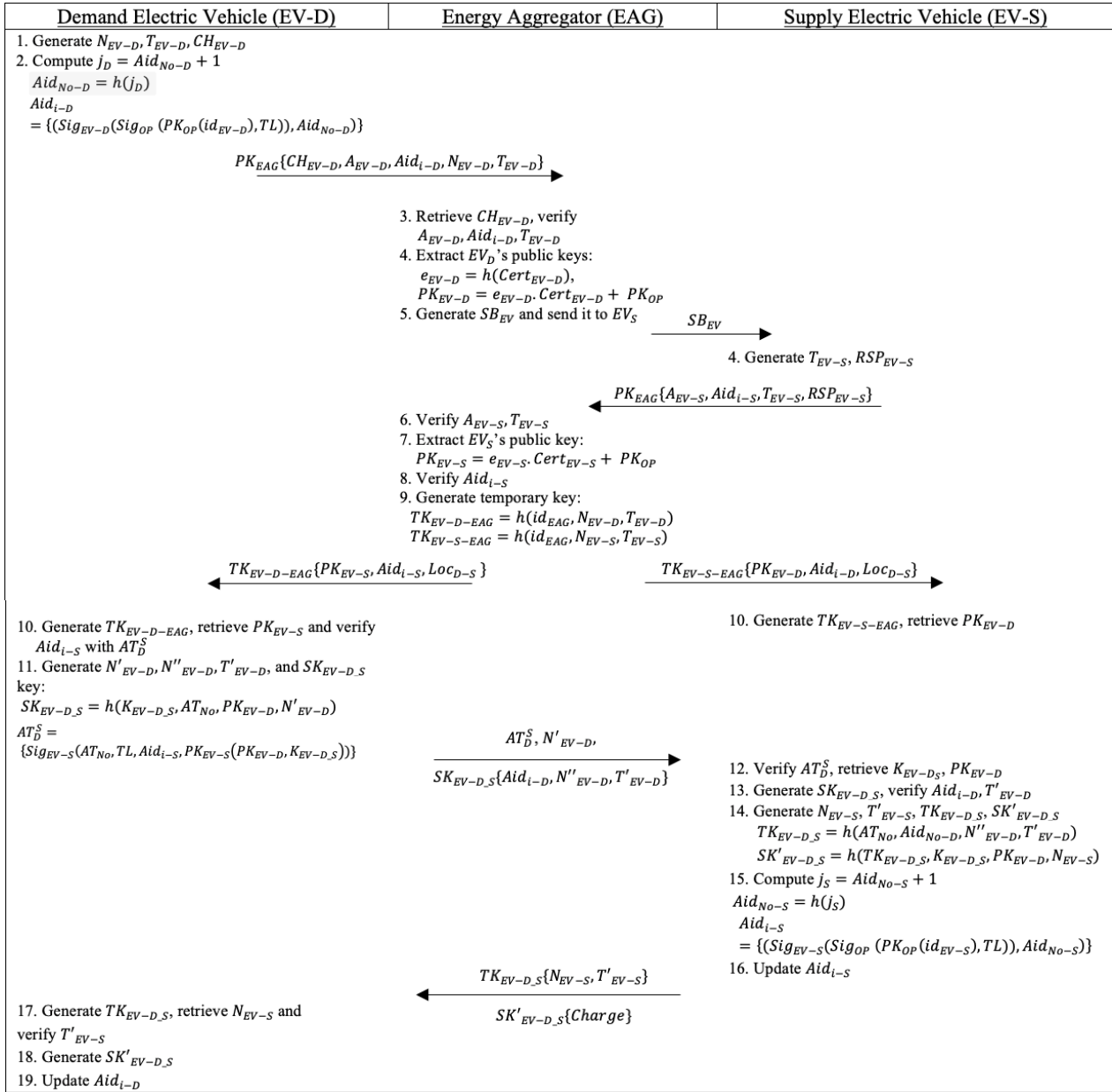
Figure 5. Proposed V2V mutual-re-authentication protocol.
