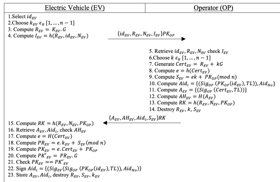
Figure 2. Proposed EV-registration phase.
