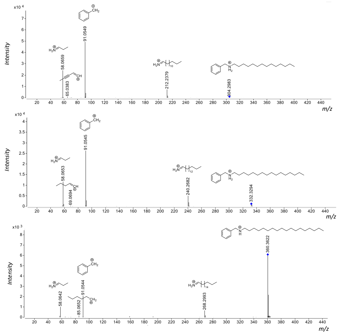
Figure 1: Experimental MS/MS spectra for the aryl alkylamines detected in the extract at the collision energy (30 eV) in positive.
