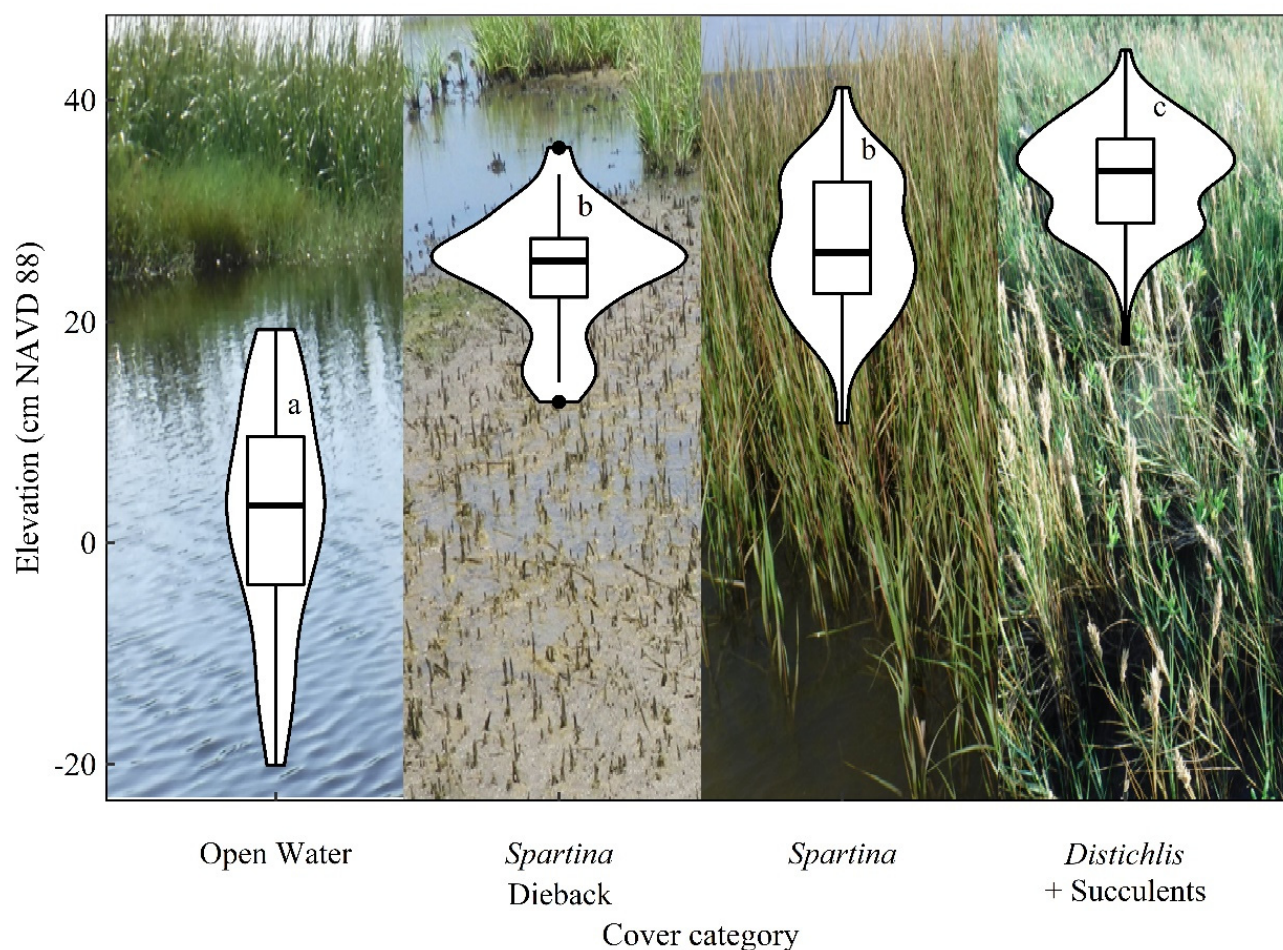
Figure 2. Box plots of the elevation for each cover category. Lower and upper box boundaries represent the 25th and 75th percentile, respectively, whereas the lines inside the boxes represent the median. The lower and upper error bars represent the 10th and 90th percentile, respectively. The outer ‘violin’ shapes show the probability density of the elevation values in each cover category. Groups with the same letter are not significantly different ( p > 0.05 ). Elevation data are rectified to the North American Vertical Datum of 1988 (NAVD88).
