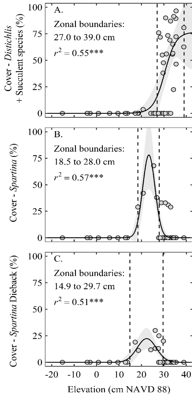
Figure 3. The relationship between elevation and the cover of (A). Distichlis + Succulents ( Distichlis spicata , Batis maritima , Lycium carolinianum , Monanthochloe littoralis , Borrichia frutescens , and Salicornia depressa ), (B). Spartina , and (C). Spartina Dieback. The dashed lines represent the elevation zonal boundaries and the gray shaded areas represent the 95% confidence intervals of the regressions. *** indicates p < 0.001 . Elevation data are rectified to the North American Vertical Datum of 1988 (NAVD88).
