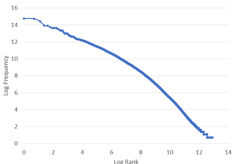
Figure 4. Zipf curves for the Indonesian corpus (650 K).
