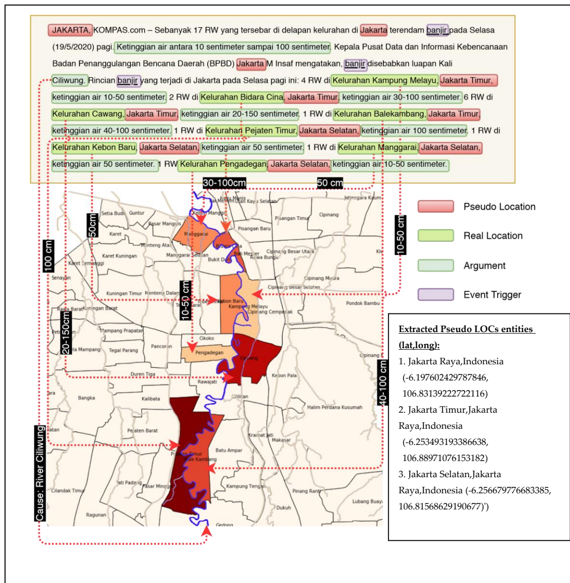
Figure 13. Visualization sample from a single article with result from our proposed Event Geoparser. The source article is displayed and tagged with colors, indicating arguments, event trigger, and pseudo-location/real-location label for every detected toponym.
