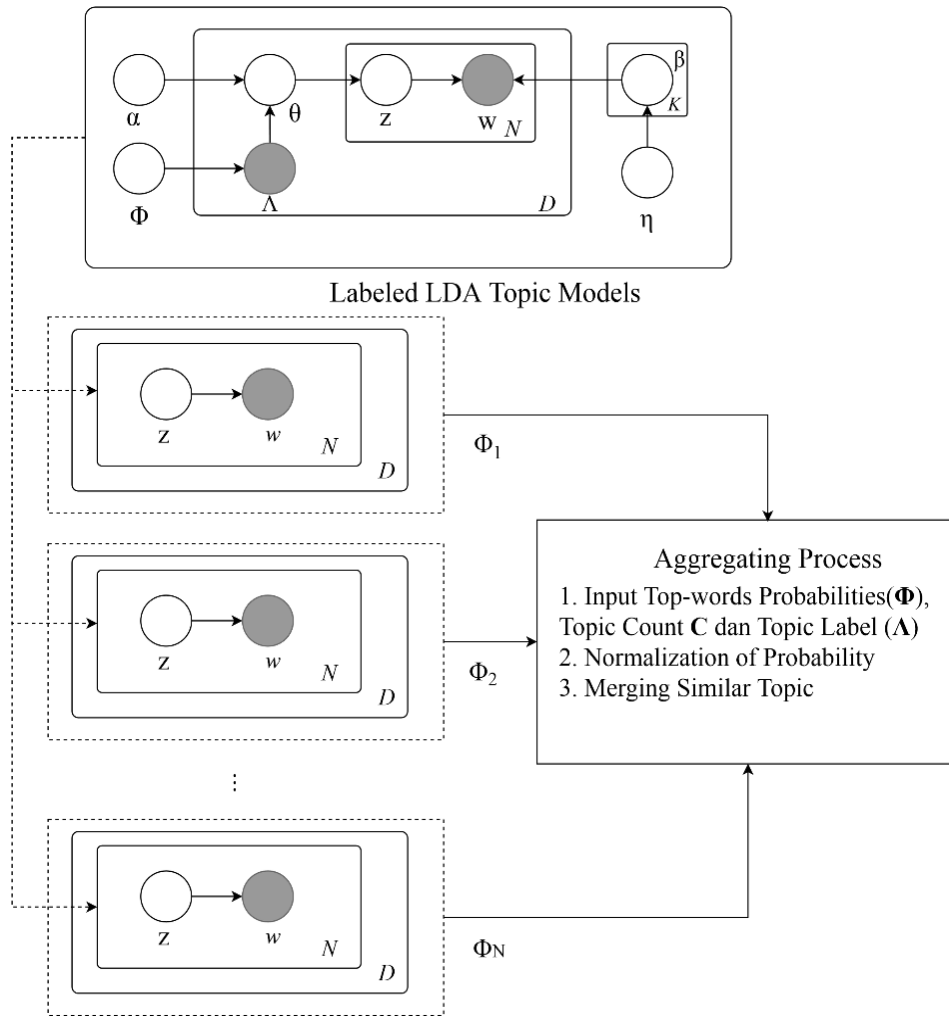
Figure 6. Aggregated topic model plate notation and schema.
