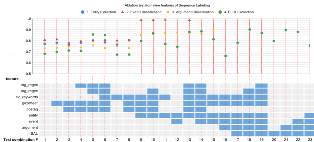
Figure 10. Ablation Test of weighted F1 score from nine combinations of features of four geotagging steps (step 1, 3, 4, and 5 from Figure 4). Active features are marked as blue cells (below part of the graphic). Missing score points means such combination of features is not applicable on that particular step.
