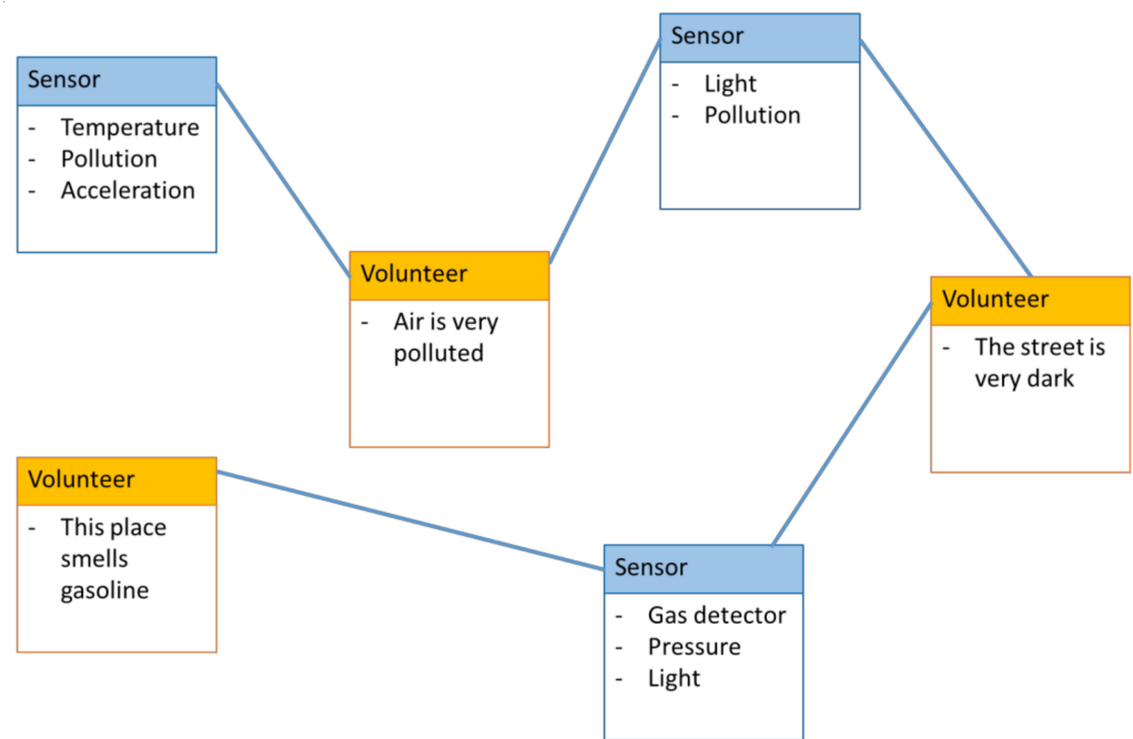
Figure 4. Relationships of sensor and volunteers based on observed property.
