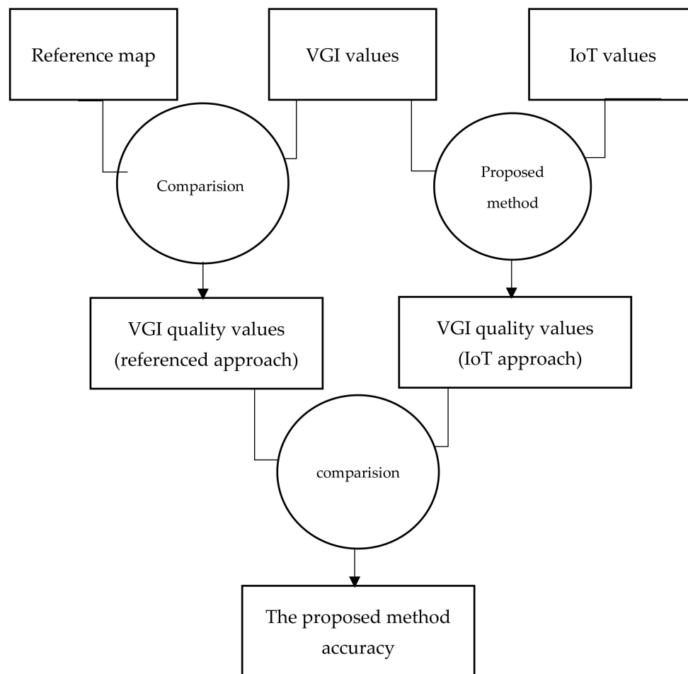
Figure 8. Evaluation flowchart.
