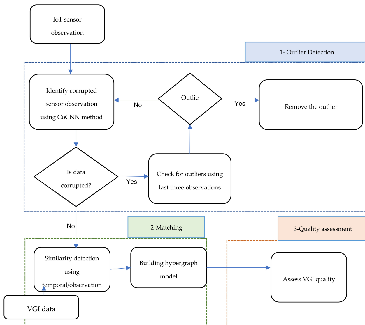
Figure 1. The proposed quality assessment method.
