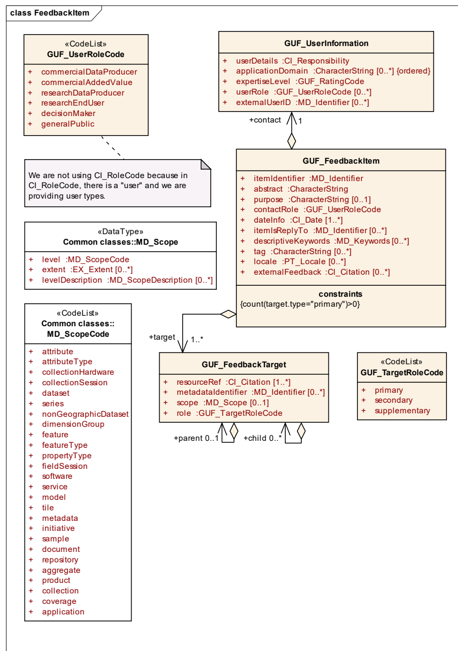
Figure 1. UML class diagram describing the GUF_FeedbackItem in relation to GUF_FeedbackTarget and GUF_UserInformation, as described in the official pen Geospatial Consortium (OGC) Geospatial User Feedback (GUF) standard (adapted from UML diagrams used in [16]). Orange boxes represent GUF classes, while white boxes come from ISO 19115.
