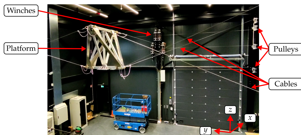
Figure 1. IPAnema Safe ( https://youtu.be/vFaTntglG5g , accessed on 24 June 2026) installed at MARIN in Wageningen, The Netherlands.
