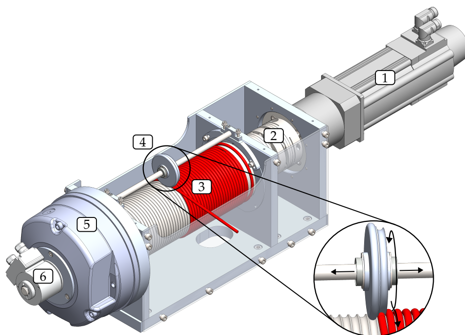
Figure 6. Final IPAnema Safe winch design.
