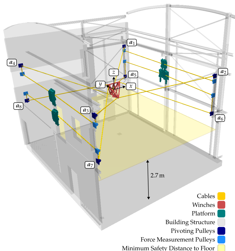
Figure 3. Visualization of the IPAnema Safe layout.
