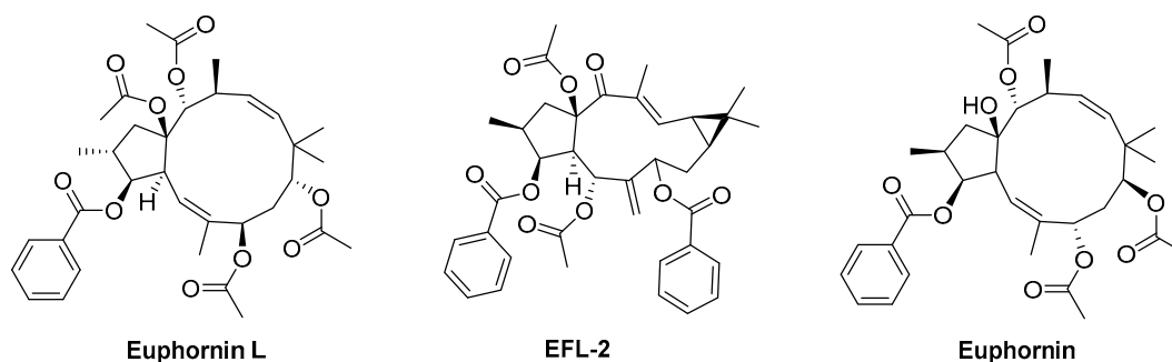
Figure 3. Chemical structures of some in vivo bioactive Euphorbia compounds.
