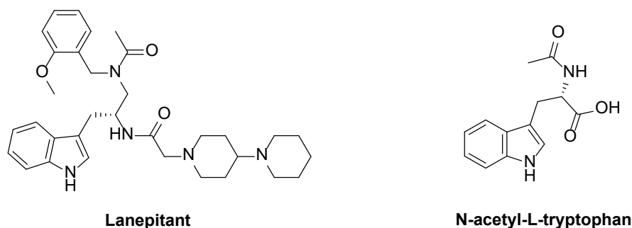
Figure 16. Neurokinin receptor ligands.
