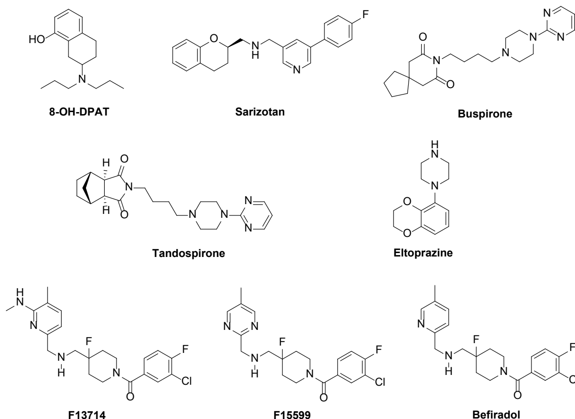
Figure 3. 5-HT 1A R agonists.
