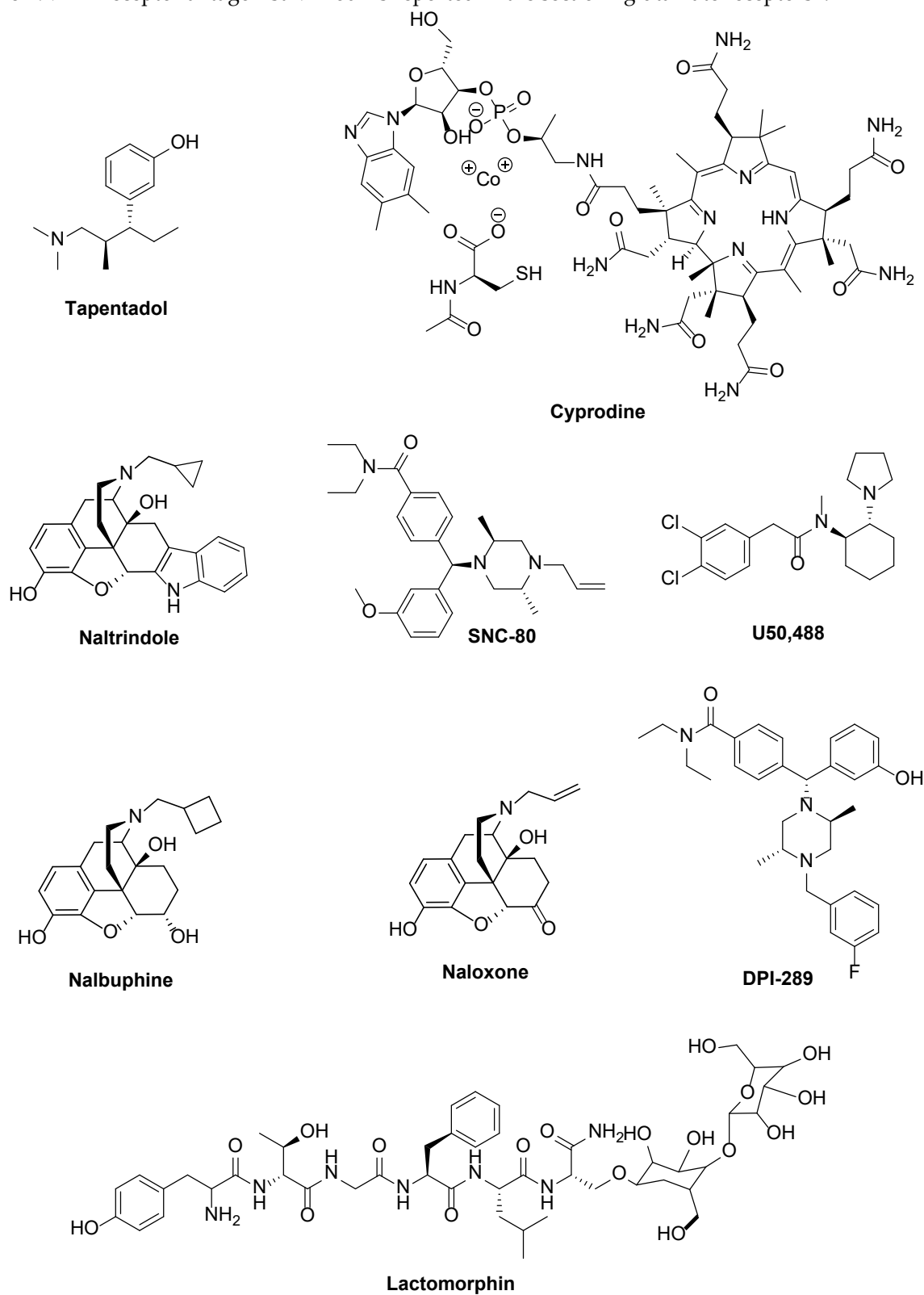
Figure 17. Opioid receptor ligands.
