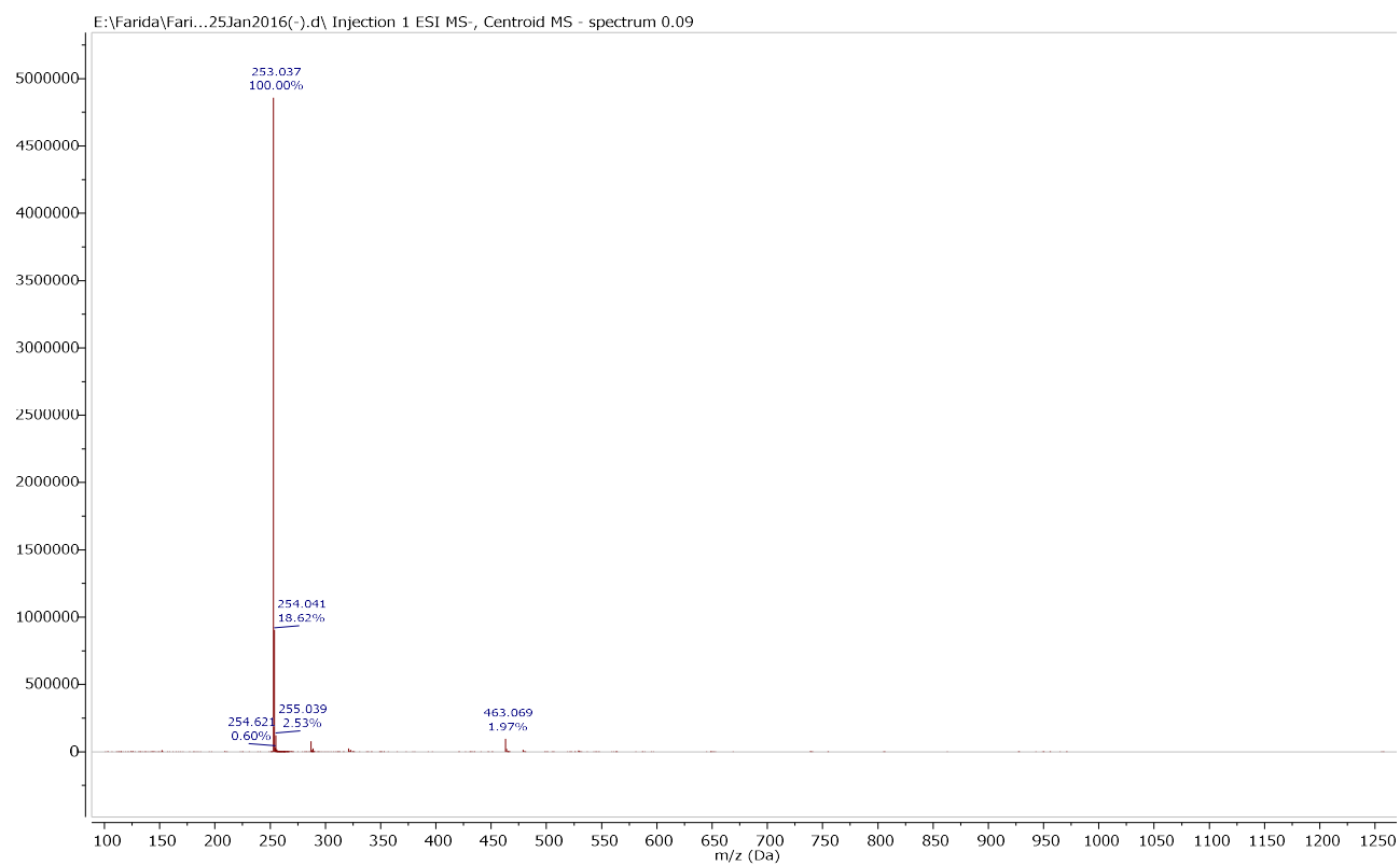
Figure S6: Negative HRESIMS for compound 2
