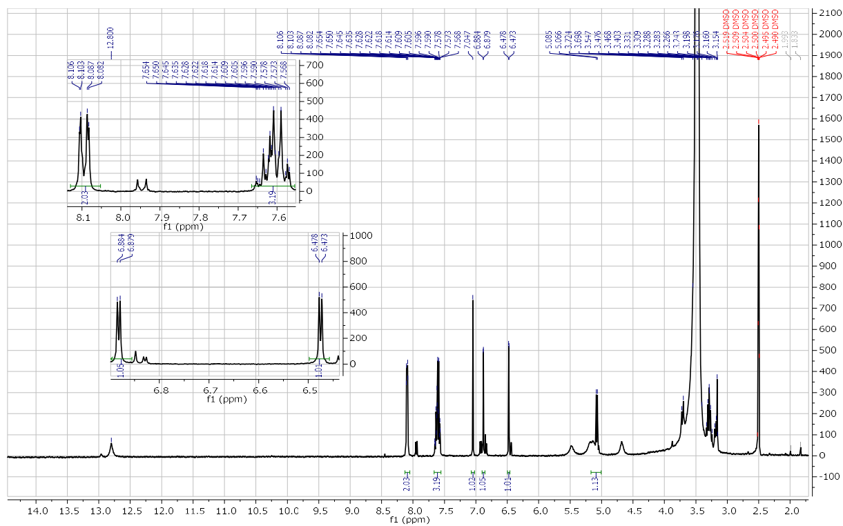
Figure S7: ^1\text{H} NMR spectrum of compound 3
