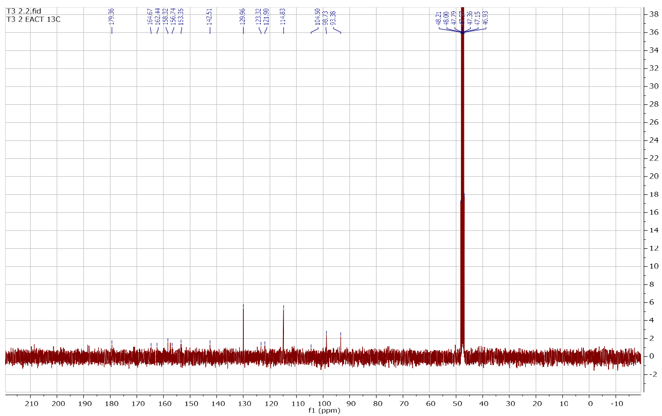
Figure S2: ^{13}\text{C} NMR spectrum of compound 1
