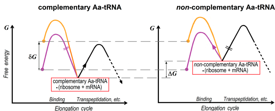
Figure 5. Scheme of the total free energy change in formation and further transformation of the Aa-tRNA•(ribosome•mRNA) complex for the complementary and non-complementary Aa-tRNAs. Purple line: factor-free binding; orange line: EF-Tu•GTP-promoted binding. \Delta G ( \gg k_B T ): the free energy difference between the binding of non-complementary and complementary Aa-tRNA to the ribosome•mRNA complex. \delta G ( \gg k_B T ): the free energy difference between the factor-free and Tu factor-promoted binding of Aa-tRNA to the ribosome•mRNA complex, i.e., the free energy outcome of the exergonic reaction of GTP hydrolysis, \text{EF-Tu}\cdot\text{GTP} \rightarrow \text{EF-Tu}\cdot\text{GDP} + \text{P}_i . The time of a reaction is exponentially dependent on the barrier height. The main, i.e., the fastest (overcoming the lower free energy barrier) pathway of transformation of the Aa-tRNA•(ribosome•mRNA) complex is shown by an arrow, and the slower pathway is crossed out.
