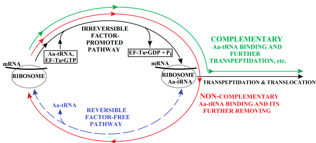
Figure 6. Proofreading: Rejection of the amino acid brought by the non-complementary Aa-tRNA (red solid arrow), but incorporation into the growing polypeptide chain of the amino acid brought by the Aa-tRNA complementary to the ribosome-exhibited mRNA codon (green solid arrow). The center of the scheme shows two parallel pathways for penetration into the ribosome of the “new” amino acid brought by the Aa-tRNA. The irreversible factor-promoted pathway (black one-way arrow) is supported, while the reversible factor-free pathway (blue dashed two-way arrow) is not supported by the free energy of GTP hydrolysis performed using the elongation factor Tu.
