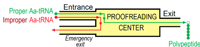
Figure 1. A scheme of proofreading.
