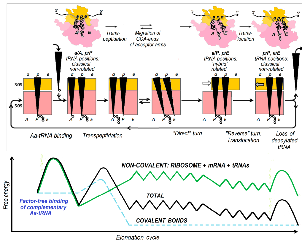
Figure 4. Top panel: the entire elongation cycle of the translating ribosome for the “factor-free” process. All the shown events, except for transpeptidation, require significant movements of the ribosome parts and/or mRNA and tRNAs. The ribosome is in the open (unlocked) state when it turns, when the deacylated tRNA is leaving, and when the Aa-tRNA is binding—in other states, it is in the closed (locked) state [2,18,19]. Bottom panel: generalized plots showing the free energy change during one “factor-free” elongation cycle (for the case when the anticodon of Aa-tRNA is complementary to the exposed mRNA codon) [17]: the covalent bond energy (blue dashed line), non-covalent interactions within the (ribosome•mRNA)•tRNAs complex (green line), and the sum of these two free energies (black line). The first large free energy barrier corresponds to the transition state at the stage of Aa-tRNA binding, and the last, to that at the stage of tRNA unbinding, and the central one to the activation barrier at the stage of transpeptidation (chemical reaction that is an energy source for the entire factor-free elongation cycle). The growth of free energy of the non-covalent interactions within the (ribosome•mRNA)•tRNAs complex occurring at the latter stage is due to poor binding of the acceptor arms of the newly formed peptidyl-tRNA to the A site and the deacylated tRNA to the P site. The small bumps on the free energy profile at the stages of forward and reverse turns symbolize free-energy barriers for the diffusion motion of the 30S subunit relative to the 50S one. Adapted from [17] with some modifications.
