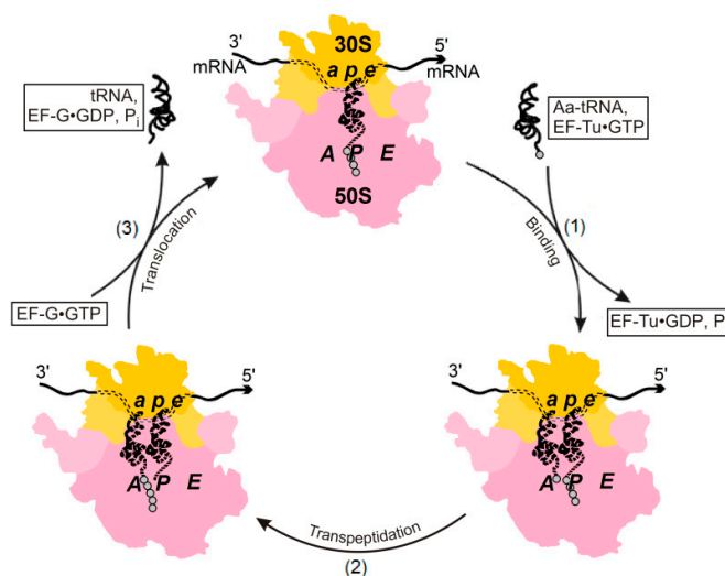
Figure 2. Factor-depending working cycle of the ribosome in vivo. The small (30S in prokaryotes) ribosomal subunit is shown in yellow—it is bound to the mRNA and contains the decoding center (DC) which consists of the a , p , and e sites that have to bind the anticodon arms of tRNAs, thus forming the (tRNA anticodon)-(mRNA codon) duplexes at different stages of the working cycle. The large (50S in prokaryotes) ribosomal subunit is shown in pink—it contains the peptidyl transferase center (PTC), which consists of the A , P , and E sites that have to bind the acceptor arms of tRNAs at different stages of the working cycle. Small gray circles bound to tRNAs denote amino acid residues. Each of the three shown stages is irreversible, because they include an exergonic chemical reaction: at stage (2), transpeptidation, and at stages (1) and (3), the auxiliary elongation factors EF-Tu and EF-G cleave the GTP molecules. Adapted from [2,16,17] with minor modifications.
