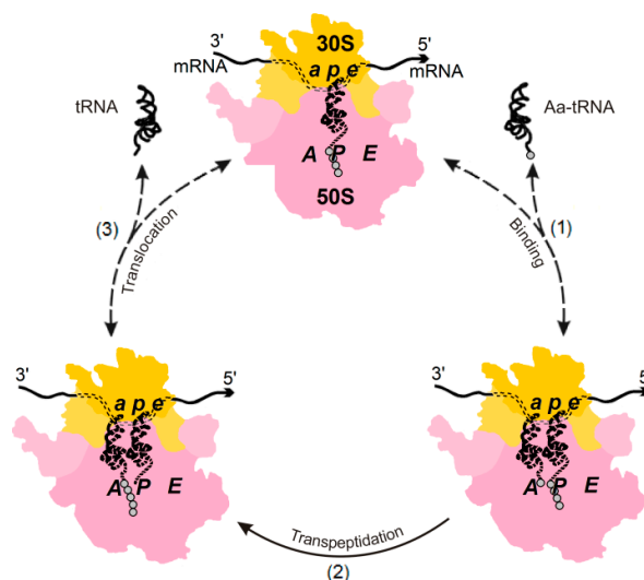
Figure 3. The elongation cycle of the translating ribosome in the simplest “factor-free” in vitro process. The only difference between Figures 3 and 2 is the absence (in Figure 3) of the elongation factors EF-Tu and EF-G together with the GTP molecules. Because of that, stages (1) and (3), which now do not include exergonic chemical reactions, can be reversible (which is shown by dashed two-way arrows), while stage (2), transpeptidation, remains irreversible. Adapted from [2,16,17] with minor modifications.
